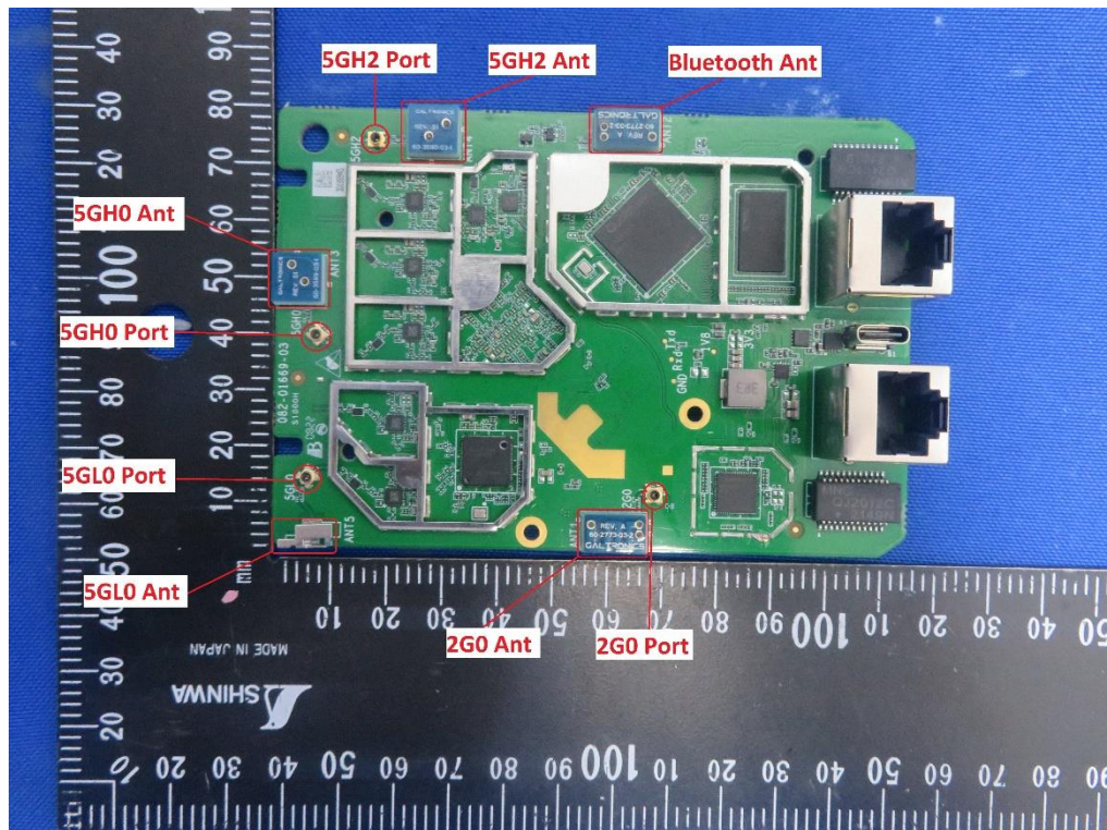
(23) EUT Photo
