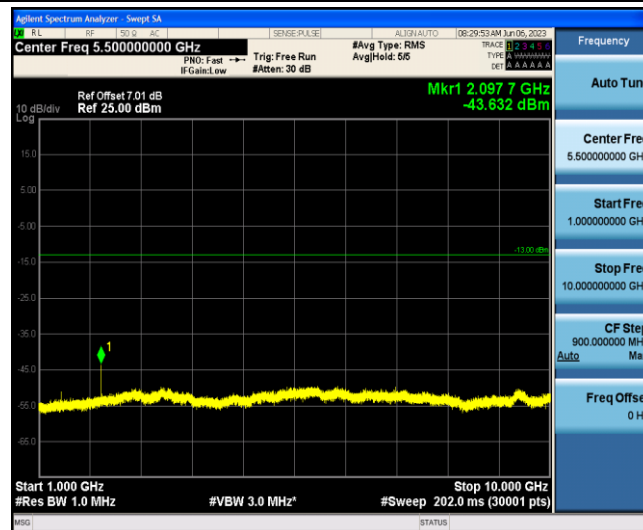
Band12-1.4MHz-QPSK-23017-1-0-Low-1000-10000--43.63-PASS
