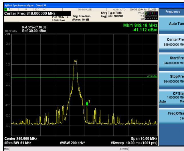
Band5-1.4MHz-16QAM-20643-1-5-High--41.11-PASS
