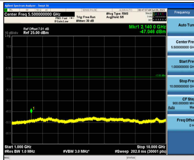
Band12-3MHz-16QAM-23165-1-0-Low-1000-10000--47.05-PASS
