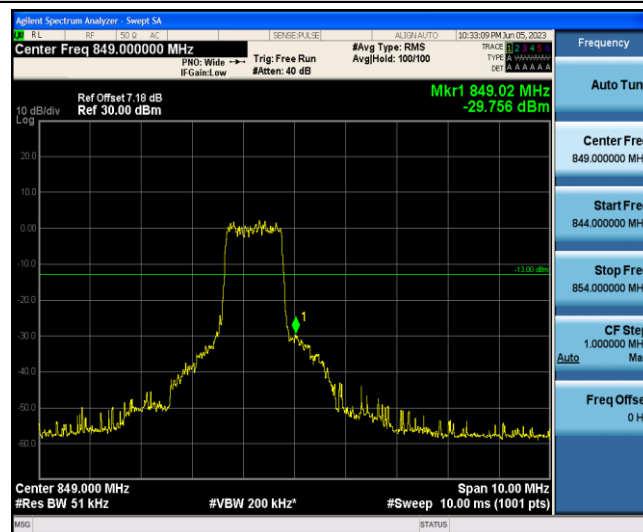
Band5-5MHz-QPSK-20625-6-0-High--29.76-PASS
