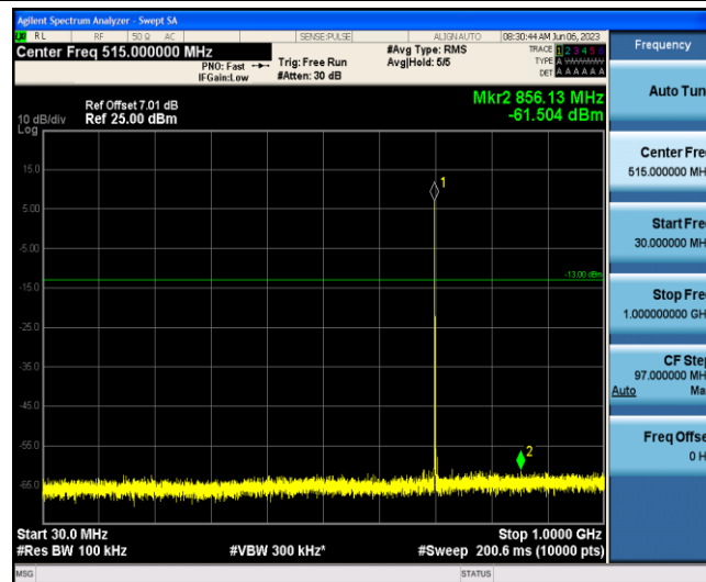
Band12-1.4MHz-16QAM-23095-1-0-Low-30-1000--61.5-PASS
