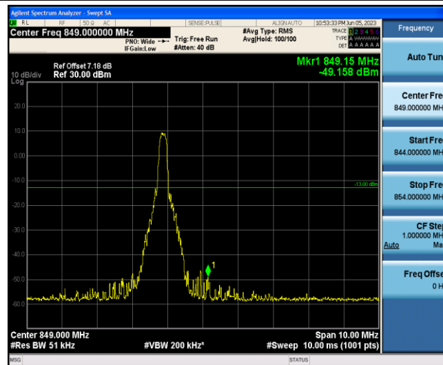
Band5-10MHz-16QAM-20600-1-5-High--49.16-PASS
