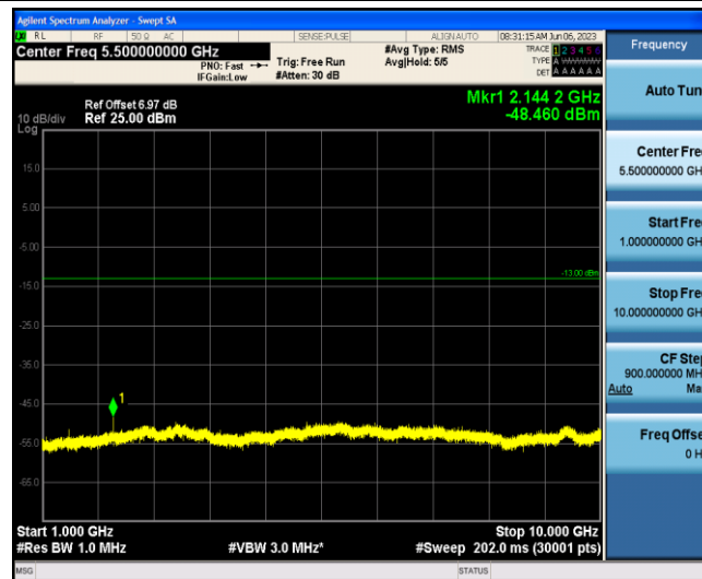
Band12-1.4MHz-QPSK-23173-1-0-Low-1000-10000--48.46-PASS
