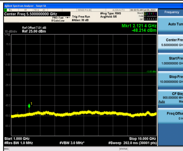
Band12-1.4MHz-16QAM-23095-1-0-Low-1000-10000--48.21-PASS
