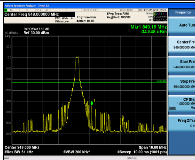
Band5-3MHz-16QAM-20635-1-5-High--34.55-PASS
