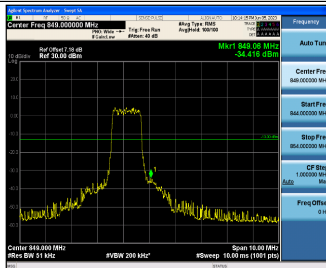
Band5-3MHz-QPSK-20635-6-0-High--34.42-PASS
