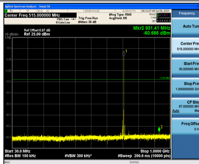
Band12-1.4MHz-QPSK-23173-1-0-Low-30-1000--60.67-PASS
