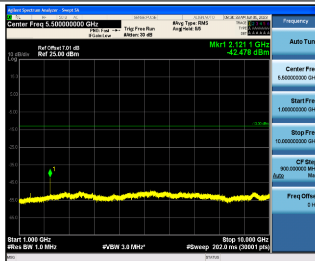
Band12-1.4MHz-QPSK-23095-1-0-Low-1000-10000--42.48-PASS
