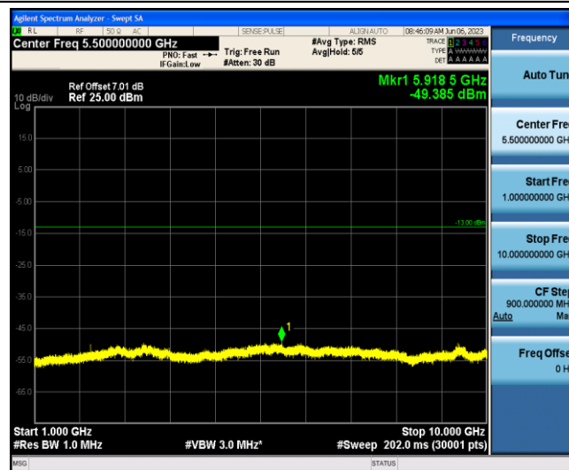
Band12-3MHz-QPSK-23095-1-0-Low-1000-10000--49.39-PASS
