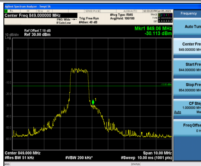
Band5-5MHz-16QAM-20625-6-0-High--30.11-PASS
