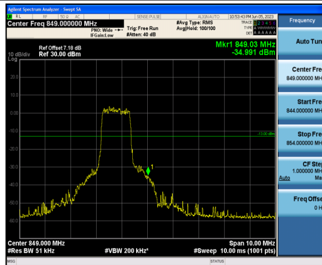
Band5-10MHz-QPSK-20600-6-0-High--34.99-PASS
