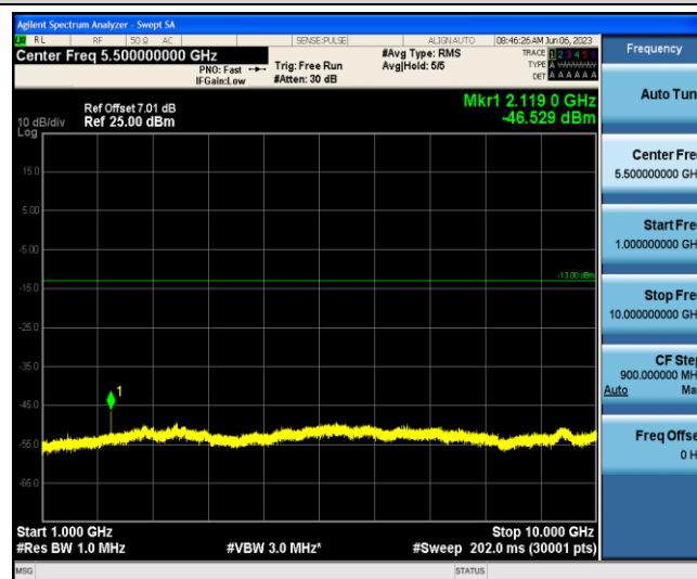
Band12-3MHz-16QAM-23095-1-0-Low-1000-10000--46.53-PASS
