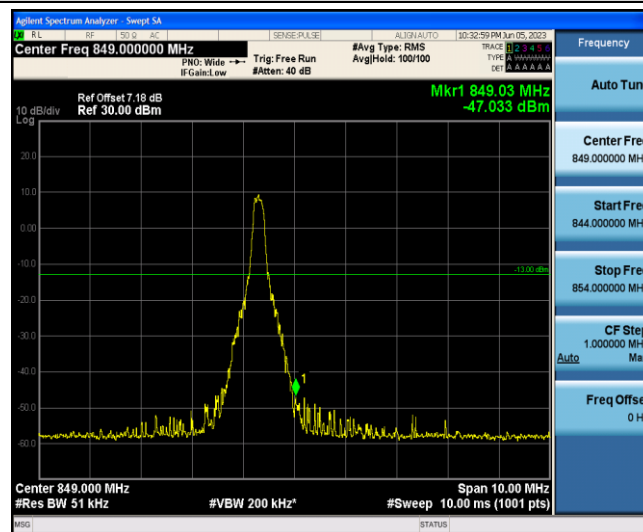
Band5-5MHz-16QAM-20625-1-5-High--47.03-PASS
