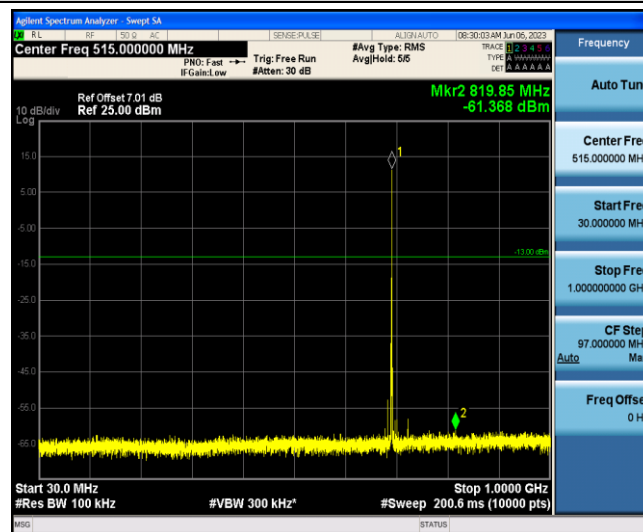
Band12-1.4MHz-16QAM-23017-1-0-Low-30-1000--61.37-PASS
