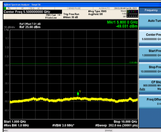
Band12-5MHz-QPSK-23035-1-0-Low-1000-10000--49.03-PASS
