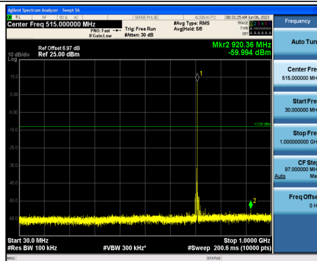
Band12-1.4MHz-16QAM-23173-1-0-Low-30-1000--59.99-PASS
