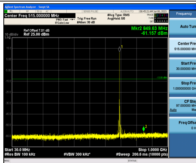
Band12-3MHz-QPSK-23025-1-0-Low-30-1000--61.16-PASS
