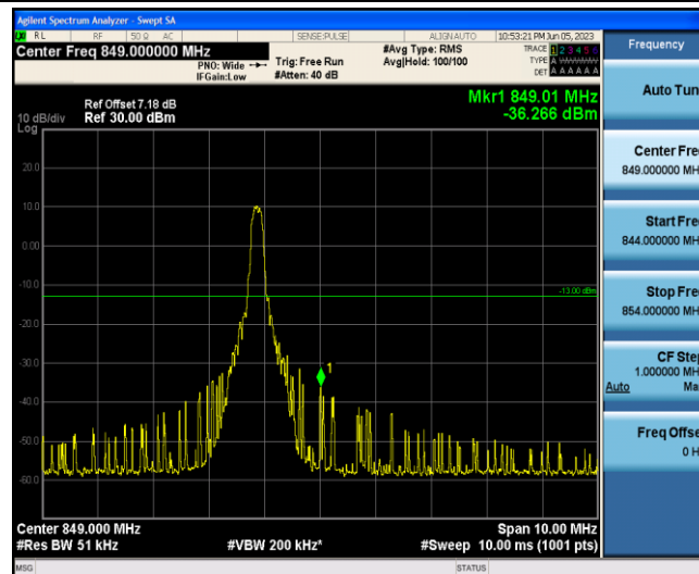
Band5-10MHz-QPSK-20600-1-5-High--36.27-PASS
