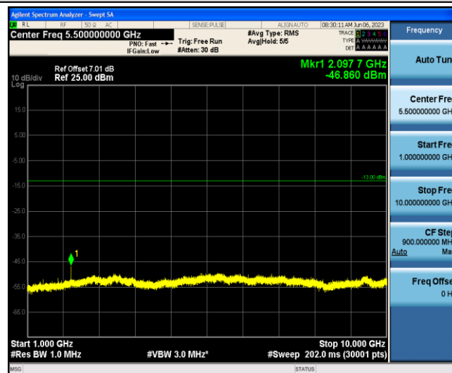
Band12-1.4MHz-16QAM-23017-1-0-Low-1000-10000--46.86-PASS
