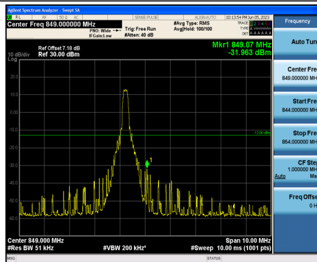
Band5-3MHz-QPSK-20635-1-5-High--31.96-PASS
