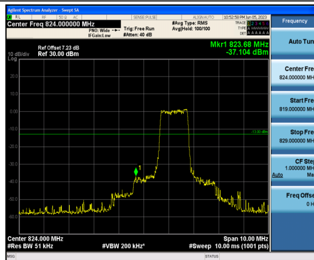
Band5-10MHz-QPSK-20450-6-0-Low--37.10-PASS
