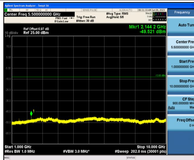
Band12-1.4MHz-16QAM-23173-1-0-Low-1000-10000--49.52-PASS
