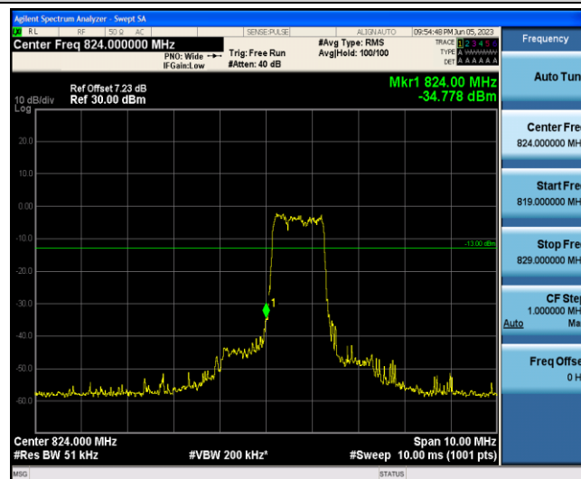
Band5-1.4MHz-16QAM-20407-6-0-Low--34.78-PASS
