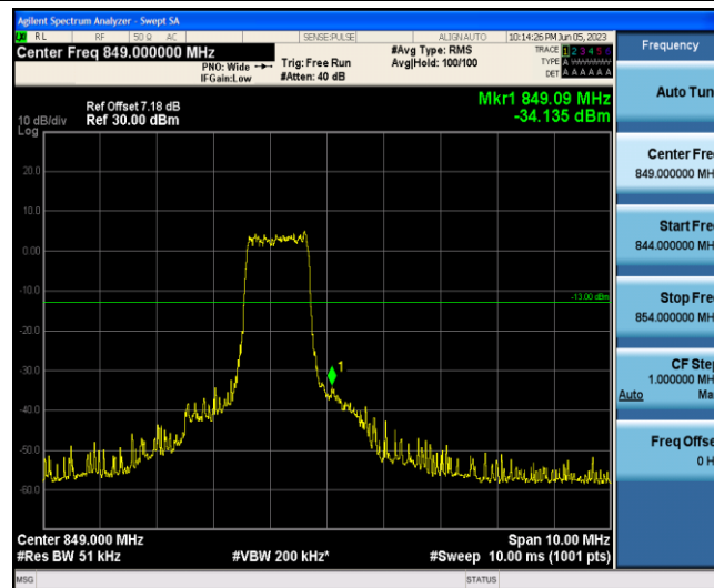
Band5-3MHz-16QAM-20635-6-0-High--34.14-PASS
