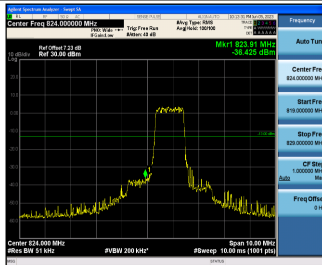
Band5-3MHz-QPSK-20415-6-0-Low--36.42-PASS
