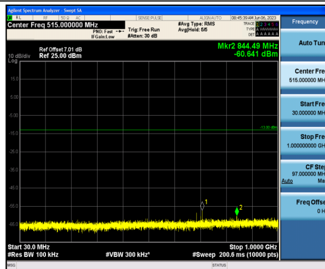
Band12-3MHz-16QAM-23025-1-0-Low-30-1000--60.64-PASS
