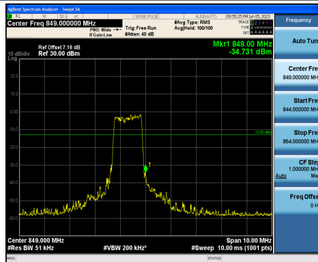
Band5-1.4MHz-QPSK-20643-6-0-High--34.73-PASS
