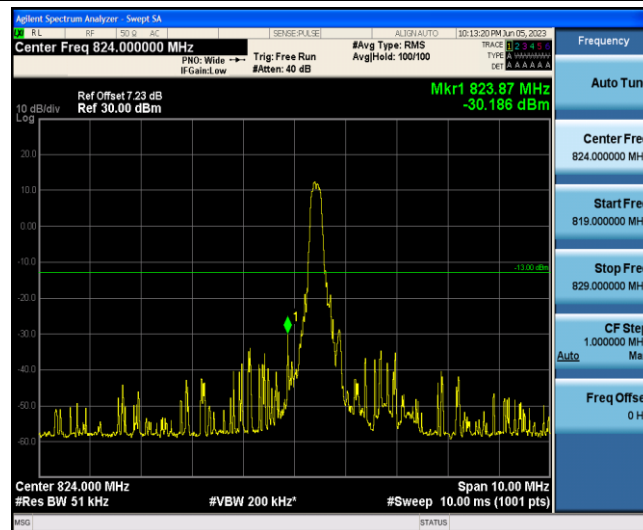
Band5-3MHz-16QAM-20415-1-0-Low--30.19-PASS
