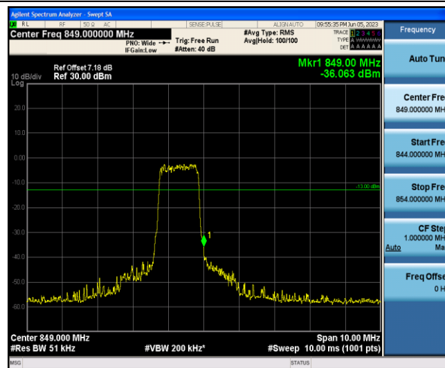
Band5-1.4MHz-16QAM-20643-6-0-High--36.06-PASS
