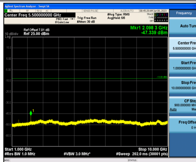
Band12-3MHz-QPSK-23025-1-0-Low-1000-10000--47.34-PASS
