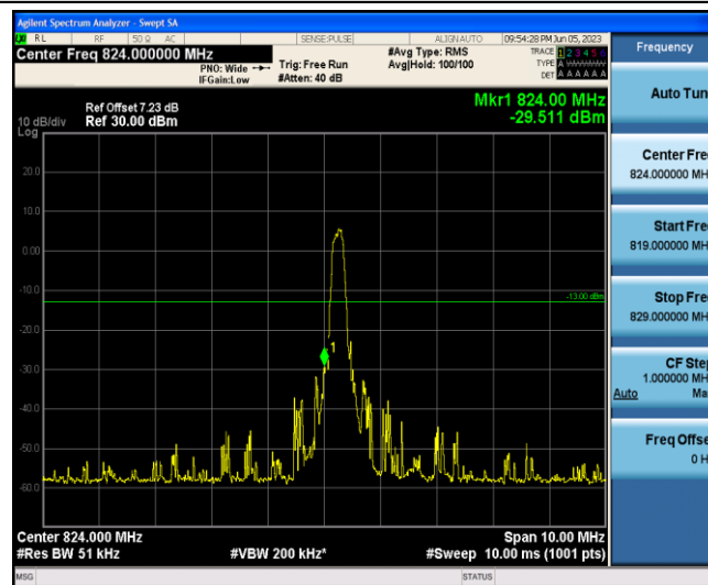
Band5-1.4MHz-16QAM-20407-1-0-Low--29.51-PASS
