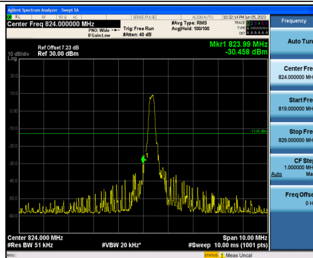
Band5-5MHz-16QAM-20425-1-0-Low--30.46-PASS
