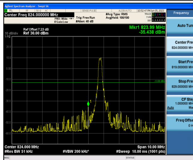
Band5-10MHz-16QAM-20450-1-0-Low--35.44-PASS
