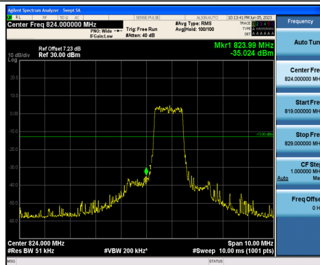
Band5-3MHz-16QAM-20415-6-0-Low--35.02-PASS
