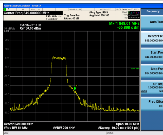
Band5-10MHz-16QAM-20600-6-0-High--35.87-PASS
