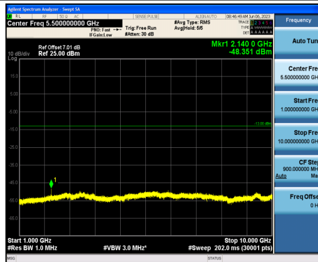
Band12-3MHz-QPSK-23165-1-0-Low-1000-10000--48.35-PASS
