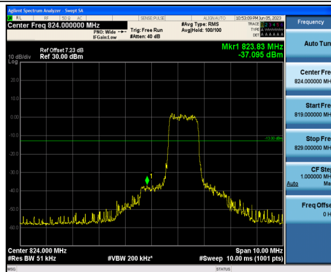
Band5-10MHz-16QAM-20450-6-0-Low--37.10-PASS
