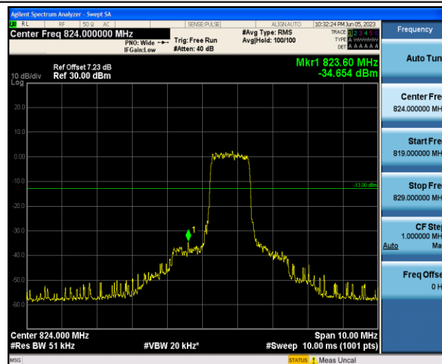
Band5-5MHz-QPSK-20425-6-0-Low--34.65-PASS
