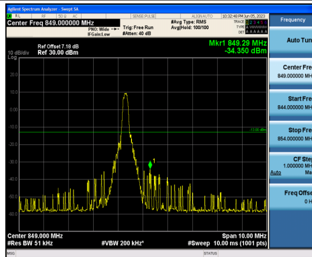
Band5-5MHz-QPSK-20625-1-5-High--34.35-PASS
