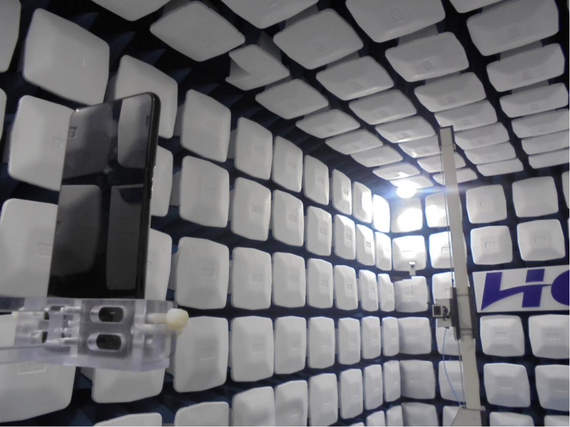
5. mmWave Test Setup Photo_18-40G
