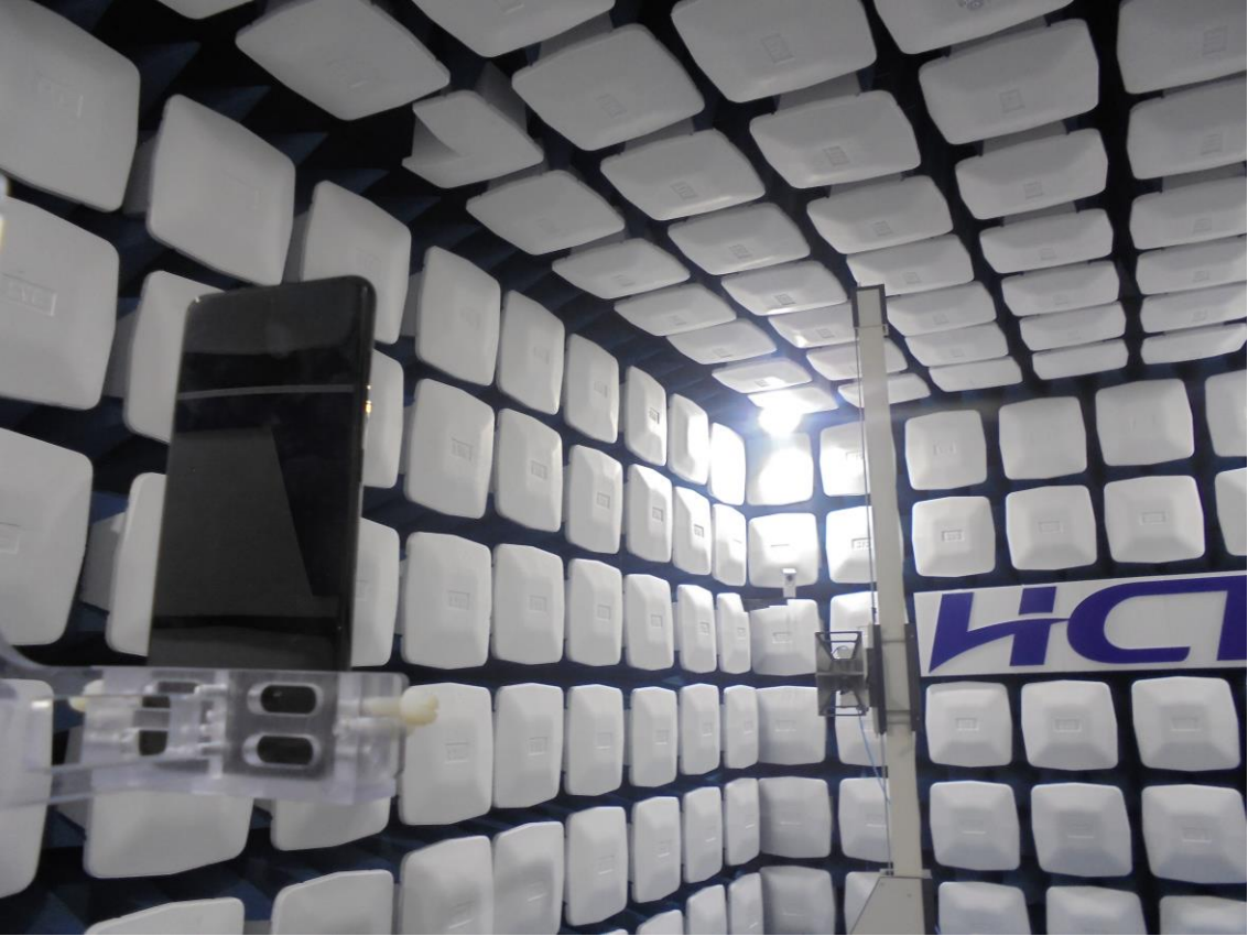
4. mmWave Test Setup Photo_1-18G
