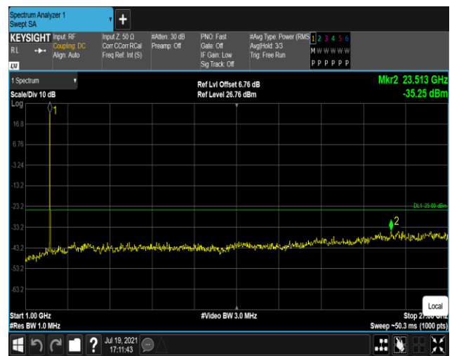
Band7-20MHz-16QAM-21100:1000~27000MHz
