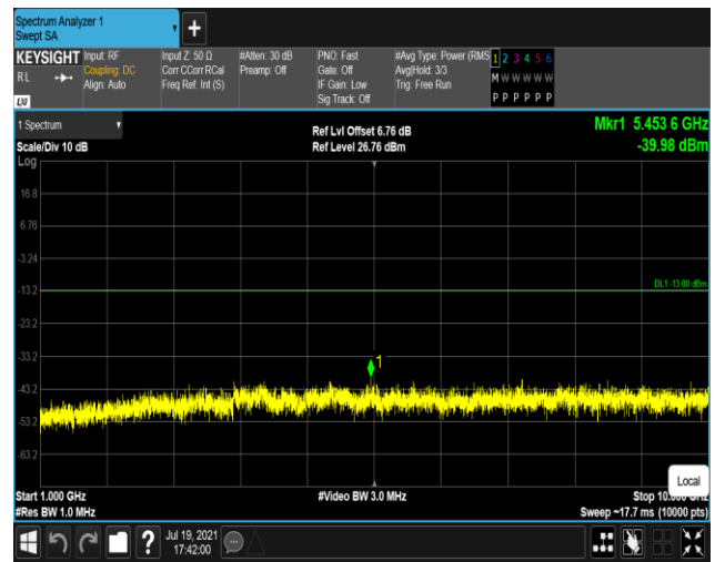
Band17-10MHz-QPSK-23790:1000~10000MHz
