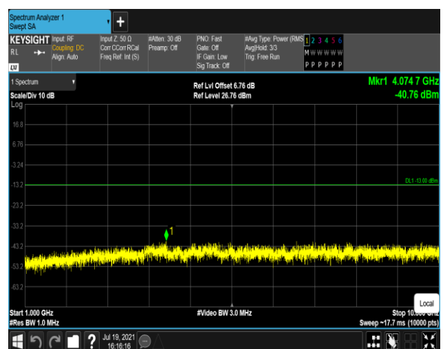
Band5-10MHz-QPSK-20600:1000~10000MHz
