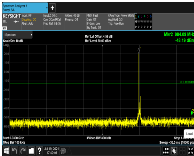
Band17-10MHz-QPSK-23800:30~1000MHz
