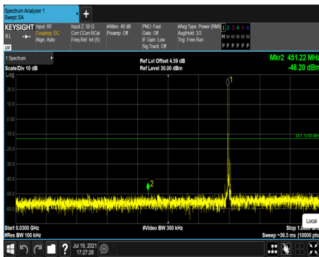
Band17-5MHz-16QAM-23790:30~1000MHz
