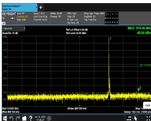
Band17-5MHz-16QAM-23825:30~1000MHz
