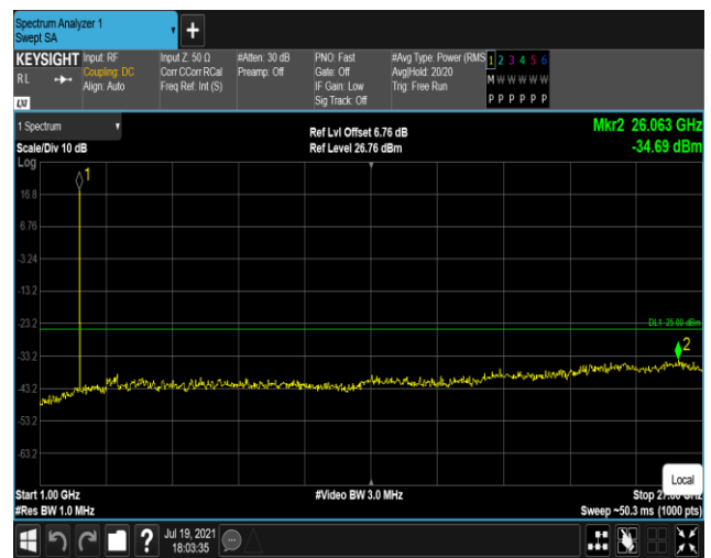
Band38-5MHz-16QAM-38000:1000~27000MHz
