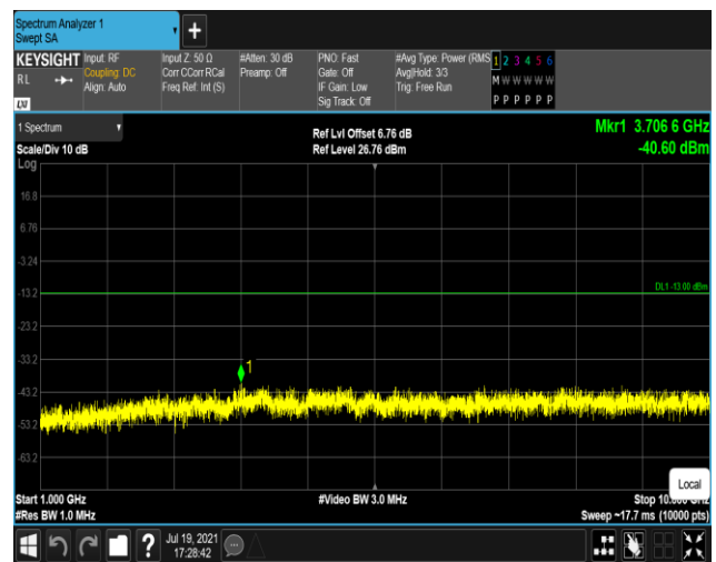
Band17-5MHz-16QAM-23825:1000~10000MHz
