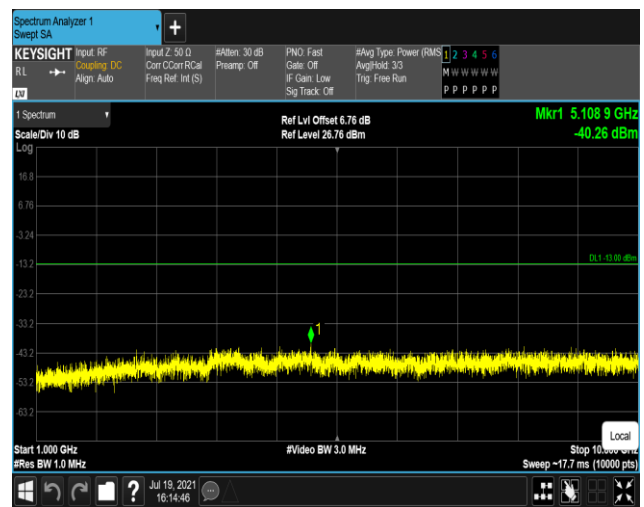
Band5-10MHz-16QAM-20525:1000~10000MHz
