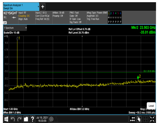
Band7-5MHz-QPSK-21100:1000~27000MHz
