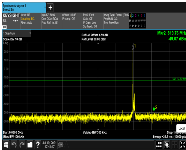
Band17-10MHz-QPSK-23790:30~1000MHz
