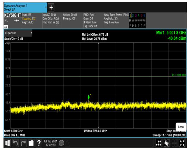
Band17-10MHz-QPSK-23800:1000~10000MHz
