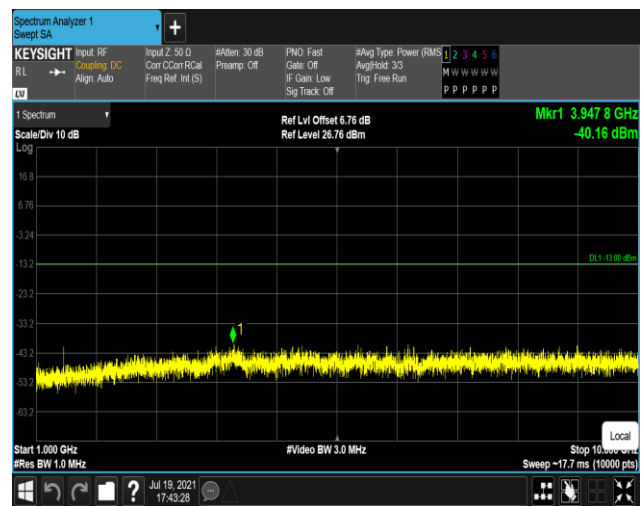
Band17-10MHz-16QAM-23800:1000~10000MHz
