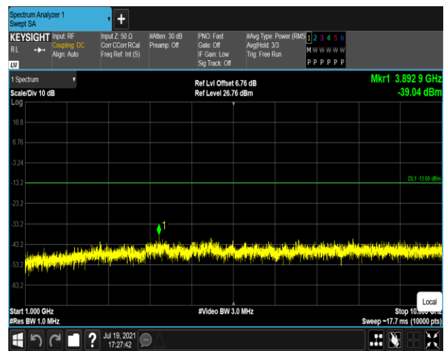
Band17-5MHz-16QAM-23790:1000~10000MHz
