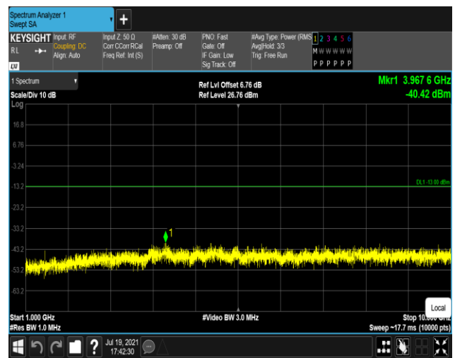
Band17-10MHz-16QAM-23790:1000~10000MHz
