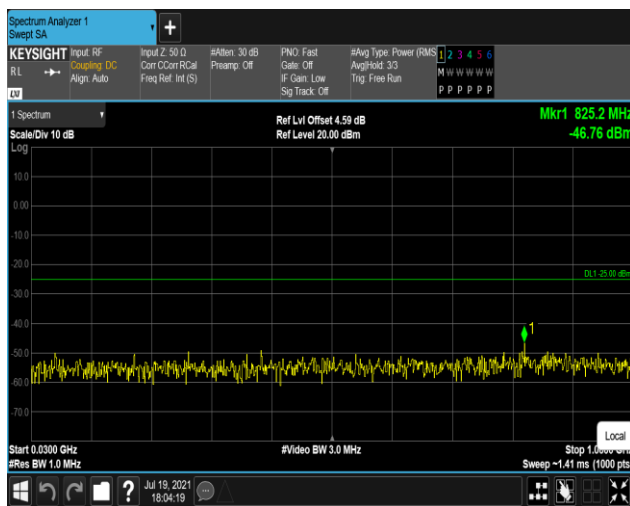
Band38-5MHz-16QAM-38225:30~1000MHz
