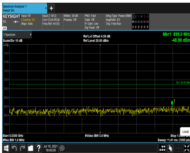
Band38-20MHz-QPSK-38000:30~1000MHz
