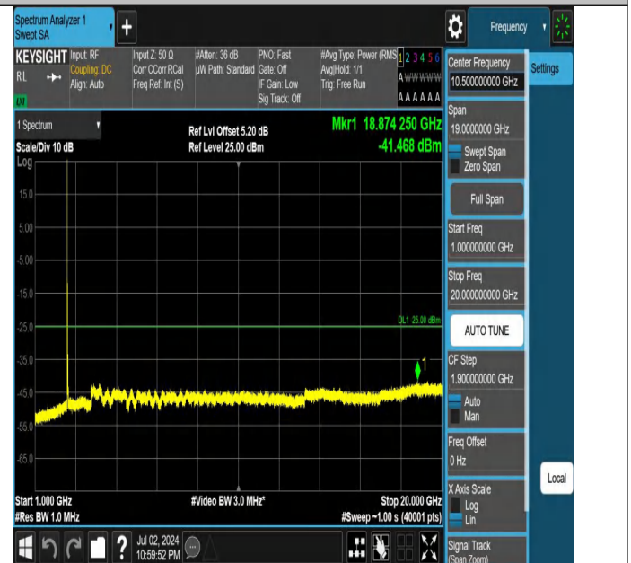
Band7-15MHz-QPSK-20825-1RB#0-1000~20000-PASS
