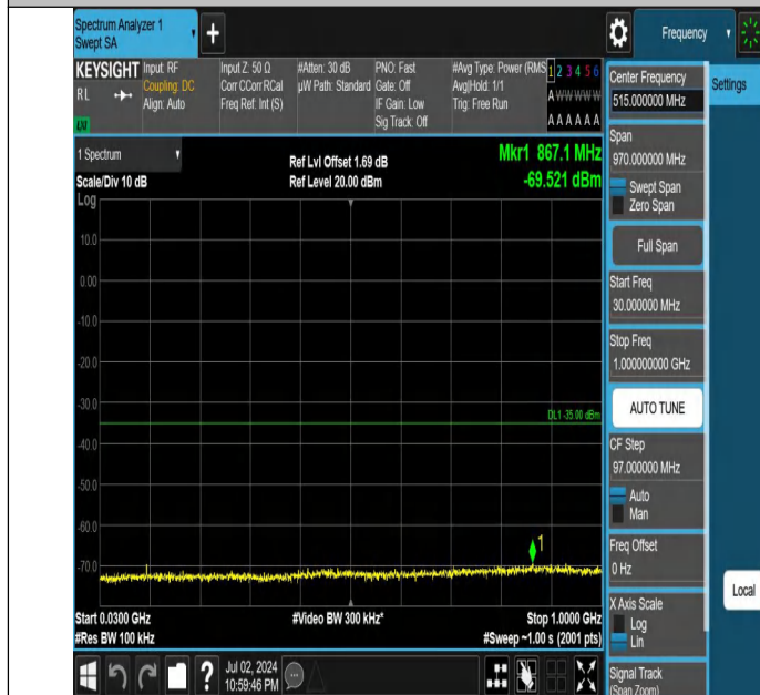
Band7-15MHz-QPSK-20825-1RB#0-30~1000-PASS
