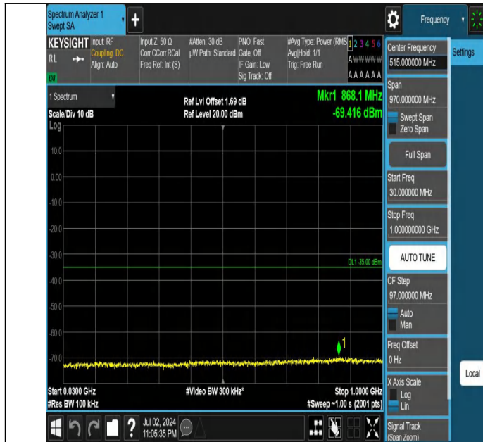
Band7-20MHz-QPSK-21350-1RB#0-30~1000-PASS
