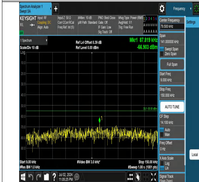
Band7-20MHz-QPSK-21350-1RB#0-0.009~0.15-PASS
