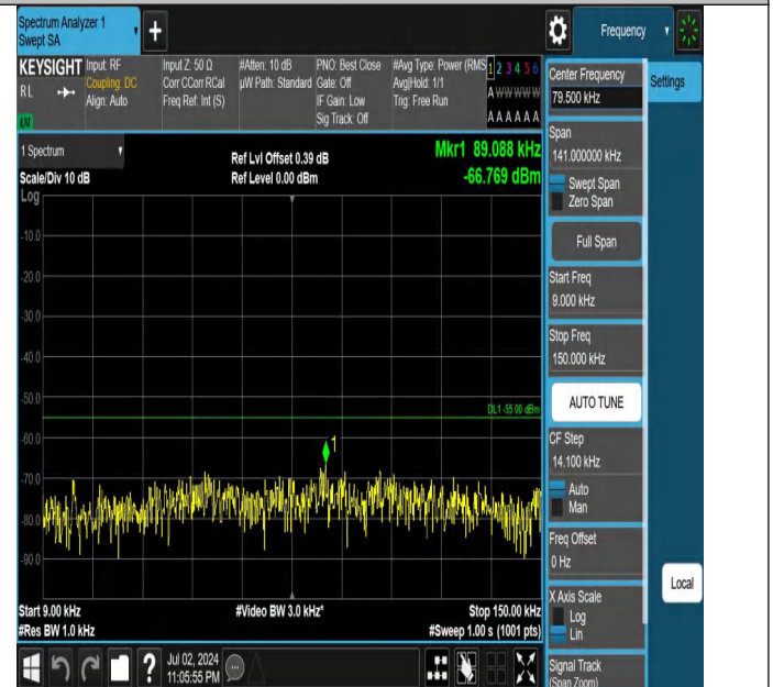
Band7-20MHz-QPSK-21350-1RB#99-0.009~0.15-PASS
