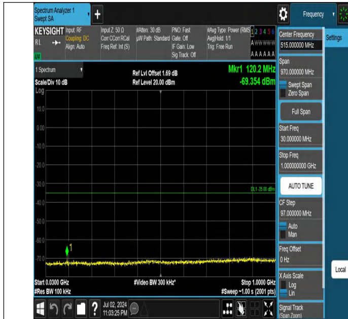
Band7-20MHz-QPSK-20850-1RB#0-30~1000-PASS
