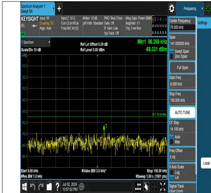
Band7-10MHz-21100-21100-1RB#0-0.009~0.15-PASS
