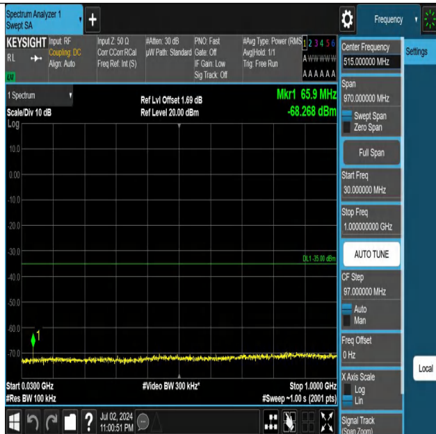
Band7-15MHz-QPSK-21100-1RB#0-30~1000-PASS
