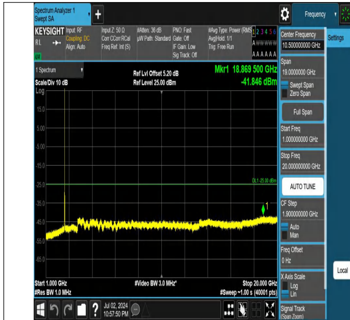
Band7-10MHz-21100-21100-1RB#49-1000~20000-PASS
