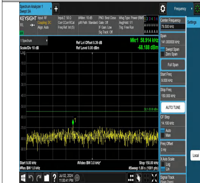
Band7-15MHz-QPSK-21100-1RB#0-0.009~0.15-PASS
