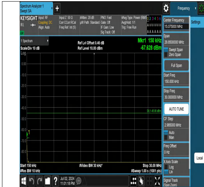
Band7-15MHz-QPSK-21100-1RB#74-0.15~30-PASS
