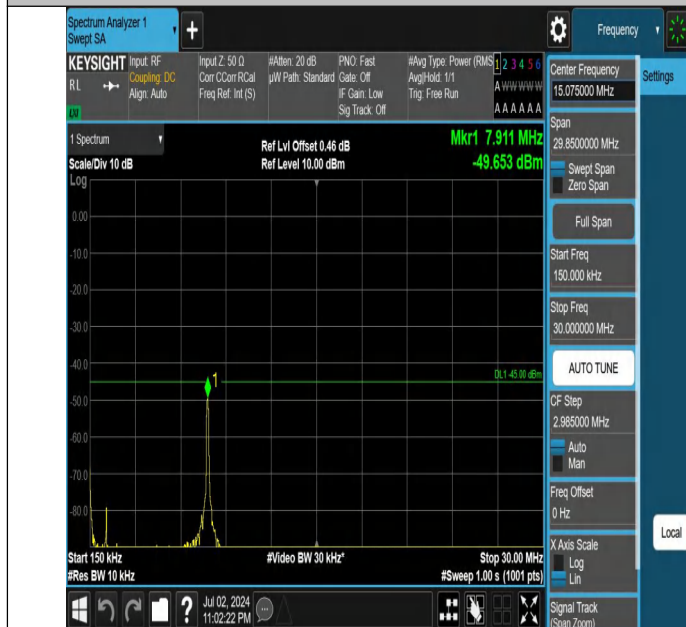
Band7-15MHz-QPSK-21375-1RB#74-0.15~30-PASS
