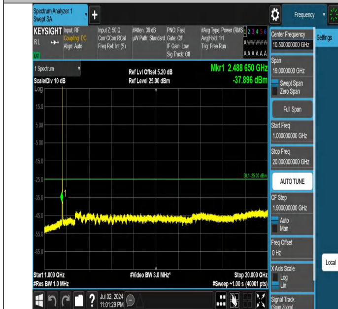
Band7-15MHz-QPSK-21100-1RB#74-1000~20000-PASS
