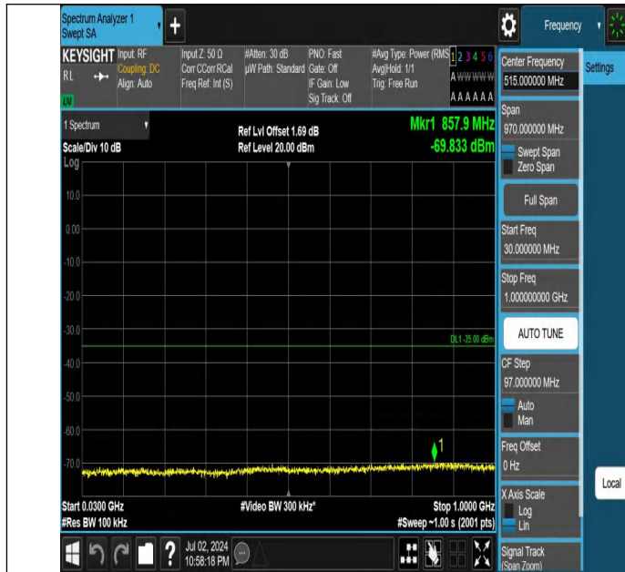
Band7-10MHz-21100-21400-1RB#0-30~1000-PASS
