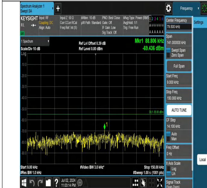
Band7-20MHz-QPSK-20850-1RB#0-0.009~0.15-PASS
