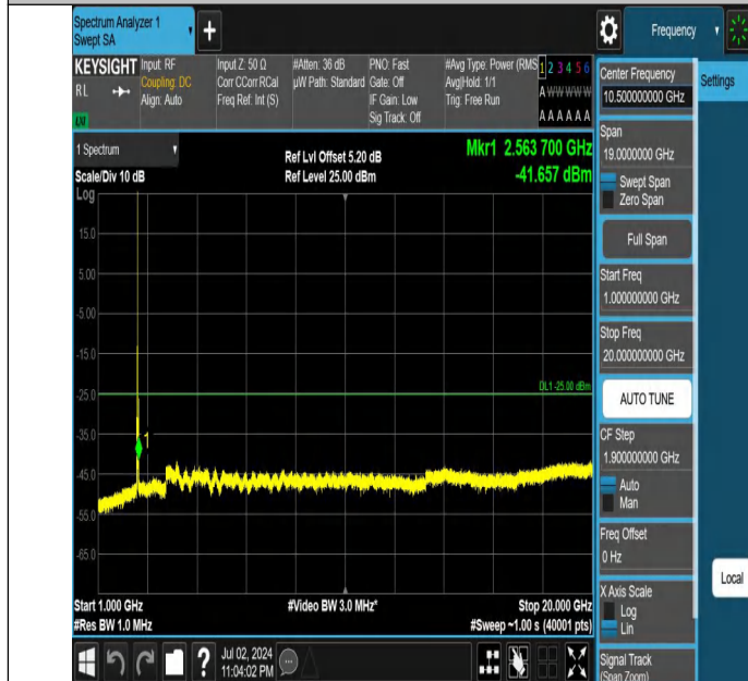
Band7-20MHz-QPSK-20850-1RB#99-1000~20000-PASS
