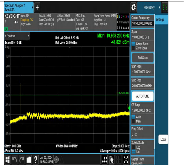
Band7-10MHz-21100-21400-1RB#0-1000~20000-PASS
