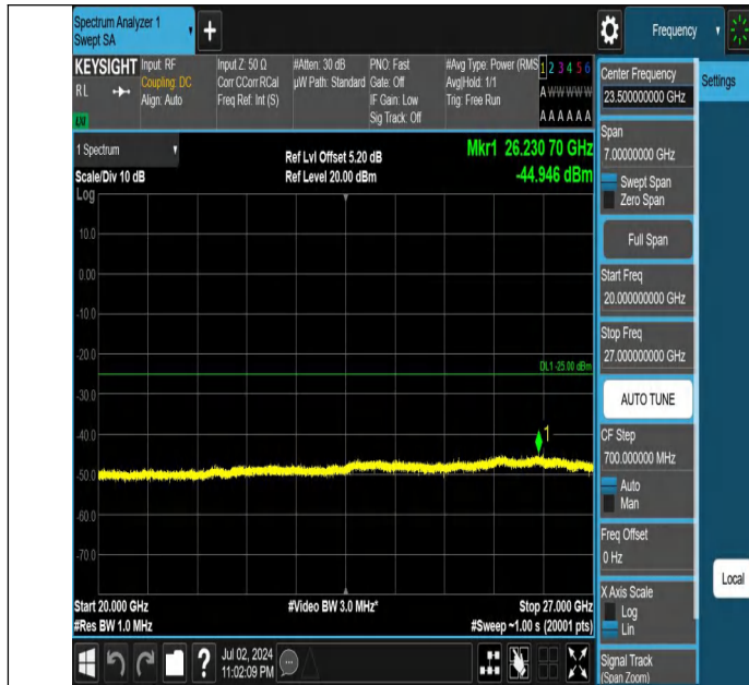
Band7-15MHz-QPSK-21375-1RB#0-20000~27000-PASS
