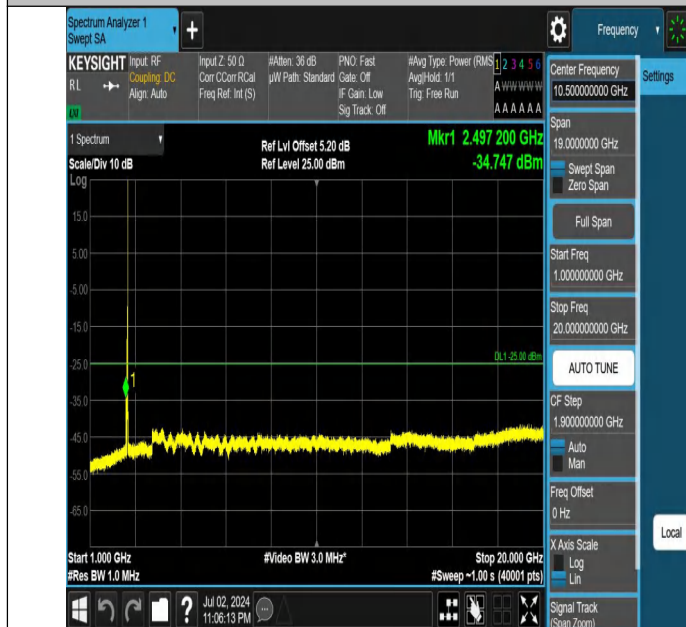
Band7-20MHz-QPSK-21350-1RB#99-1000~20000-PASS
