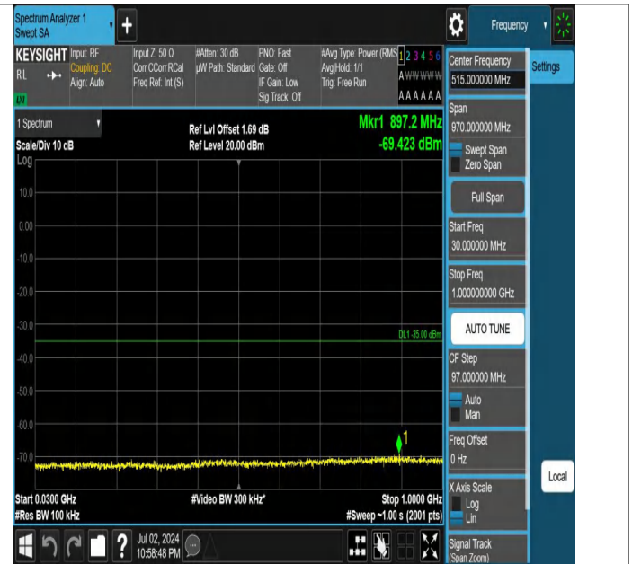
Band7-10MHz-21100-21400-1RB#49-30~1000-PASS
