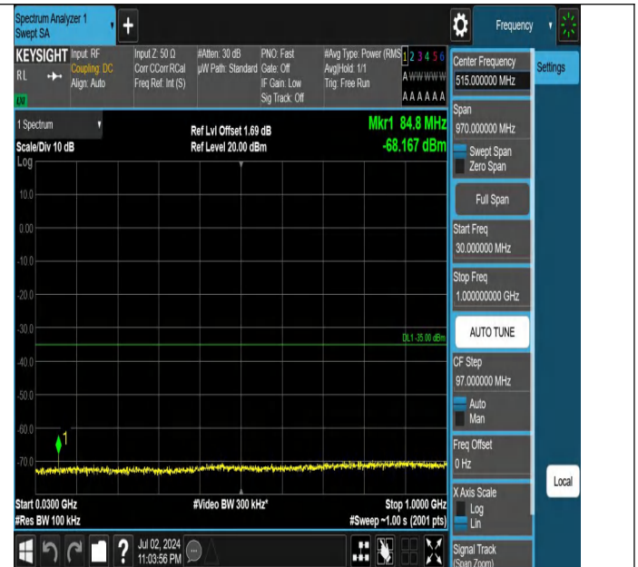
Band7-20MHz-QPSK-20850-1RB#99-30~1000-PASS
