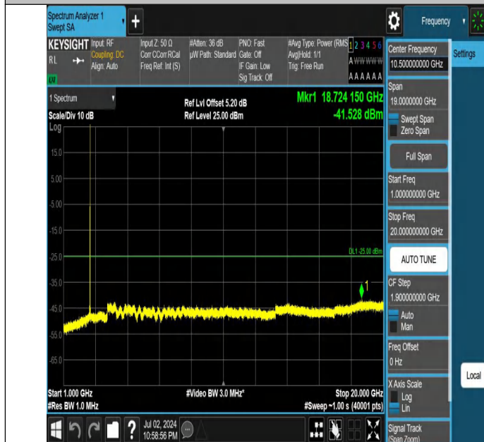
Band7-10MHz-21100-21400-1RB#49-1000~20000-PASS
