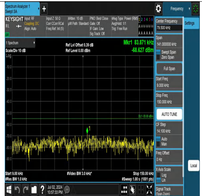
Band7-10MHz-21100-21100-1RB#49-0.009~0.15-PASS
