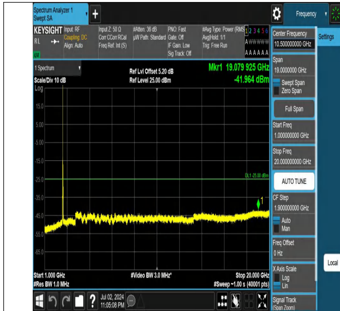
Band7-20MHz-QPSK-21100-1RB#99-1000~20000-PASS
