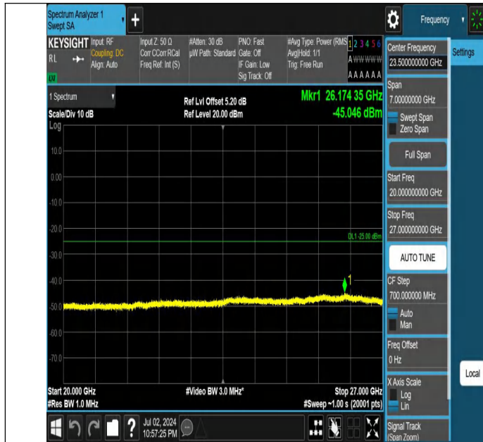
Band7-10MHz-21100-21100-1RB#0-20000~27000-PASS
