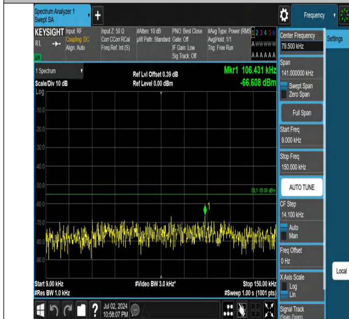
Band7-10MHz-21100-21400-1RB#0-0.009~0.15-PASS
