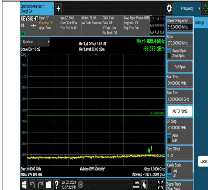
Band7-10MHz-21100-21100-1RB#0-30~1000-PASS
