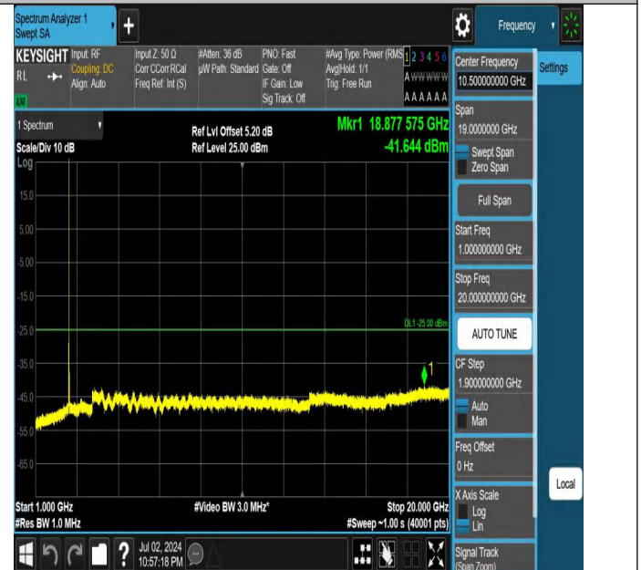
Band7-10MHz-21100-21100-1RB#0-1000~20000-PASS
