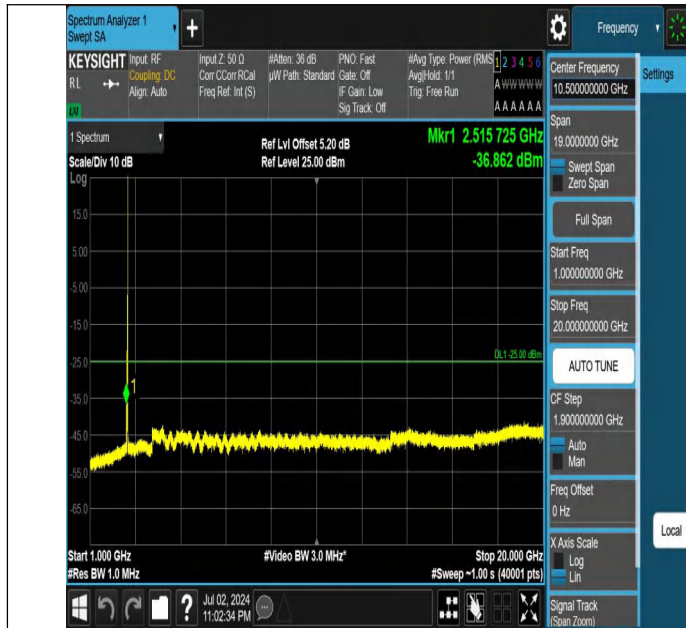
Band7-15MHz-QPSK-21375-1RB#74-1000~20000-PASS
