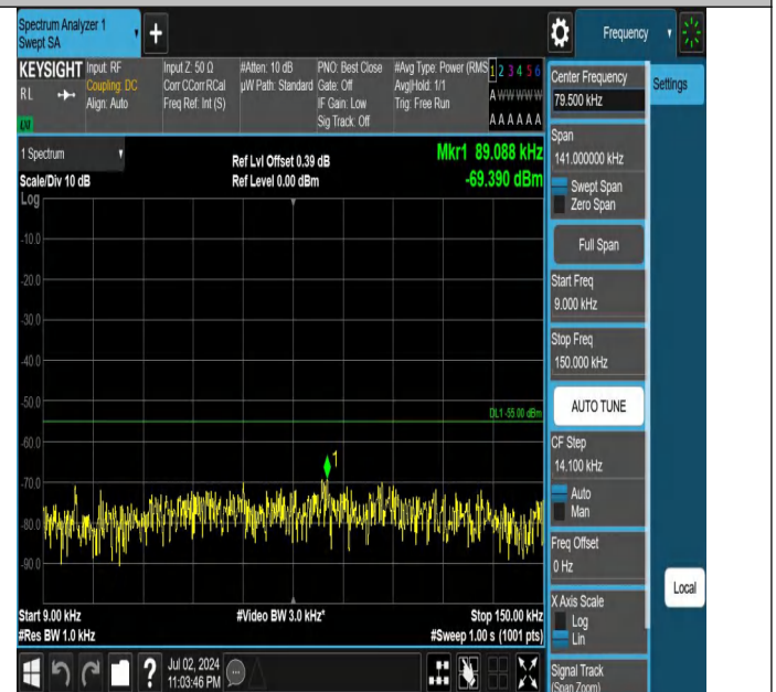
Band7-20MHz-QPSK-20850-1RB#99-0.009~0.15-PASS
