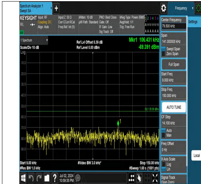
Band7-15MHz-QPSK-20825-1RB#0-0.009~0.15-PASS
