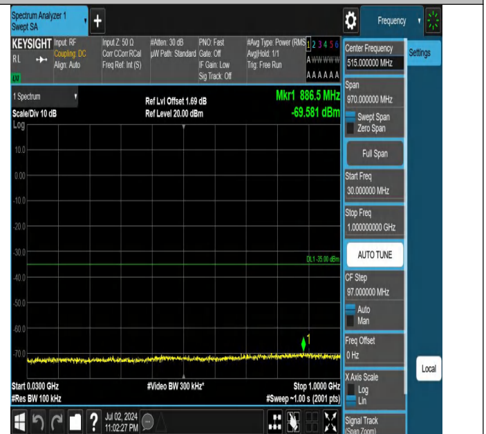
Band7-15MHz-QPSK-21375-1RB#74-30~1000-PASS
