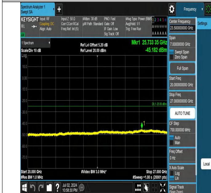
Band7-10MHz-21100-21400-1RB#0-20000~27000-PASS
