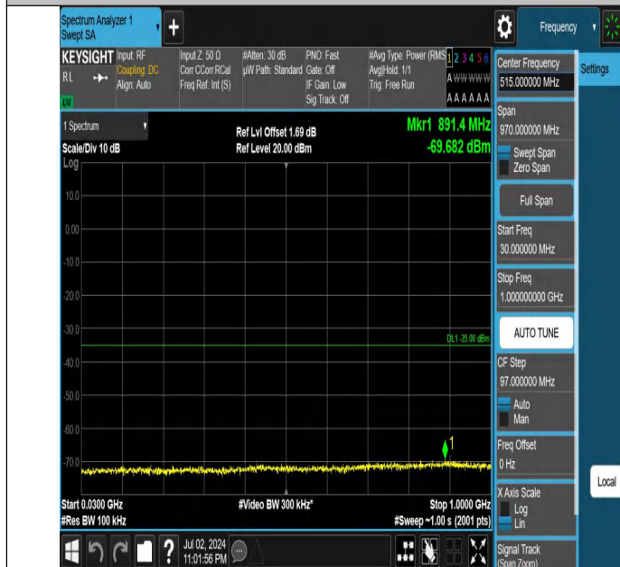
Band7-15MHz-QPSK-21375-1RB#0-30~1000-PASS
