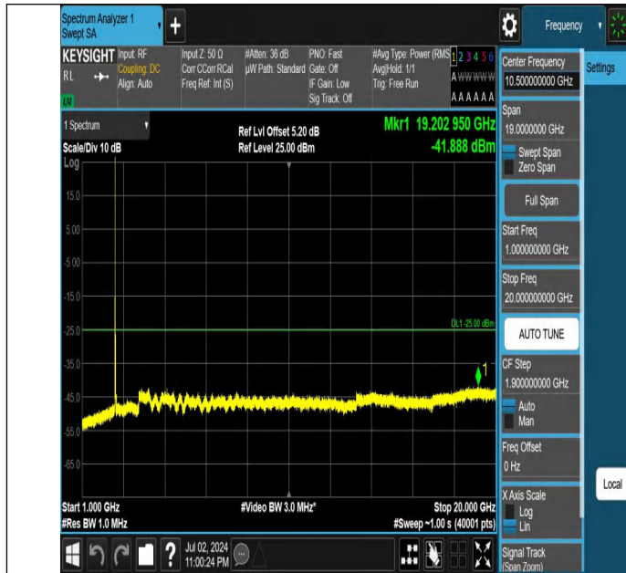
Band7-15MHz-QPSK-20825-1RB#74-1000~20000-PASS
