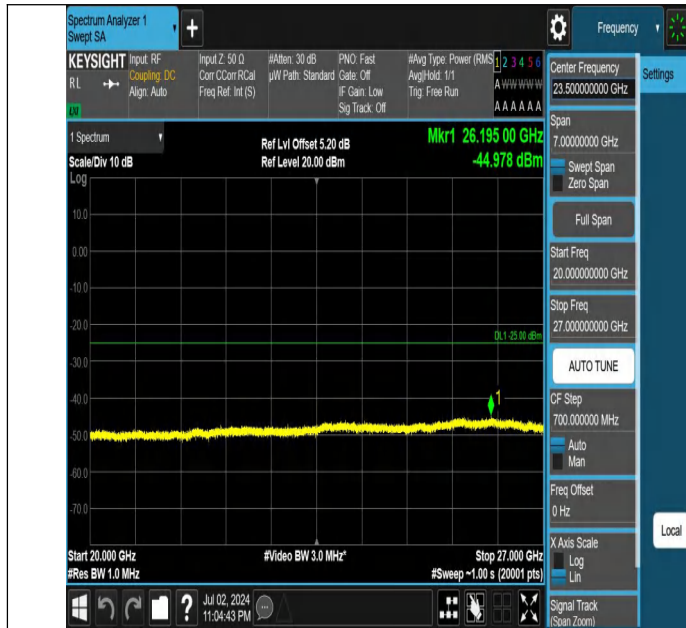
Band7-20MHz-QPSK-21100-1RB#0-20000~27000-PASS
