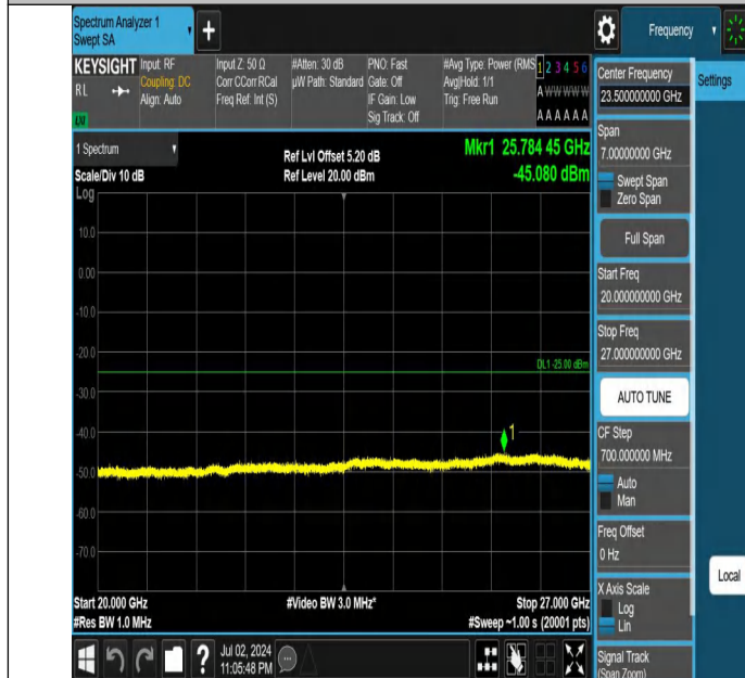
Band7-20MHz-QPSK-21350-1RB#0-20000~27000-PASS
