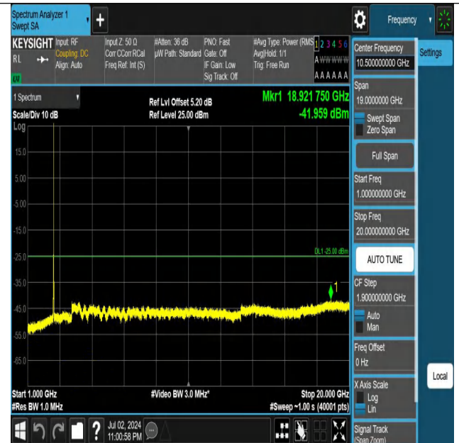
Band7-15MHz-QPSK-21100-1RB#0-1000~20000-PASS
