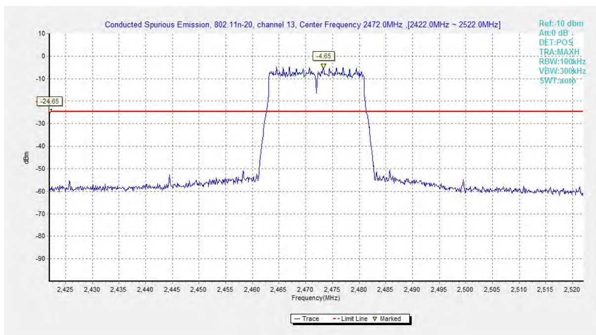
Fig.A.6.1.113 Conducted Spurious Emission (802.11 n-HT20, Ch13, Center Frequency)
