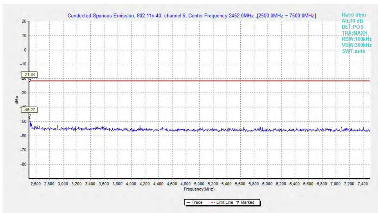
Fig.A.6.1.140 Conducted Spurious Emission (802.11n-HT40, Ch9, 2.5 GHz-7.5 GHz)
