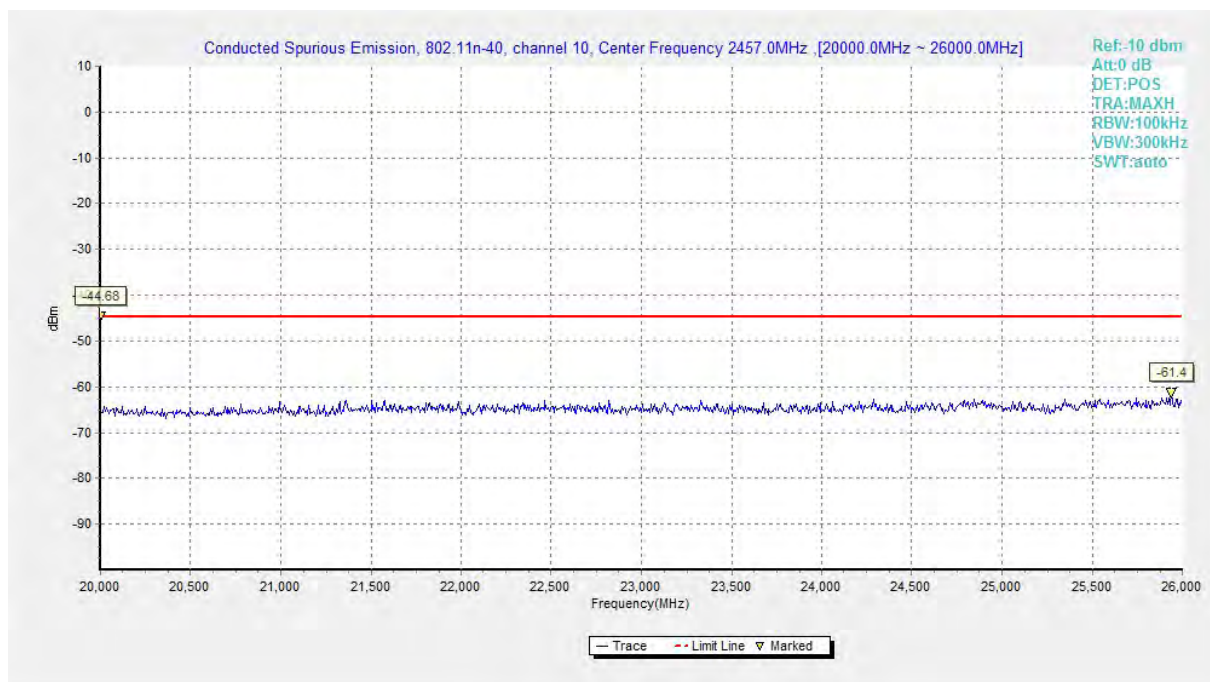
Fig.A.6.1.152 Conducted Spurious Emission (802.11 n-HT40, Ch10, 20 GHz-26 GHz)
