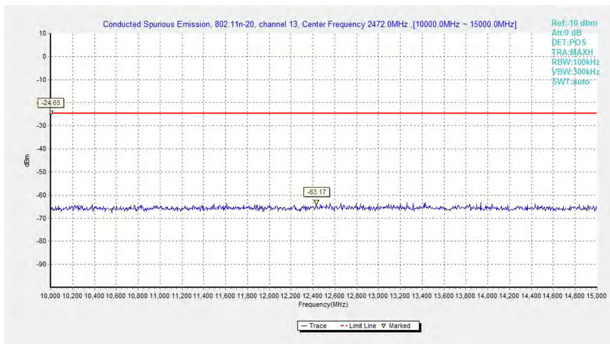
Fig.A.6.1.118 Conducted Spurious Emission (802.11 n-HT20, Ch13, 10 GHz-15 GHz)
