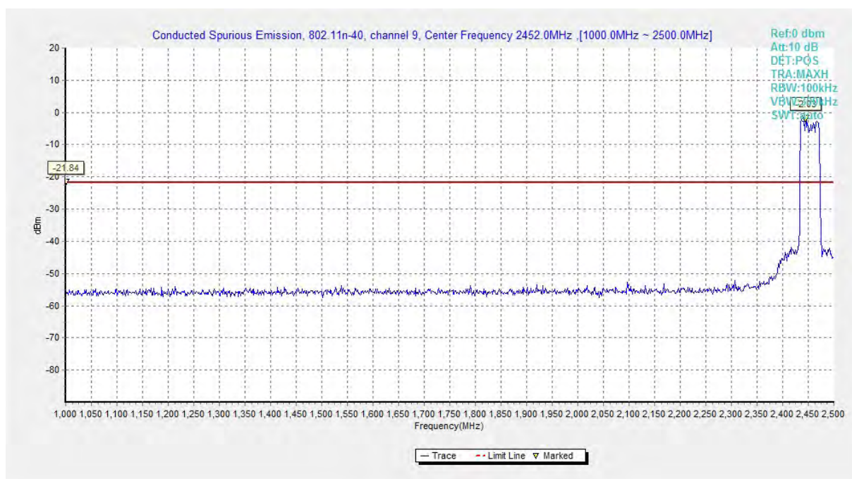
Fig.A.6.1.139 Conducted Spurious Emission (802.11n-HT40, Ch9, 1 GHz-2.5 GHz)
