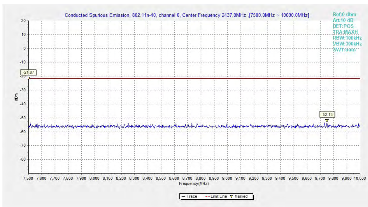
Fig.A.6.1.133 Conducted Spurious Emission (802.11n-HT40, Ch6, 7.5 GHz-10 GHz)
