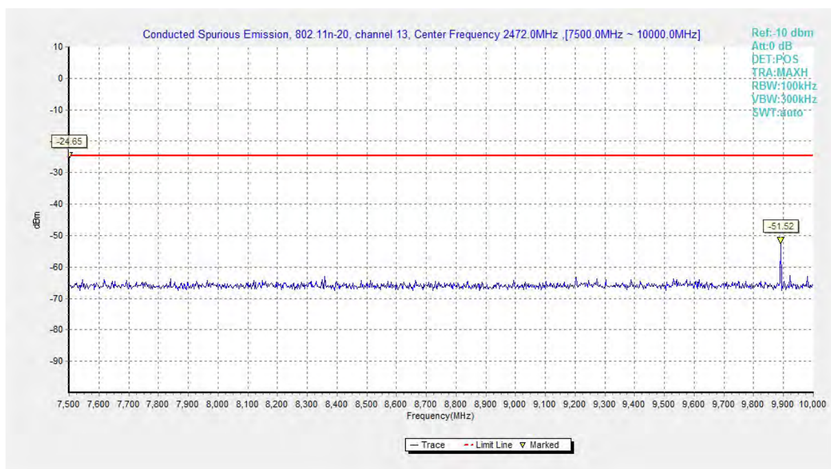
Fig.A.6.1.117 Conducted Spurious Emission (802.11 n-HT20, Ch13, 7.5 GHz-10 GHz)
