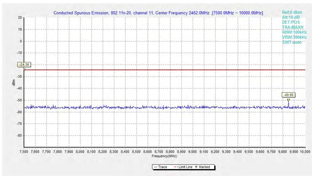
Fig.A.6.1.101 Conducted Spurious Emission (802.11n-HT20, Ch11, 7.5 GHz-10 GHz)
