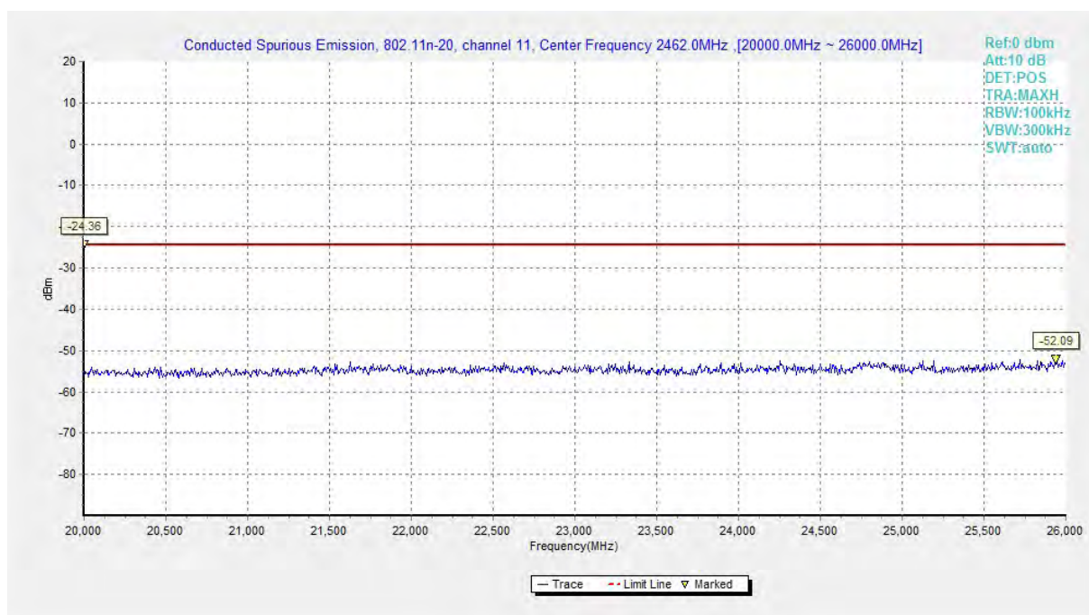
Fig.A.6.1.104 Conducted Spurious Emission (802.11n-HT20, Ch11, 20 GHz-26 GHz)
