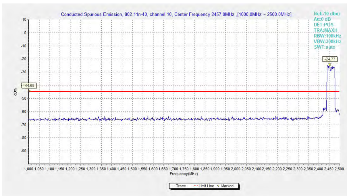
Fig.A.6.1.147 Conducted Spurious Emission (802.11 n-HT40, Ch10, 1 GHz-2.5 GHz)
