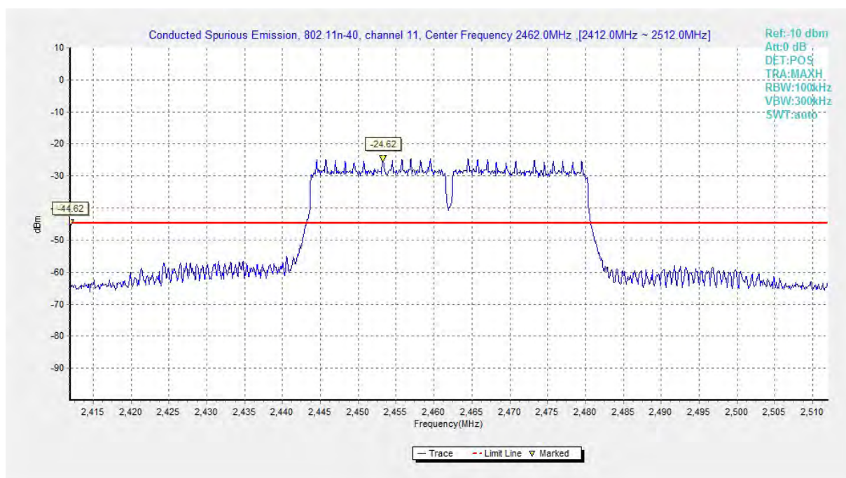
Fig.A.6.1.153 Conducted Spurious Emission (802.11 n-HT40, Ch11, Center Frequency)
