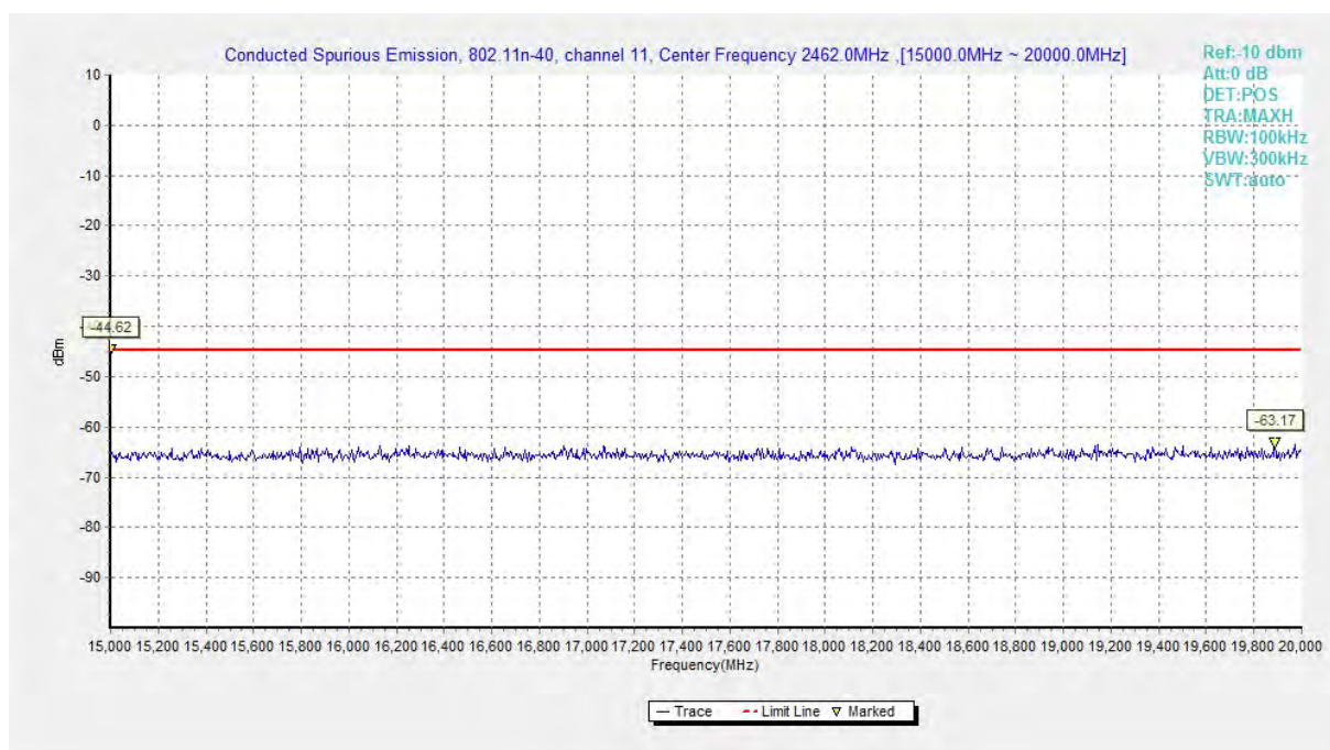
Fig.A.6.1.159 Conducted Spurious Emission (802.11 n-HT40, Ch11, 15 GHz-20 GHz)
