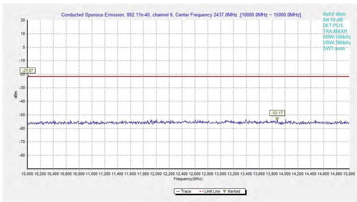
Fig.A.6.1.134 Conducted Spurious Emission (802.11n-HT40, Ch6, 10 GHz-15 GHz)
