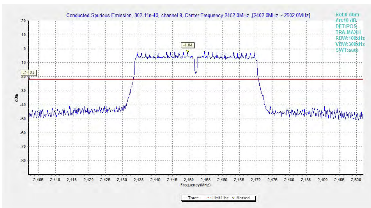
Fig.A.6.1.137 Conducted Spurious Emission (802.11n-HT40, Ch9, Center Frequency)
