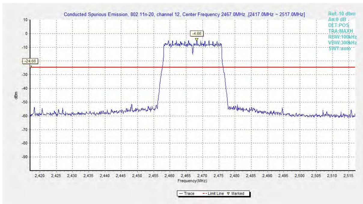
Fig.A.6.1.105 Conducted Spurious Emission (802.11 n-HT20, Ch12, Center Frequency)
