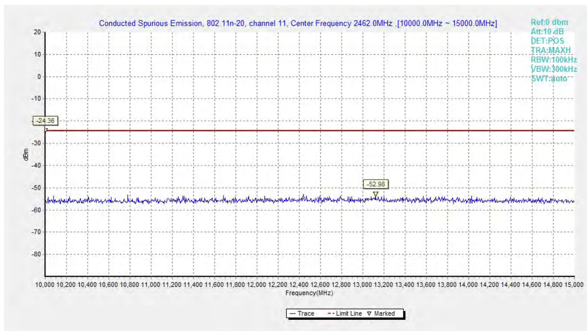
Fig.A.6.1.102 Conducted Spurious Emission (802.11n-HT20, Ch11, 10 GHz-15 GHz)
