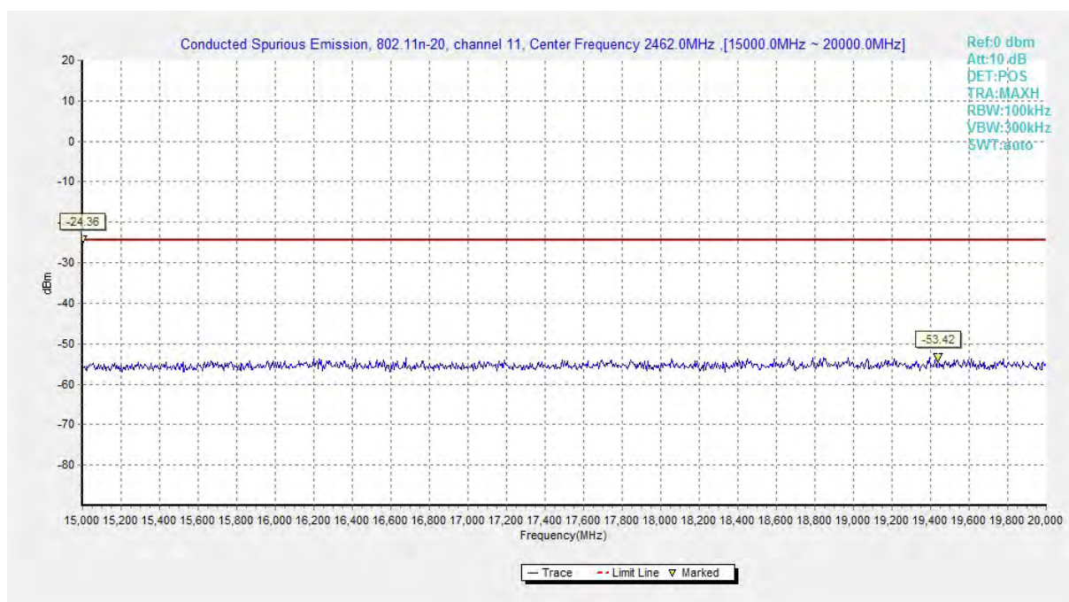
Fig.A.6.1.103 Conducted Spurious Emission (802.11n-HT20, Ch11, 15 GHz-20 GHz)
