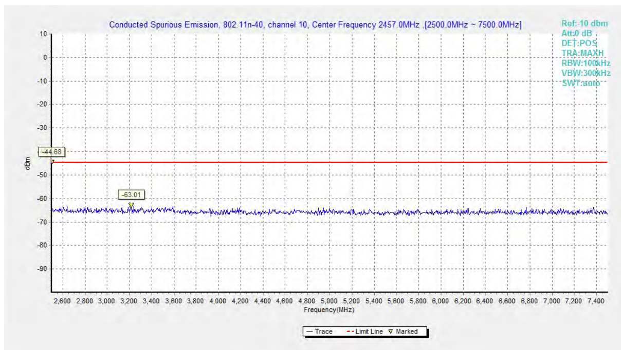
Fig.A.6.1.148 Conducted Spurious Emission (802.11 n-HT40, Ch10, 2.5 GHz-7.5 GHz)
