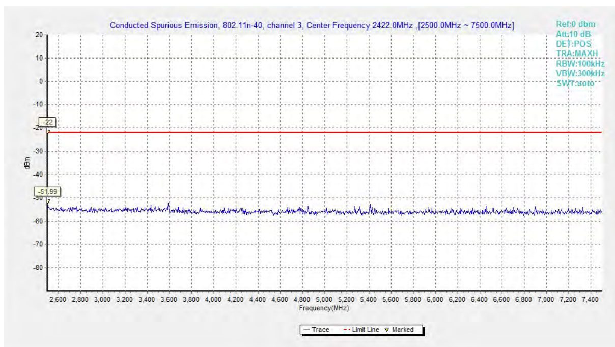
Fig.A.6.1.124 Conducted Spurious Emission (802.11n-HT40, Ch3, 2.5 GHz-7.5 GHz)
