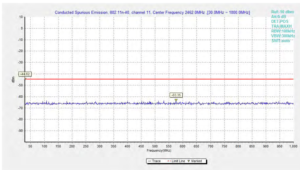
Fig.A.6.1.154 Conducted Spurious Emission (802.11 n-HT40, Ch11, 30 MHz-1 GHz)
