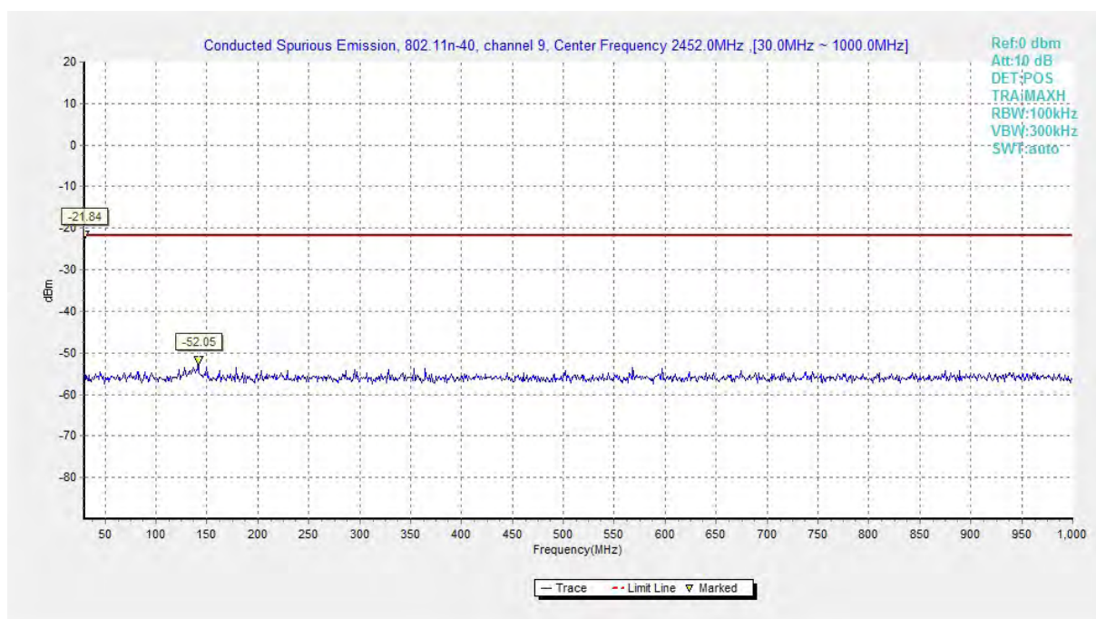
Fig.A.6.1.138 Conducted Spurious Emission (802.11n-HT40, Ch9, 30 MHz-1 GHz)
