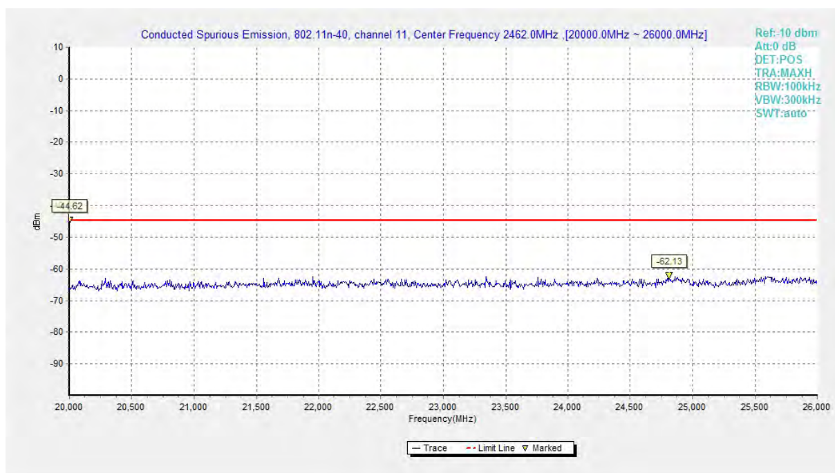
Fig.A.6.1.160 Conducted Spurious Emission (802.11 n-HT40, Ch11, 20 GHz-26 GHz)
