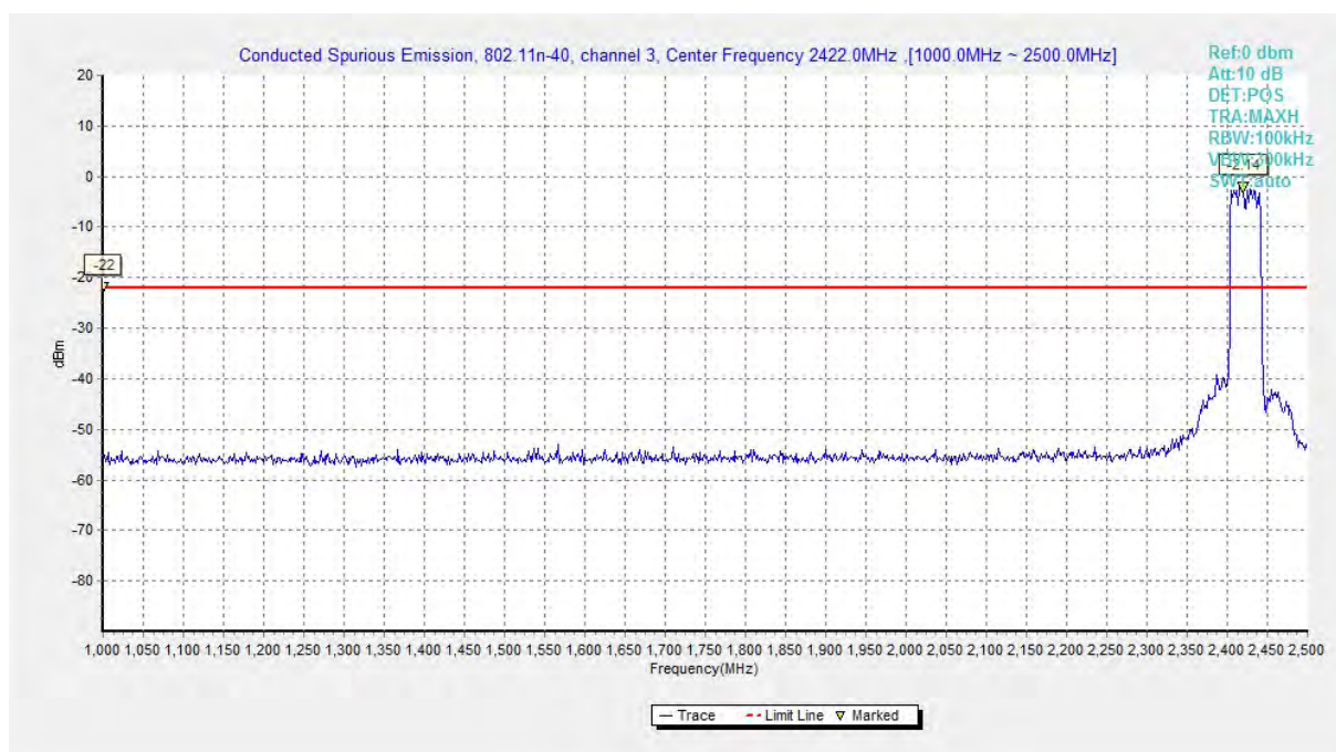
Fig.A.6.1.123 Conducted Spurious Emission (802.11n-HT40, Ch3, 1 GHz-2.5 GHz)
