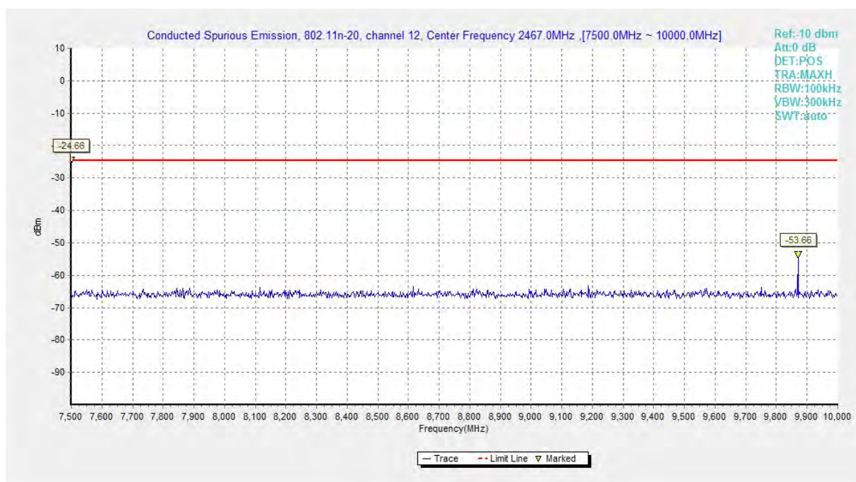
Fig.A.6.1.109 Conducted Spurious Emission (802.11 n-HT20, Ch12, 7.5 GHz-10 GHz)
