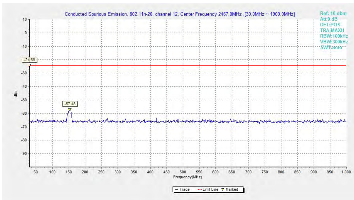
Fig.A.6.1.106 Conducted Spurious Emission (802.11 n-HT20, Ch12, 30 MHz-1 GHz)
