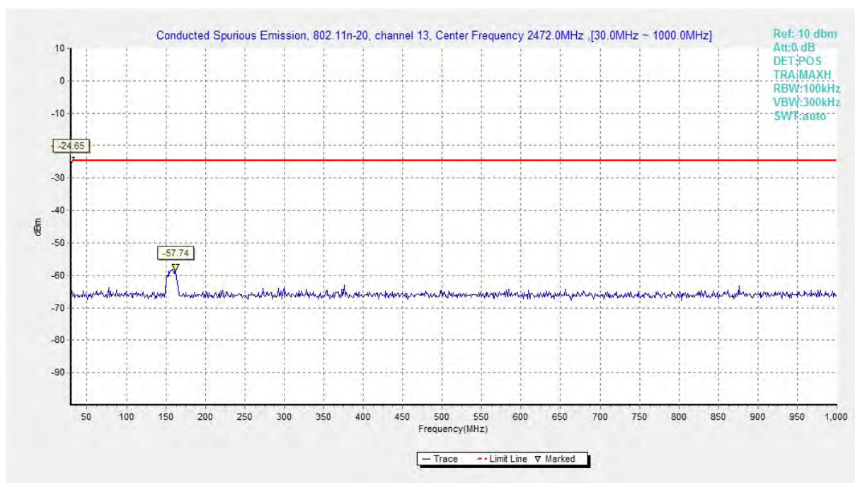
Fig.A.6.1.114 Conducted Spurious Emission (802.11 n-HT20, Ch13, 30 MHz-1 GHz)
