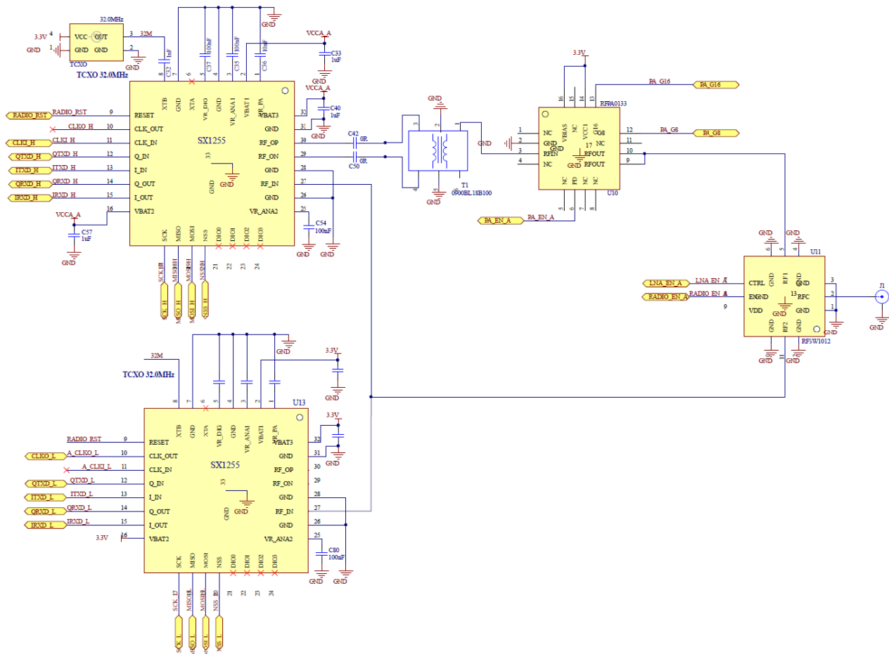
Figure5:RAK833cardinnerschematic.
