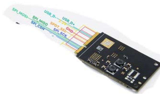
Figure3:Module Interface
