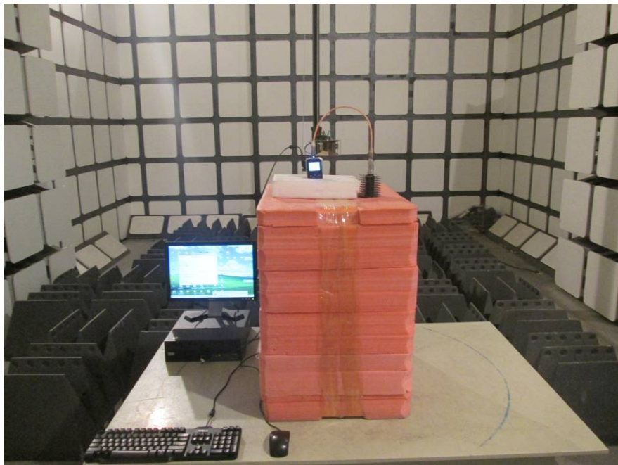
Transmitting Radiated Emissions View (Above 1 GHz)
