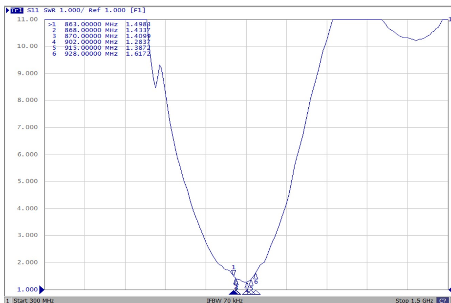
Standing wave ratio data
