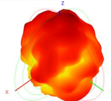
5850.0MHz H+V, Eff: 44.5%
