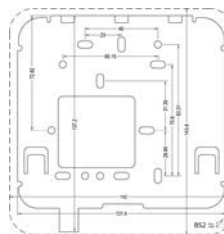
Drilling Template
