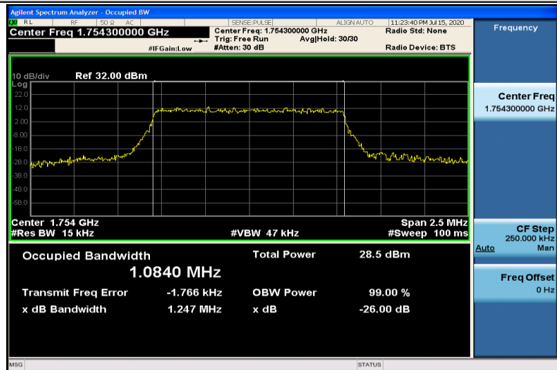
Band4-1.4MHz-16QAM-20393-6RB#0-1.0840
