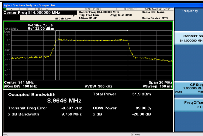
Band5-10MHz-QPSK-20600-50RB#0-8.9646
