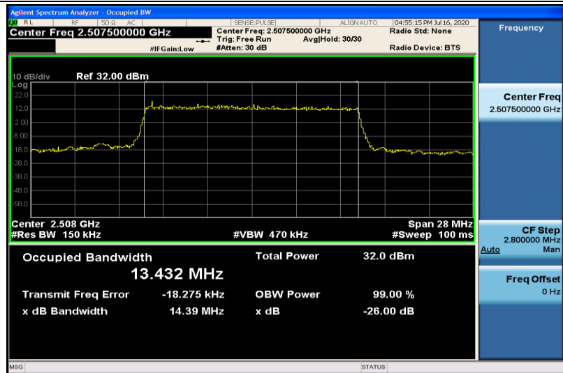
Band7-15MHz-QPSK-20825-75RB#0-13.432
