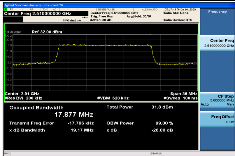
Band7-20MHz-QPSK-20850-100RB#0-17.877
