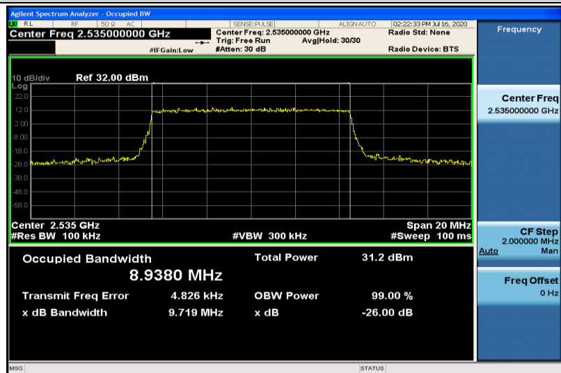
Band7-10MHz-16QAM-21100-50RB#0-8.9380
