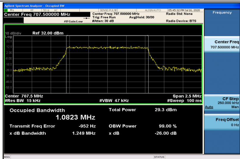
Band12-1.4MHz-16QAM-23095-6RB#0-1.0823
