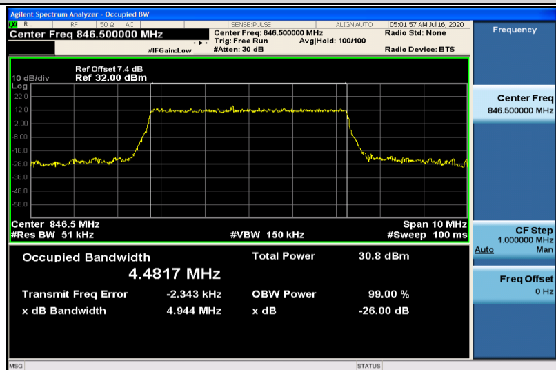
Band5-5MHz-16QAM-20625-25RB#0-4.4817
