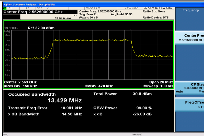
Band7-15MHz-16QAM-21375-75RB#0-13.429
