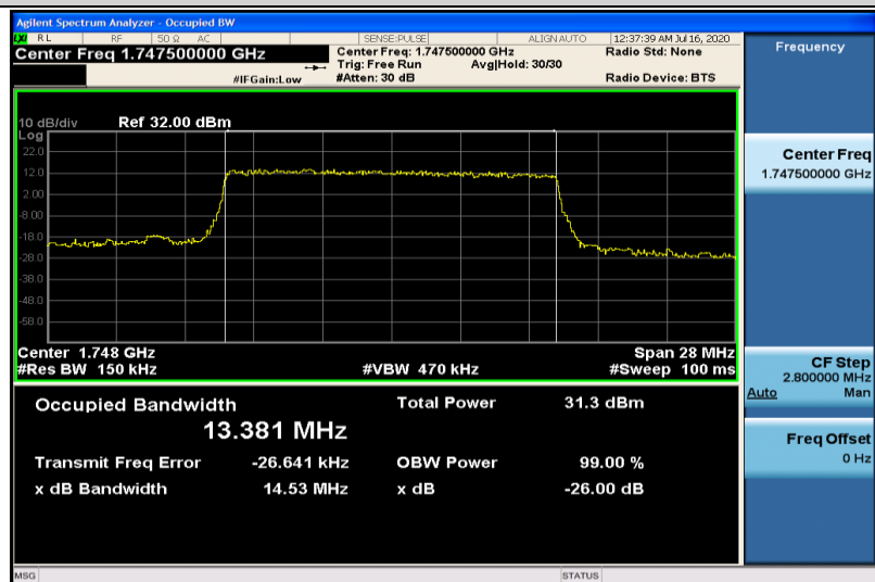
Band4-15MHz-QPSK-20325-75RB#0-13.381
