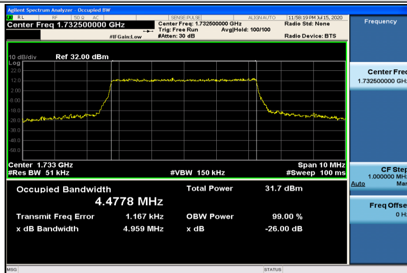
Band4-5MHz-QPSK-20175-25RB#0-4.4778
