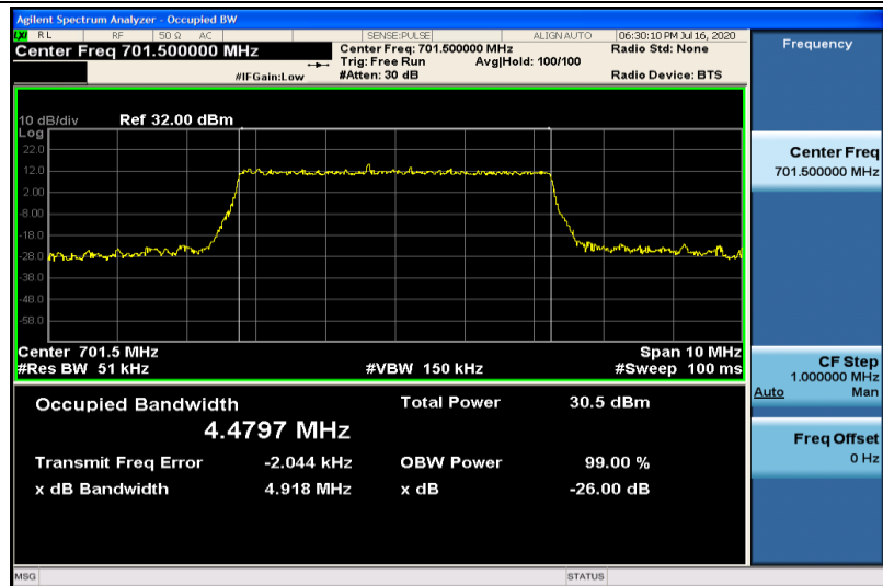
Band12-5MHz-16QAM-23035-25RB#0-4.4797
