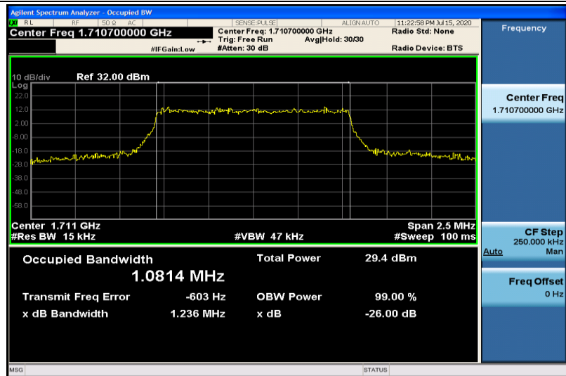
Band4-1.4MHz-16QAM-19957-6RB#0-1.0814
