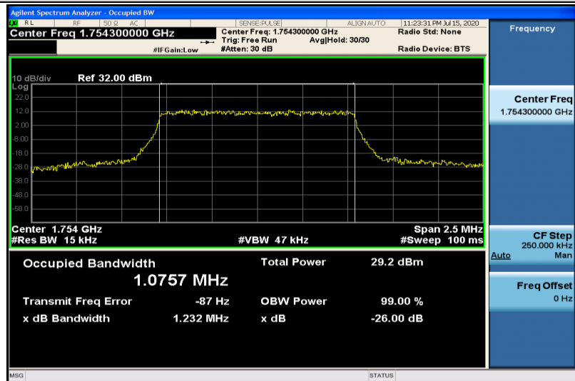
Band4-1.4MHz-QPSK-20393-6RB#0-1.0757
