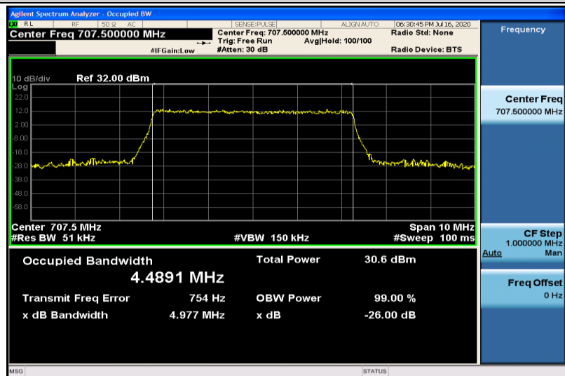
Band12-5MHz-16QAM-23095-25RB#0-4.4891
