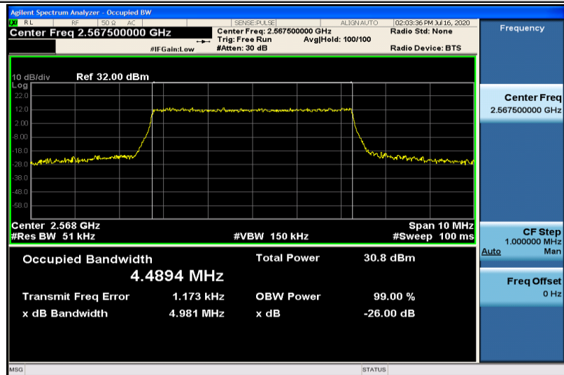
Band7-5MHz-16QAM-21425-25RB#0-4.4894
