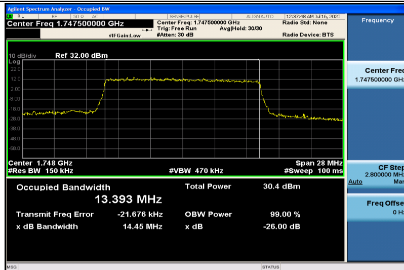
Band4-15MHz-16QAM-20325-75RB#0-13.393
