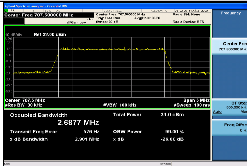
Band12-3MHz-QPSK-23095-15RB#0-2.6877
