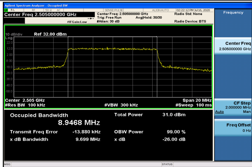
Band7-10MHz-16QAM-20800-50RB#0-8.9468
