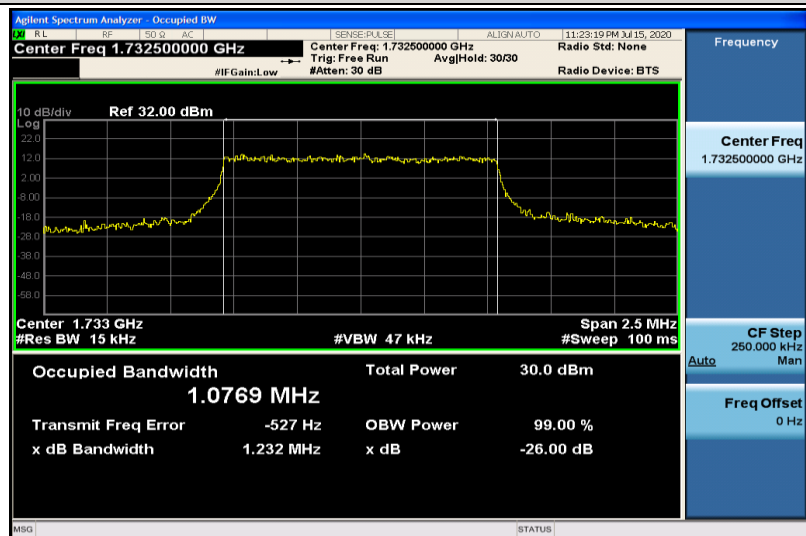
Band4-1.4MHz-16QAM-20175-6RB#0-1.0769
