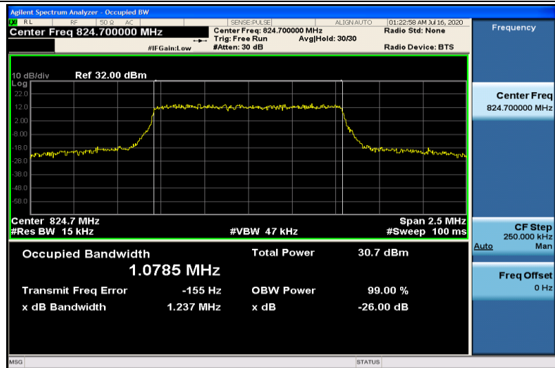
Band5-1.4MHz-QPSK-20407-6RB#0-1.0785
