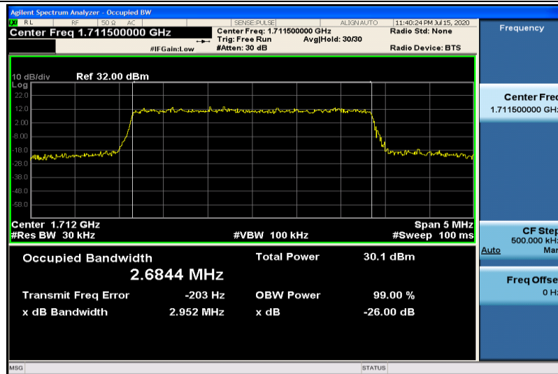
Band4-3MHz-16QAM-19965-15RB#0-2.6844
