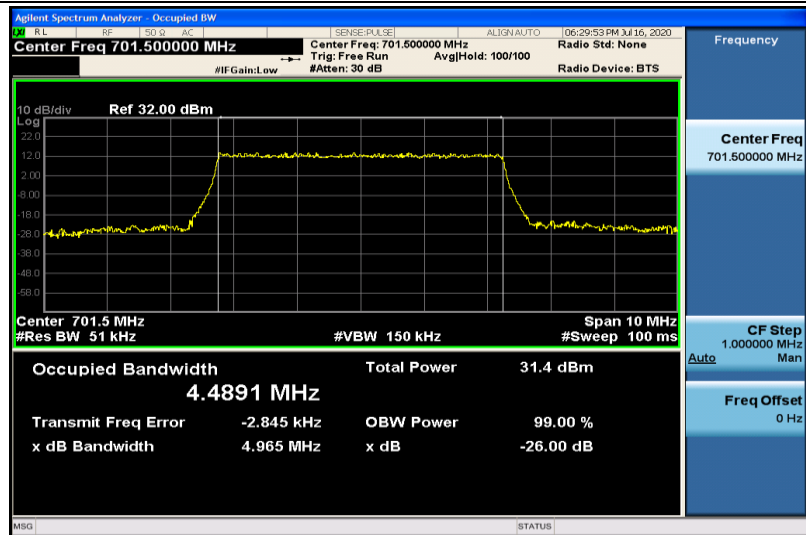
Band12-5MHz-QPSK-23035-25RB#0-4.4891
