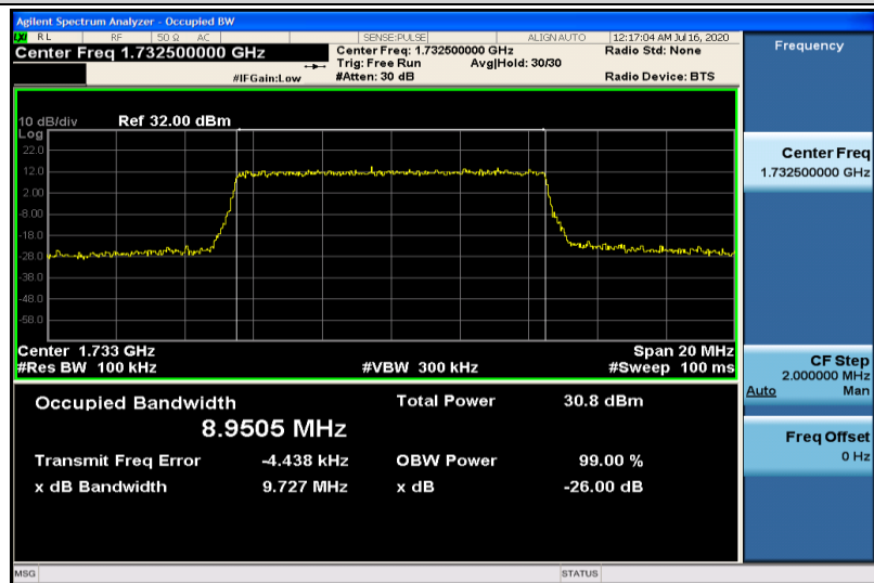
Band4-10MHz-16QAM-20175-50RB#0-8.9505
