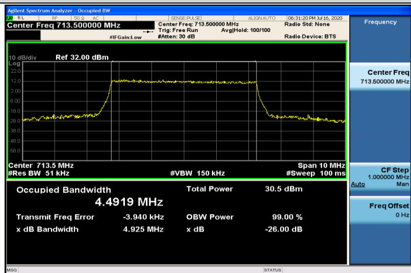
Band12-5MHz-16QAM-23155-25RB#0-4.4919
