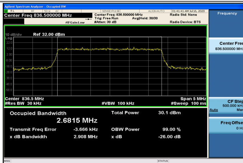
Band5-3MHz-16QAM-20525-15RB#0-2.6815
