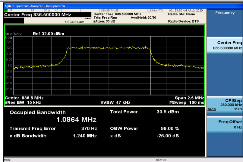
Band5-1.4MHz-QPSK-20525-6RB#0-1.0864
