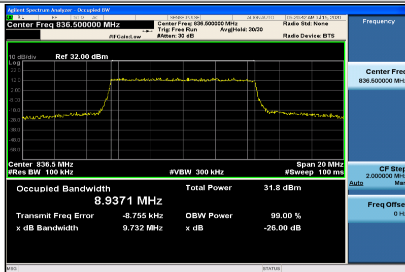
Band5-10MHz-QPSK-20525-50RB#0-8.9371
