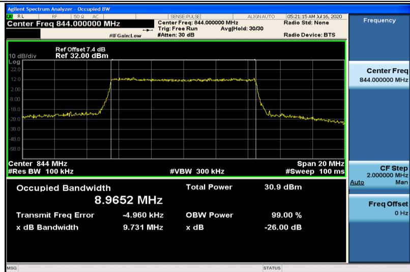
Band5-10MHz-16QAM-20600-50RB#0-8.9652
