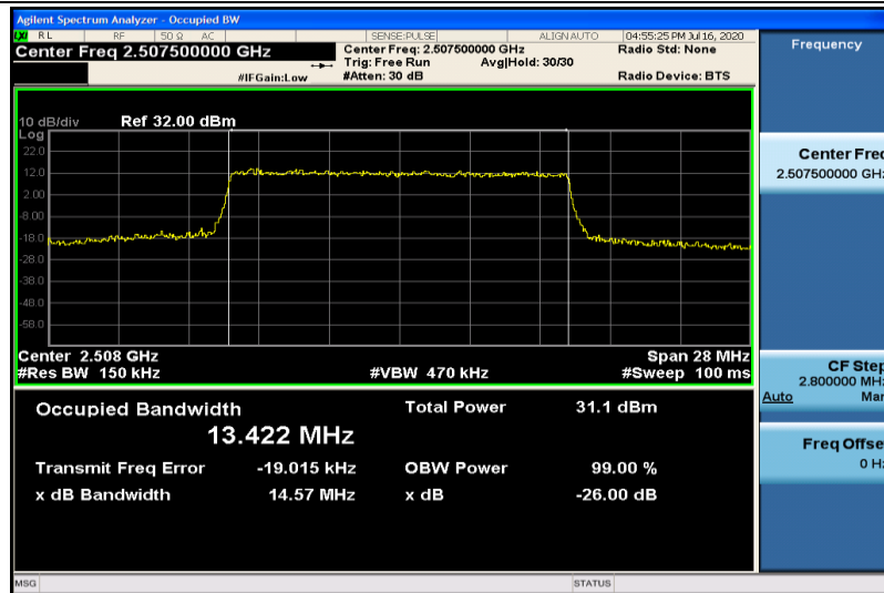
Band7-15MHz-16QAM-20825-75RB#0-13.422
