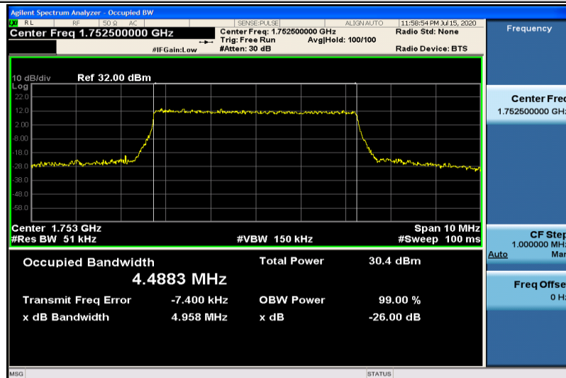
Band4-5MHz-QPSK-20375-25RB#0-4.4883
