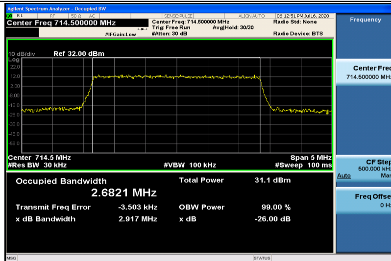
Band12-3MHz-QPSK-23165-15RB#0-2.6821
