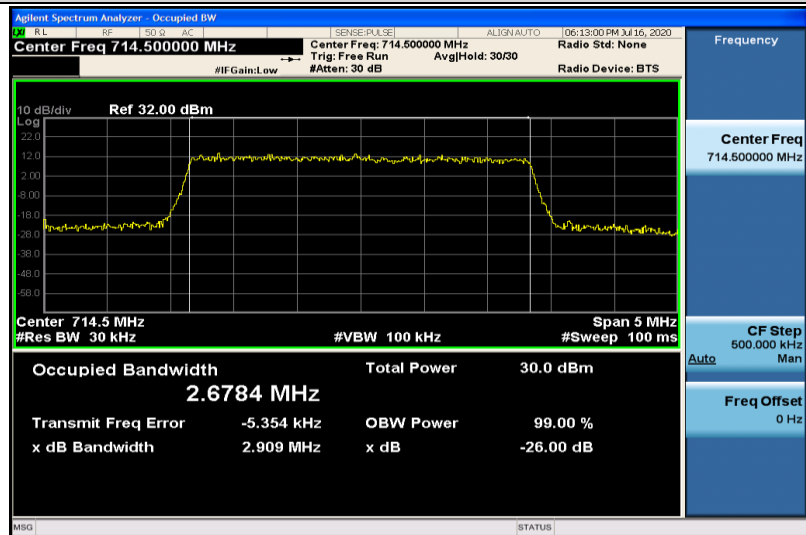
Band12-3MHz-16QAM-23165-15RB#0-2.6784
