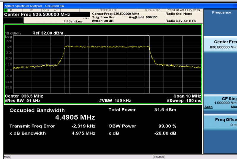
Band5-5MHz-QPSK-20525-25RB#0-4.4905
