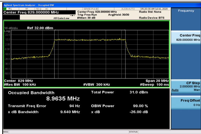
Band5-10MHz-16QAM-20450-50RB#0-8.9635
