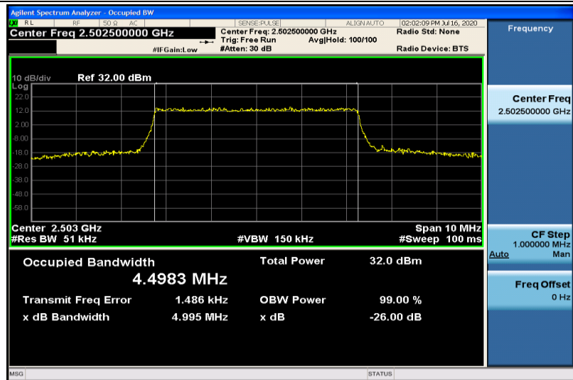
Band7-5MHz-QPSK-20775-25RB#0-4.4983
