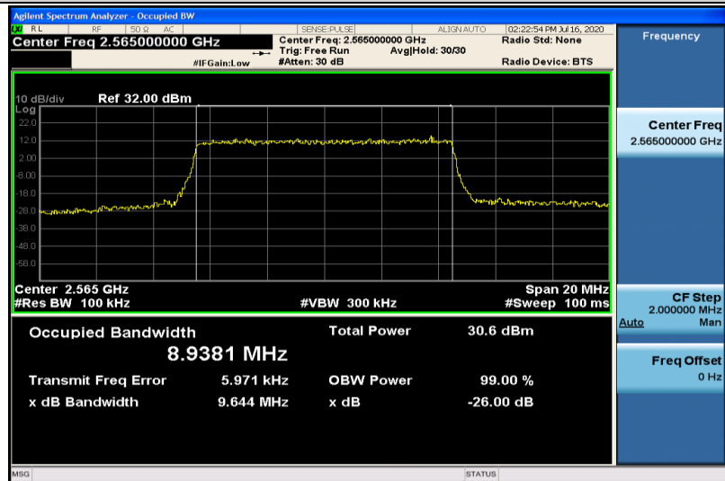
Band7-10MHz-16QAM-21400-50RB#0-8.9381
