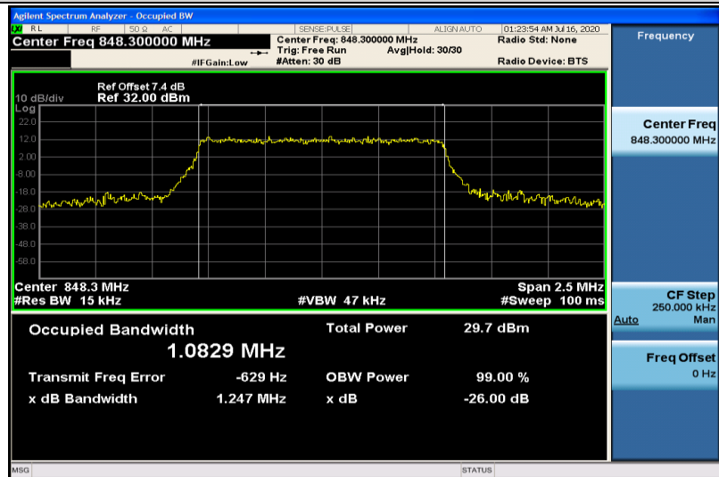
Band5-1.4MHz-16QAM-20643-6RB#0-1.0829
