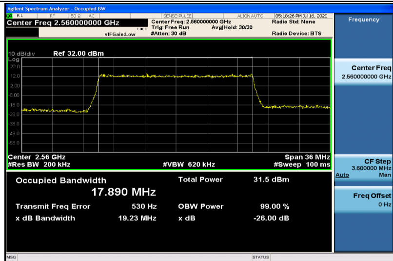
Band7-20MHz-QPSK-21350-100RB#0-17.890
