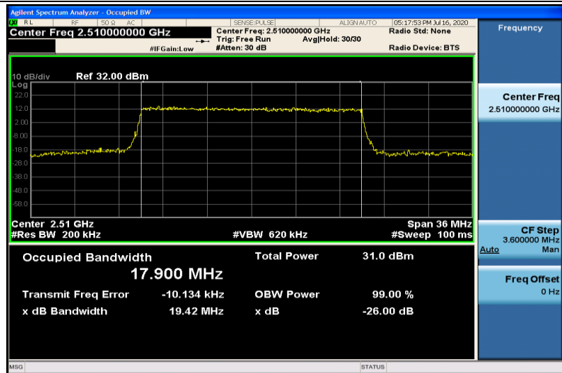
Band7-20MHz-16QAM-20850-100RB#0-17.900
