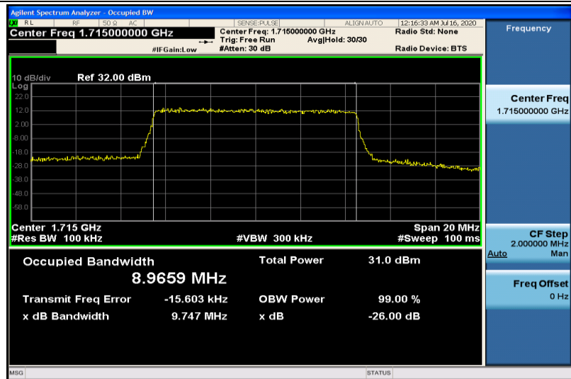
Band4-10MHz-QPSK-20000-50RB#0-8.9659
