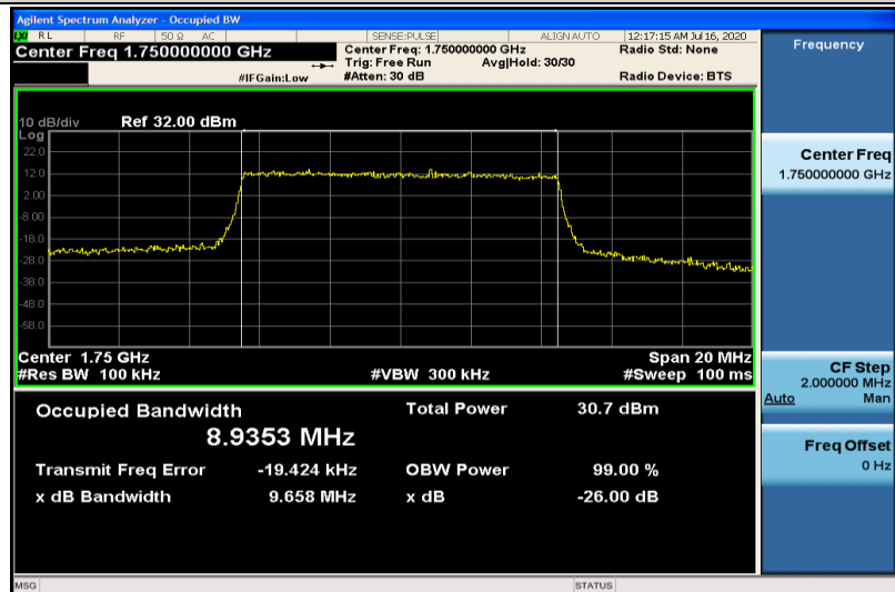
Band4-10MHz-QPSK-20350-50RB#0-8.9353
