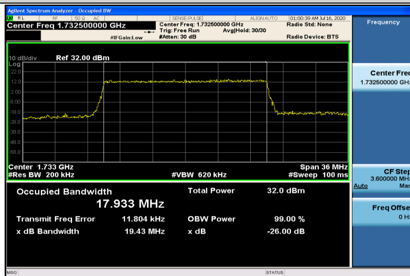
Band4-20MHz-QPSK-20175-100RB#0-17.933
