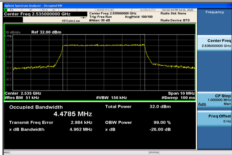
Band7-5MHz-QPSK-21100-25RB#0-4.4785
