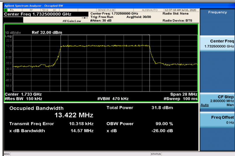
Band4-15MHz-QPSK-20175-75RB#0-13.422
