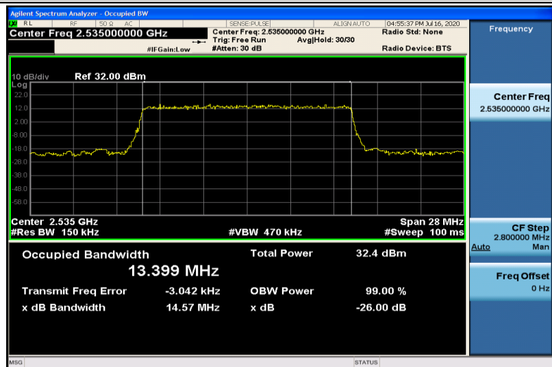
Band7-15MHz-QPSK-21100-75RB#0-13.399
