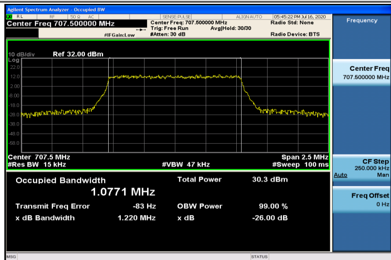
Band12-1.4MHz-QPSK-23095-6RB#0-1.0771
