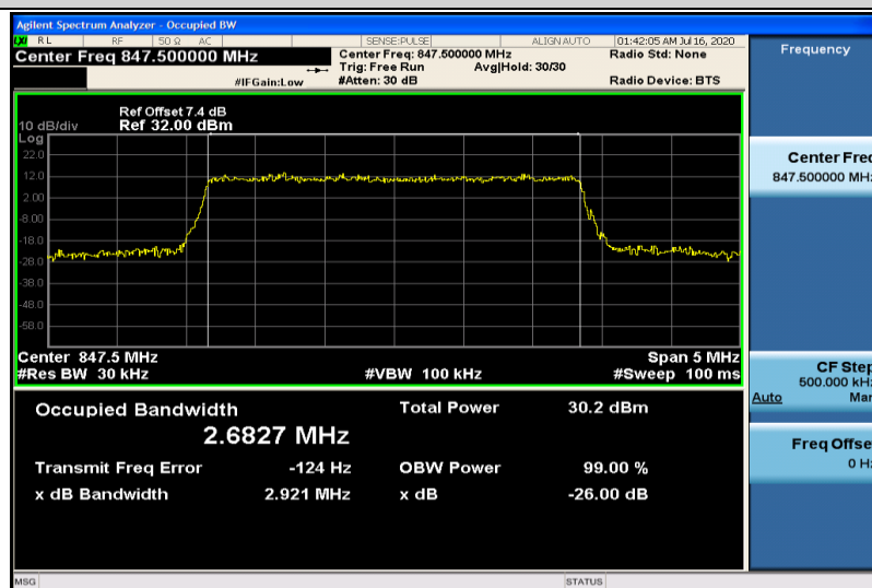
Band5-3MHz-16QAM-20635-15RB#0-2.6827
