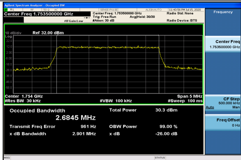
Band4-3MHz-QPSK-20385-15RB#0-2.6845
