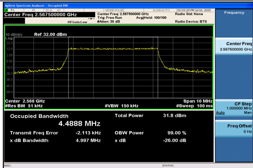
Band7-5MHz-QPSK-21425-25RB#0-4.4888
