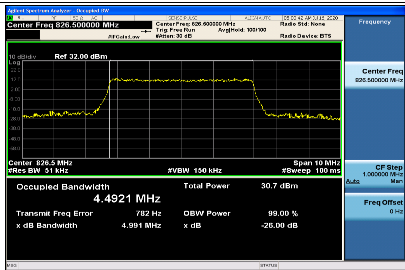
Band5-5MHz-16QAM-20425-25RB#0-4.4921
