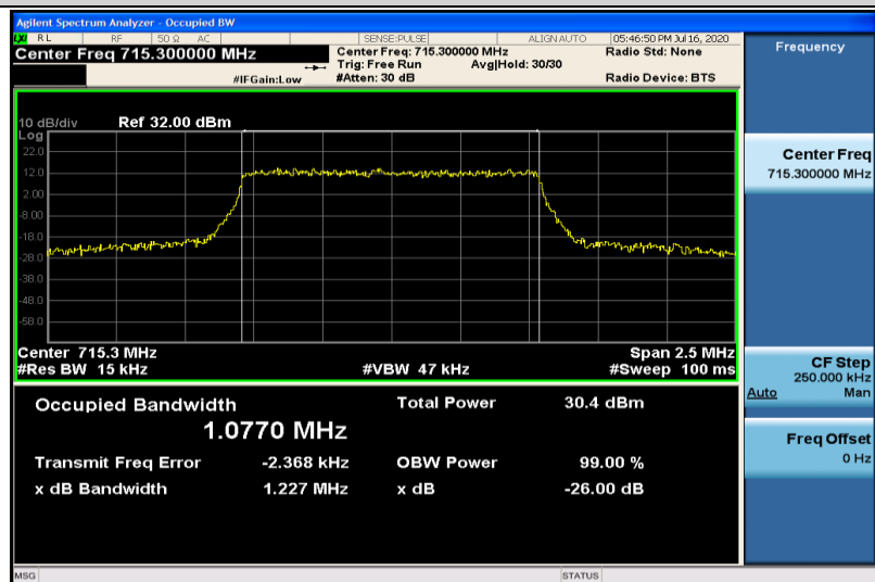
Band12-1.4MHz-QPSK-23173-6RB#0-1.0770
