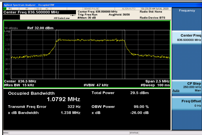
Band5-1.4MHz-16QAM-20525-6RB#0-1.0792
