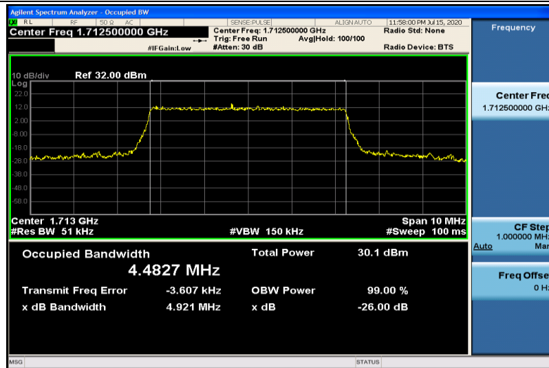
Band4-5MHz-16QAM-19975-25RB#0-4.4827
