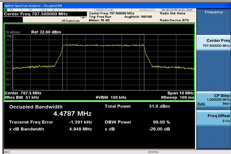
Band12-5MHz-QPSK-23095-25RB#0-4.4787
