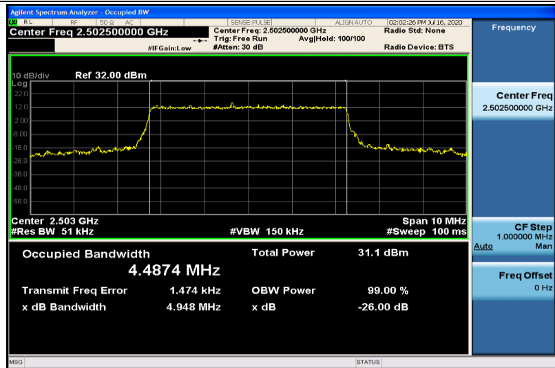
Band7-5MHz-16QAM-20775-25RB#0-4.4874
