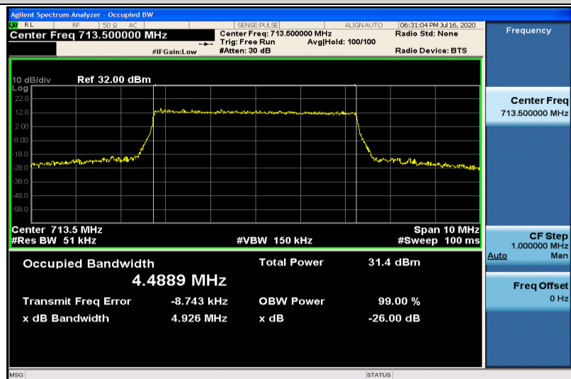
Band12-5MHz-QPSK-23155-25RB#0-4.4889
