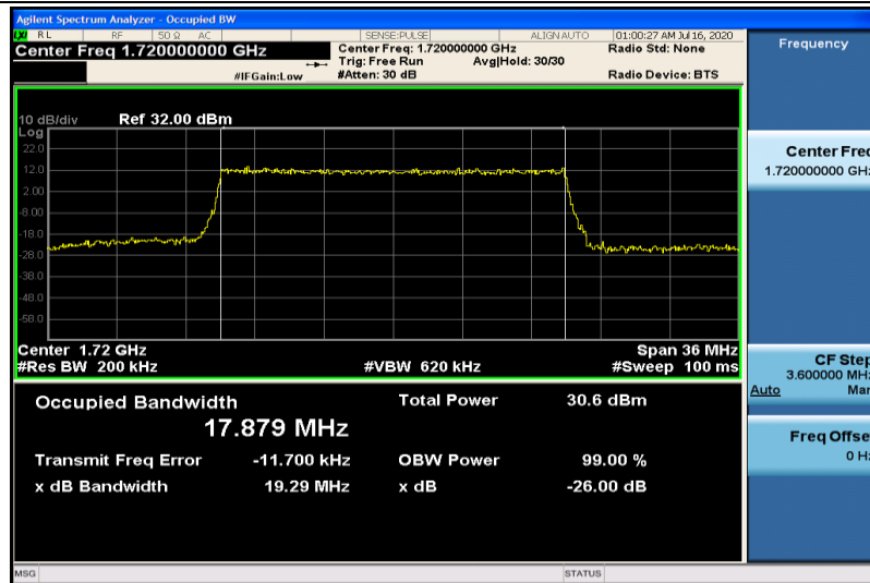
Band4-20MHz-16QAM-20050-100RB#0-17.879
