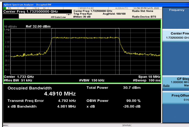
Band4-5MHz-16QAM-20175-25RB#0-4.4910
