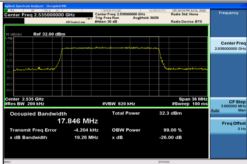
Band7-20MHz-QPSK-21100-100RB#0-17.846
