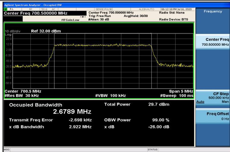
Band12-3MHz-16QAM-23025-15RB#0-2.6789
