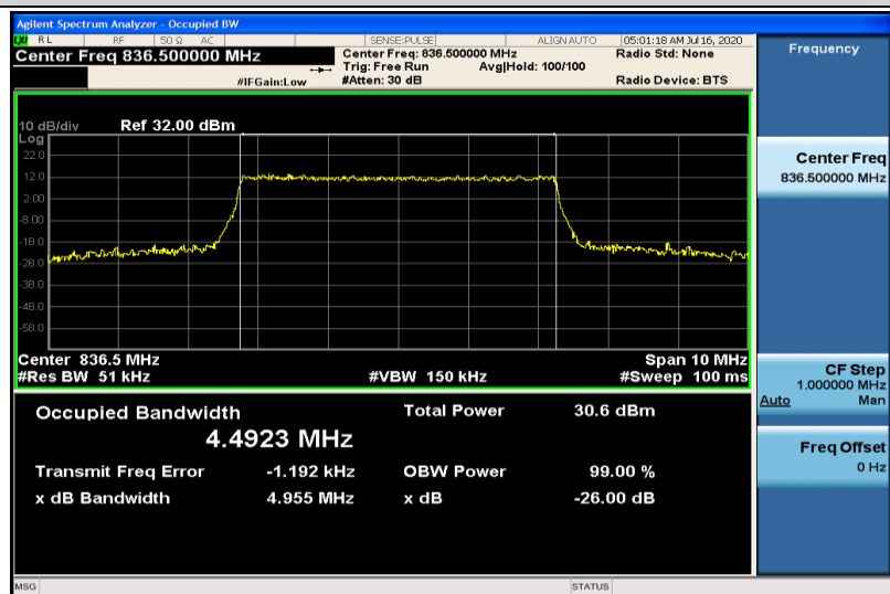
Band5-5MHz-16QAM-20525-25RB#0-4.4923
