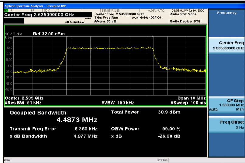
Band7-5MHz-16QAM-21100-25RB#0-4.4873
