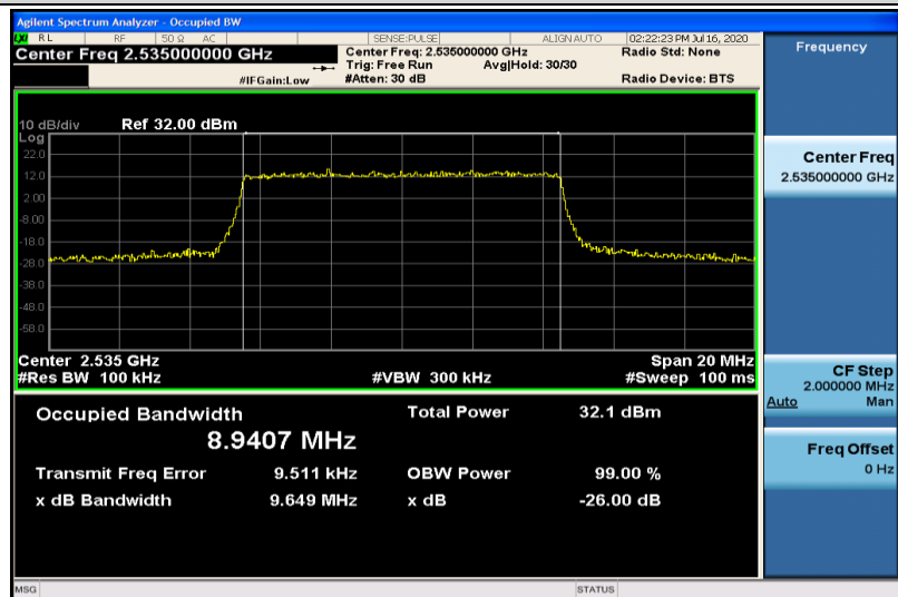
Band7-10MHz-QPSK-21100-50RB#0-8.9407
