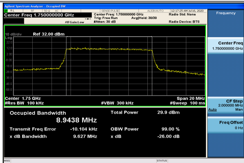
Band4-10MHz-16QAM-20350-50RB#0-8.9438
