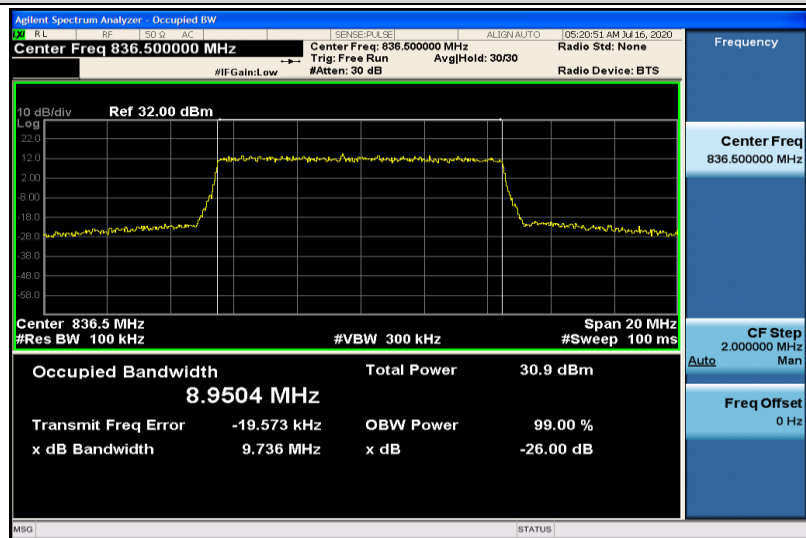
Band5-10MHz-16QAM-20525-50RB#0-8.9504
