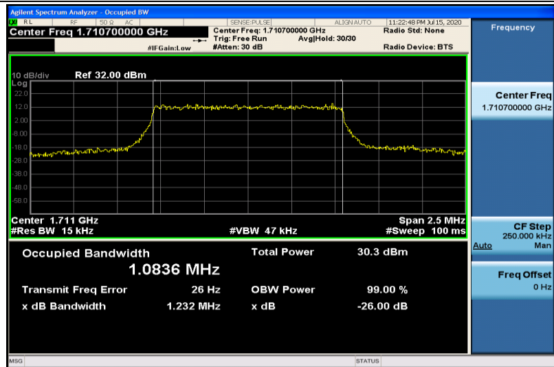
Band4-1.4MHz-QPSK-19957-6RB#0-1.0836
