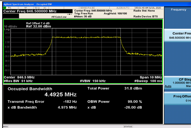
Band5-5MHz-QPSK-20625-25RB#0-4.4925
