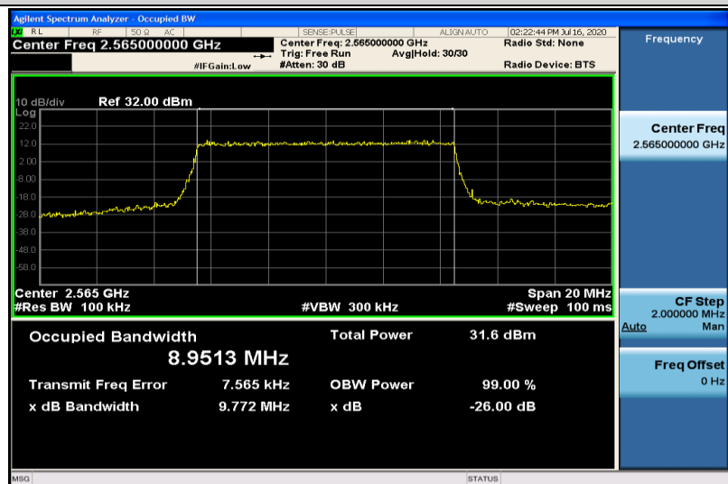
Band7-10MHz-QPSK-21400-50RB#0-8.9513
