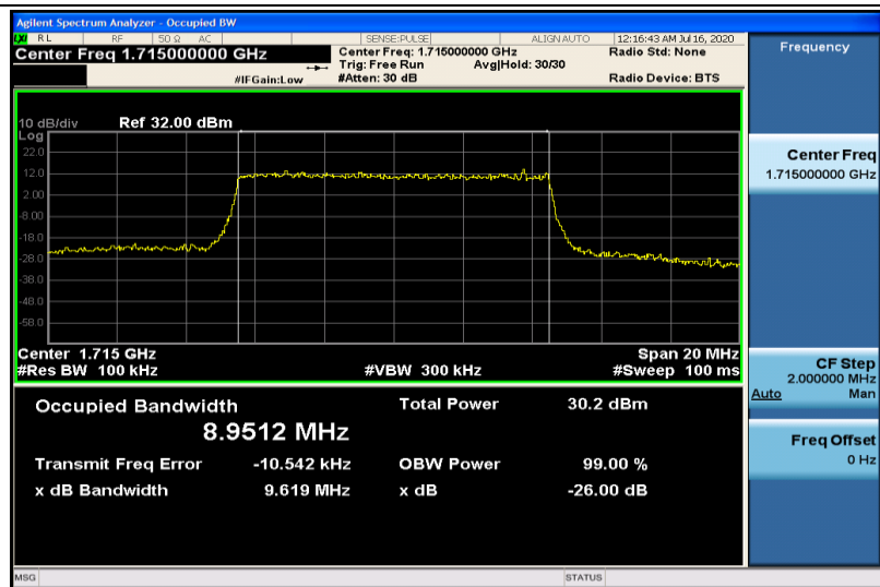
Band4-10MHz-16QAM-20000-50RB#0-8.9512
