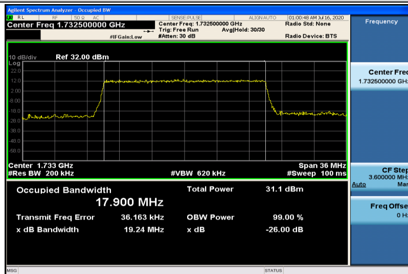
Band4-20MHz-16QAM-20175-100RB#0-17.900
