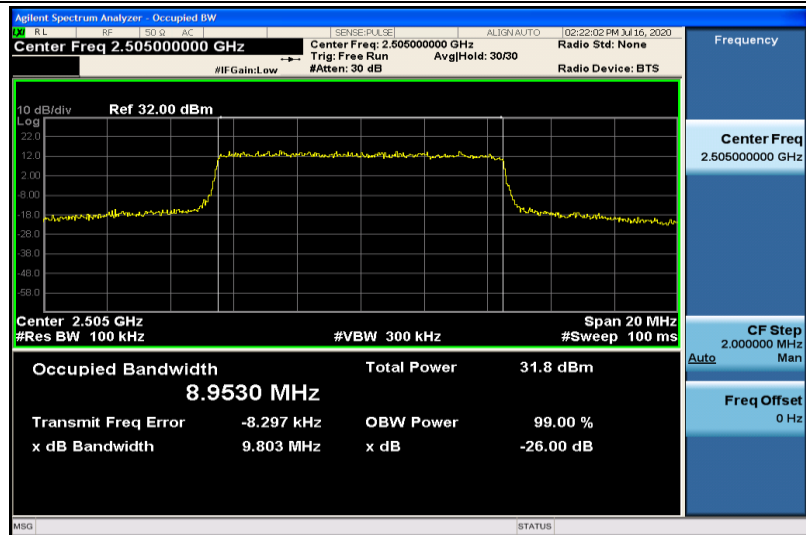
Band7-10MHz-QPSK-20800-50RB#0-8.9530
