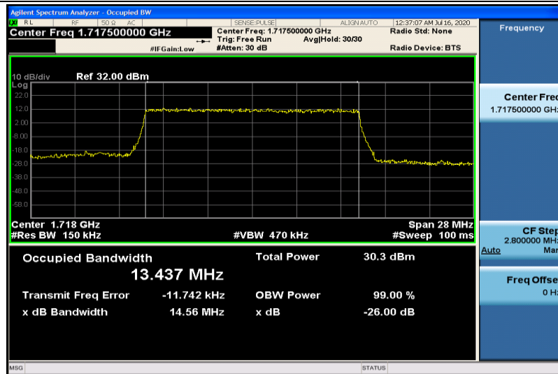
Band4-15MHz-16QAM-20025-75RB#0-13.437
