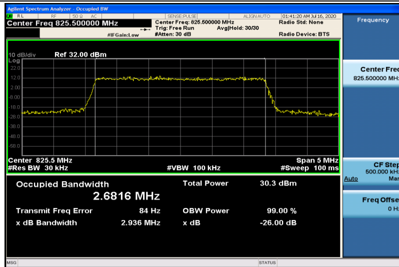
Band5-3MHz-16QAM-20415-15RB#0-2.6816
