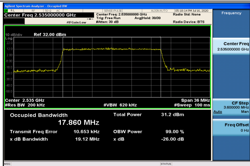
Band7-20MHz-16QAM-21100-100RB#0-17.860
