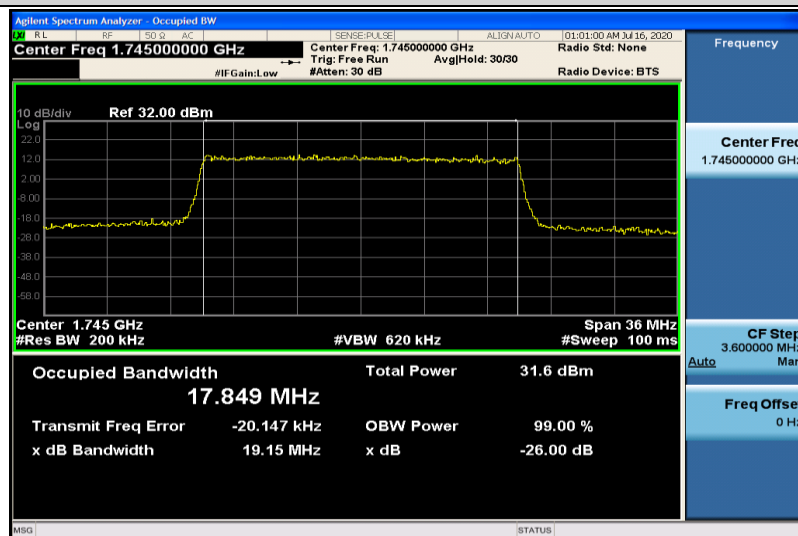
Band4-20MHz-QPSK-20300-100RB#0-17.849
