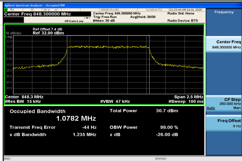
Band5-1.4MHz-QPSK-20643-6RB#0-1.0782
