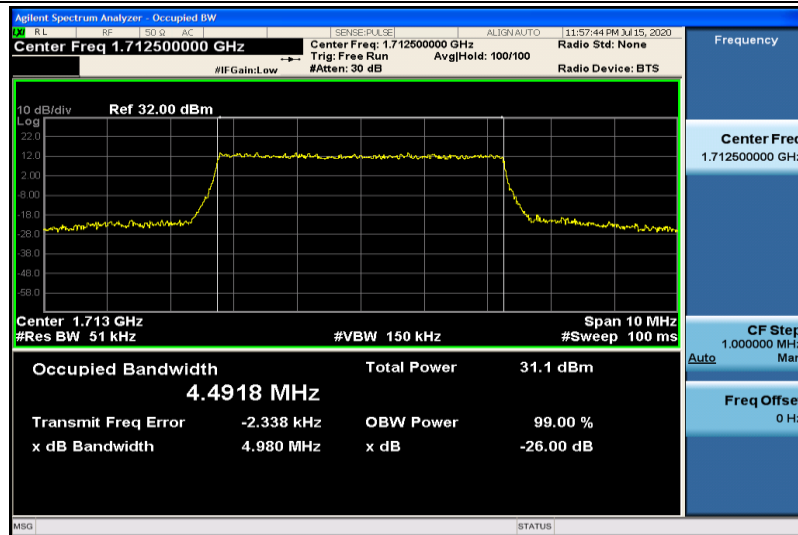
Band4-5MHz-QPSK-19975-25RB#0-4.4918
