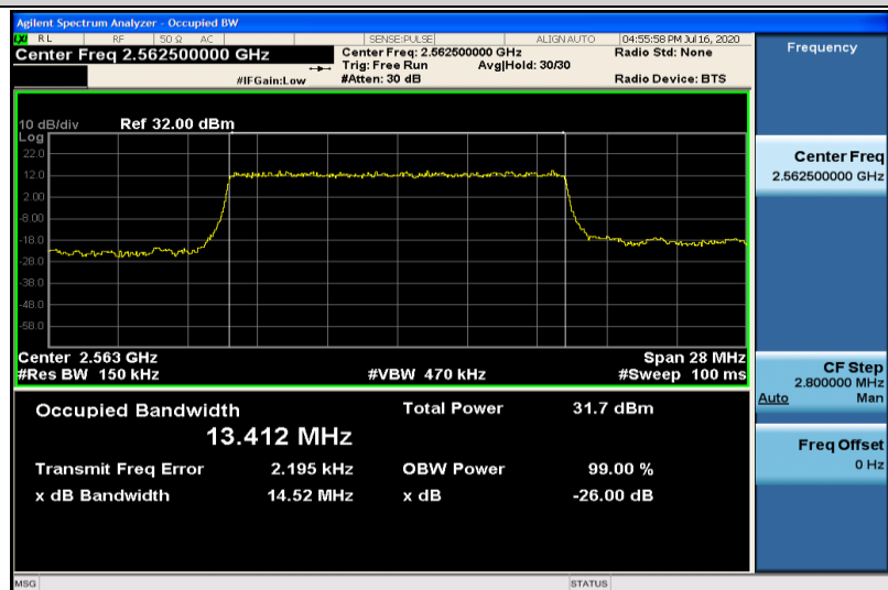
Band7-15MHz-QPSK-21375-75RB#0-13.412
