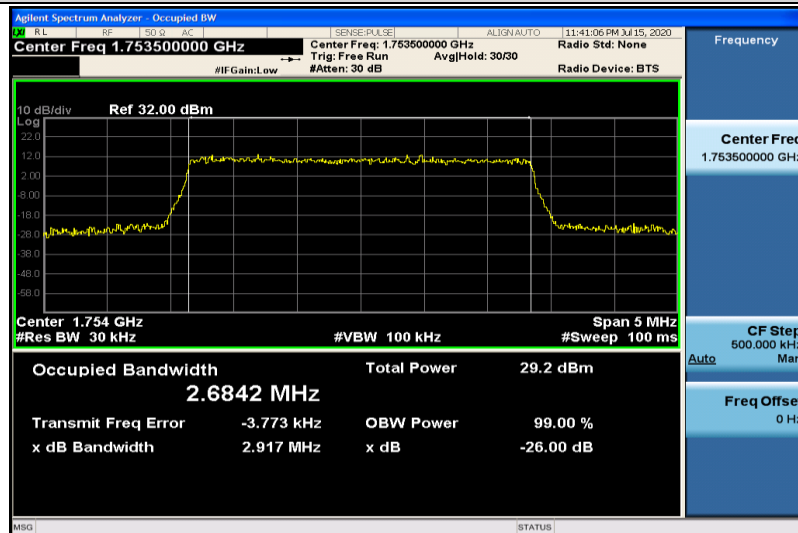
Band4-3MHz-16QAM-20385-15RB#0-2.6842
