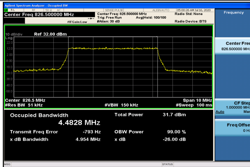
Band5-5MHz-QPSK-20425-25RB#0-4.4828
