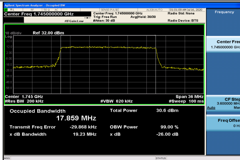
Band4-20MHz-16QAM-20300-100RB#0-17.859
