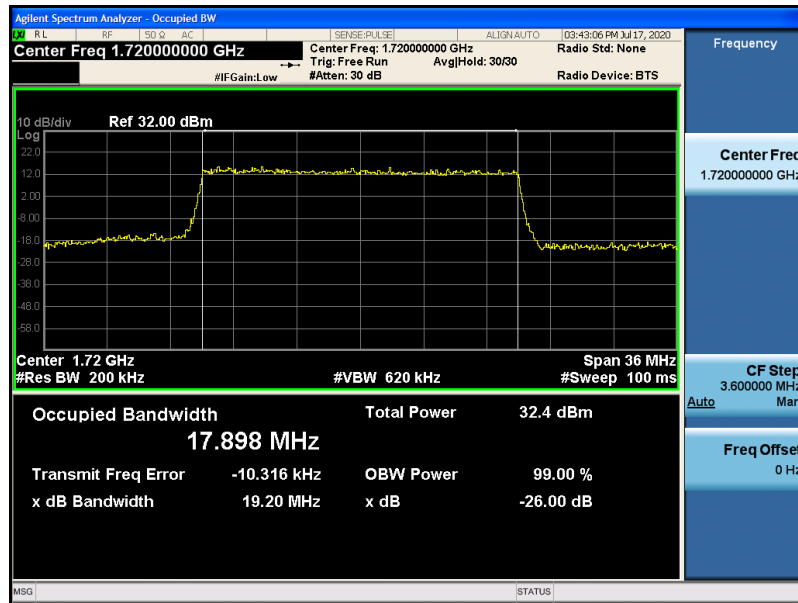
Band4-20MHz-QPSK-20050-100RB#0-17.898
