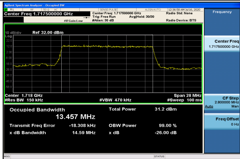
Band4-15MHz-QPSK-20025-75RB#0-13.457
