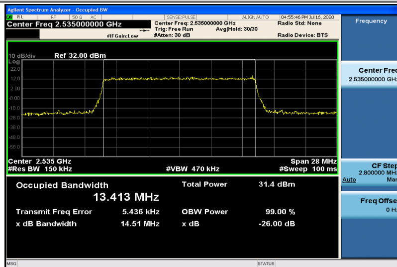
Band7-15MHz-16QAM-21100-75RB#0-13.413
