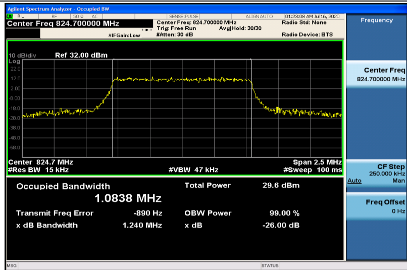
Band5-1.4MHz-16QAM-20407-6RB#0-1.0838
