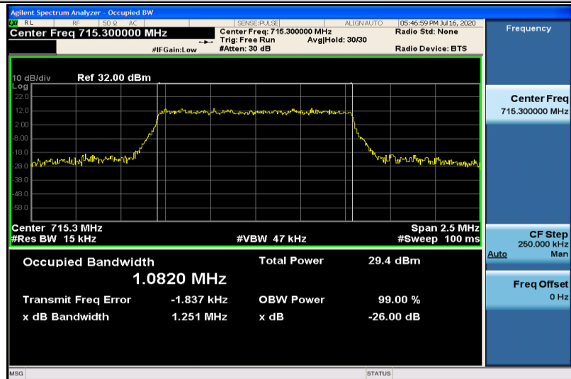
Band12-1.4MHz-16QAM-23173-6RB#0-1.0820
