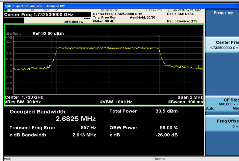
Band4-3MHz-16QAM-20175-15RB#0-2.6825
