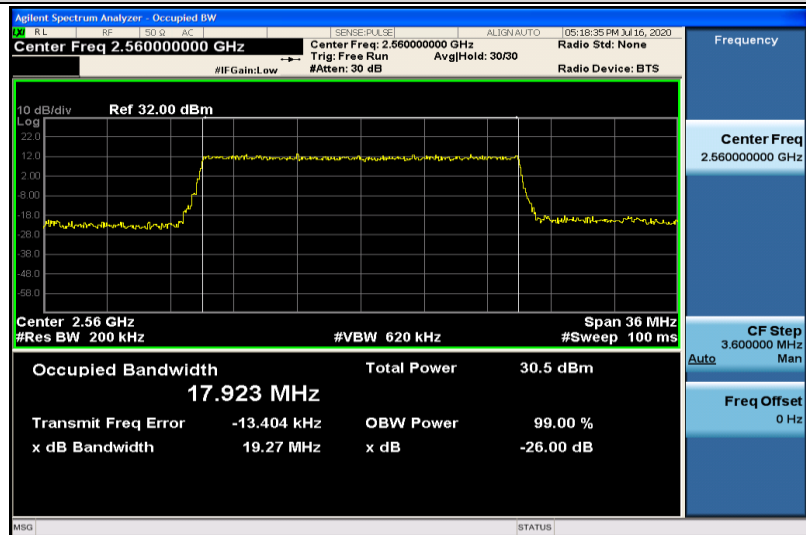
Band7-20MHz-16QAM-21350-100RB#0-17.923
