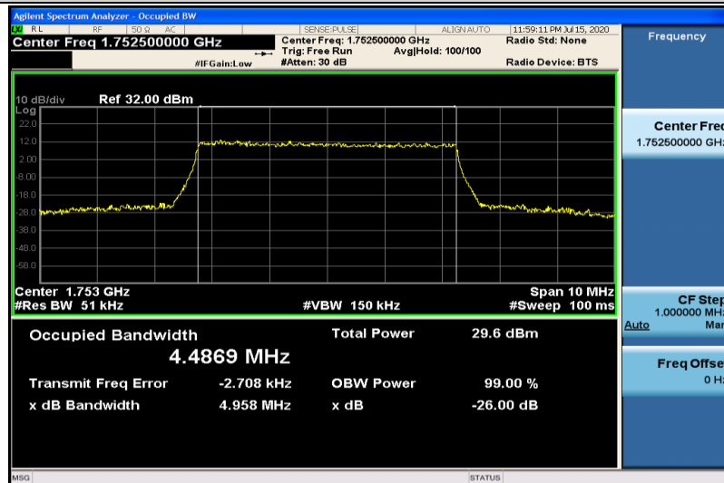
Band4-5MHz-16QAM-20375-25RB#0-4.4869
