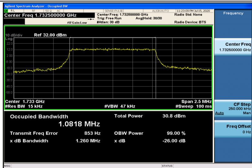
Band4-1.4MHz-QPSK-20175-6RB#0-1.0818
