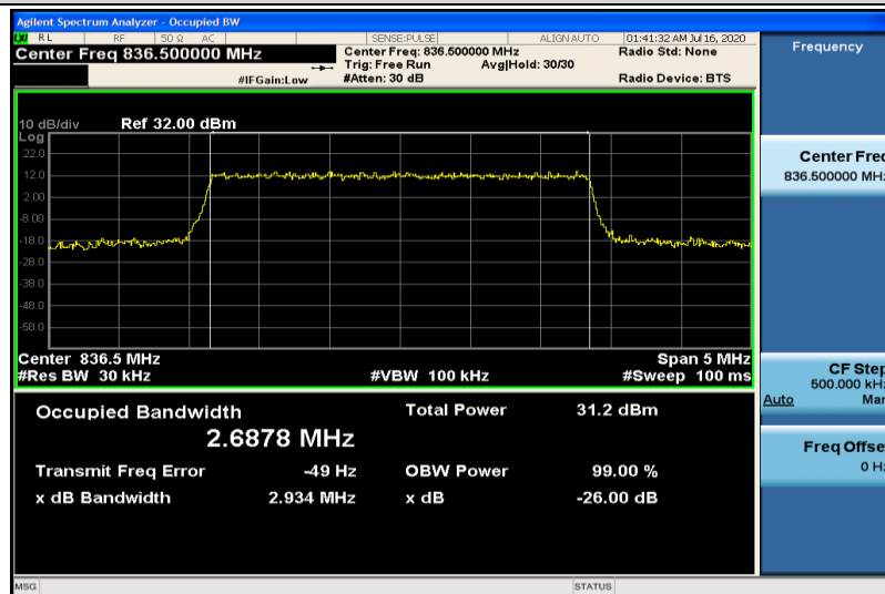
Band5-3MHz-QPSK-20525-15RB#0-2.6878
