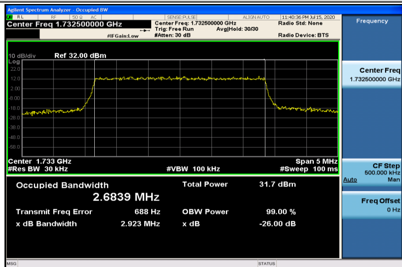
Band4-3MHz-QPSK-20175-15RB#0-2.6839
