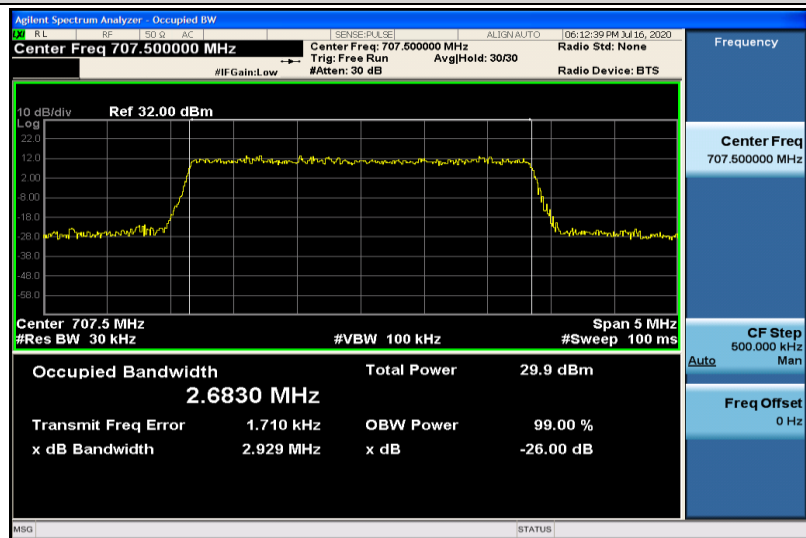
Band12-3MHz-16QAM-23095-15RB#0-2.6830
