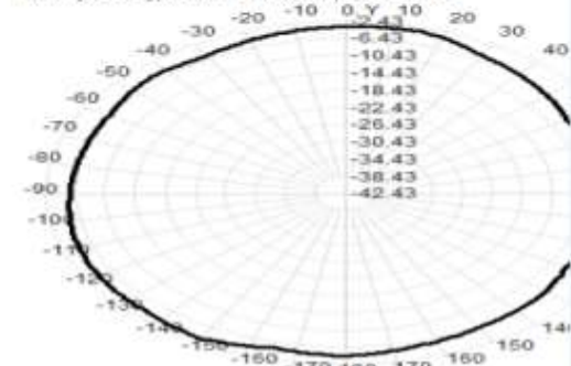
Total(H-XY), Max=-3.50dBi, CirD=4.74
