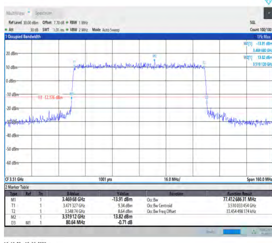
1-N78-3450-3550-PC2-30-80-H-8-CP-64QAM-Outer_Full-217@0-Ant1-77.413-80.640-≤80-PASS
