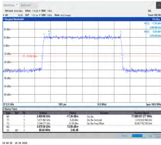
1-N78-3450-3550-PC2-30-80-H-6-CP-QPSK-Outer_Full-217@0-Ant1-77.089-80.640-≤80-PASS
