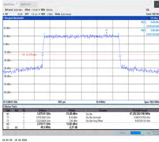
1-N78-3450-3550-PC2-30-50-M-7-CP-16QAM-Outer_Full-133@0-Ant1-47.292-49.300-≤50-PASS
