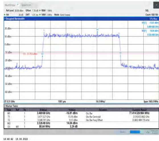
1-N78-3450-3550-PC2-30-80-H-7-CP-16QAM-Outer_Full-217@0-Ant1-77.414-80.640-≤80-PASS
