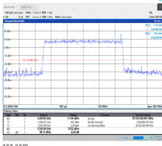
1-N78-3450-3550-PC2-30-90-M-9-CP-256QAM-Outer_Full-245@0-Ant1-87.074-90.720-≤90-PASS
