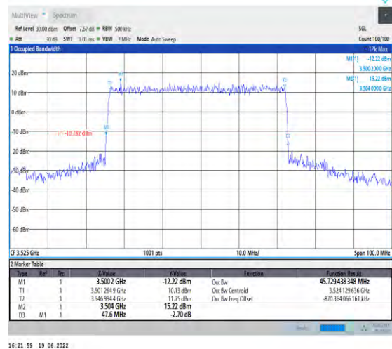
1-N78-3450-3550-PC2-30-50-H-1-DFT-QPSK-Outer_Full-128@0-Ant1-45.729-47.600-≤50-PASS
