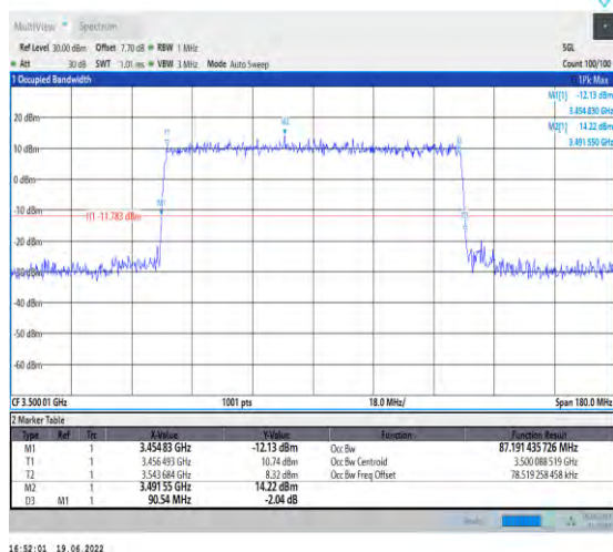
1-N78-3450-3550-PC2-30-90-M-8-CP-64QAM-Outer_Full-245@0-Ant1-87.191-90.540-≤90-PASS
