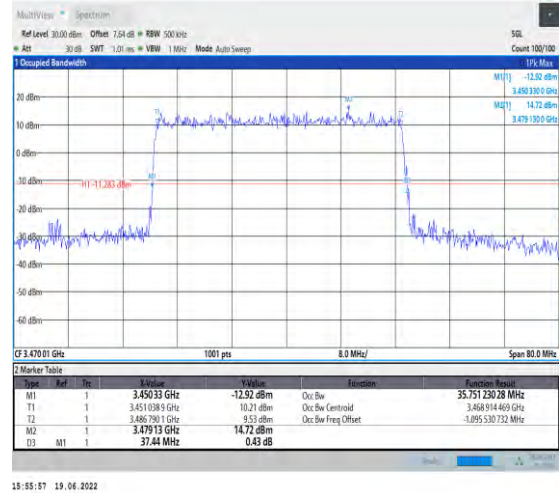
1-N78-3450-3550-PC2-30-40-L-4-DFT-64QAM-Outer_Full-100@0-Ant1-35.751-37.440-≤40-PASS
