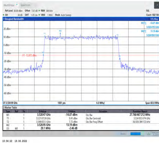
1-N78-3450-3550-PC2-30-30-H-8-CP-64QAM-Outer_Full-78@0-Ant1-27.76-29.100-≤30-PASS
