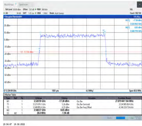
1-N78-3450-3550-PC2-30-30-H-9-CP-256QAM-Outer_Full-78@0-Ant1-27.819-28.800-≤30-PASS
