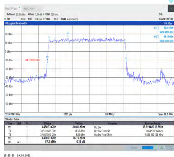
1-N78-3450-3550-PC2-30-40-L-2-DFT-PI2BPSK-Outer_Full-100@0-Ant1-35.62-37.200-≤40-PASS
