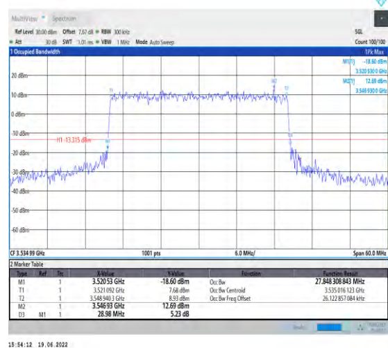
1-N78-3450-3550-PC2-30-30-H-7-CP-16QAM-Outer_Full-78@0-Ant1-27.848-28.980-≤30-PASS
