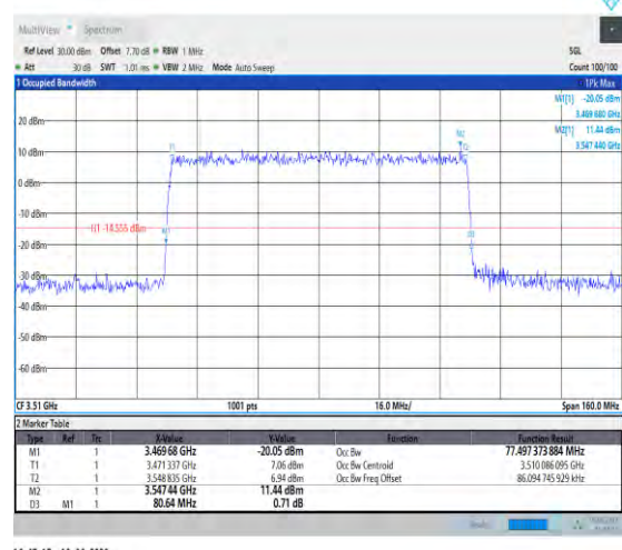
1-N78-3450-3550-PC2-30-80-H-9-CP-256QAM-Outer_Full-217@0-Ant1-77.497-80.640-≤80-PASS
