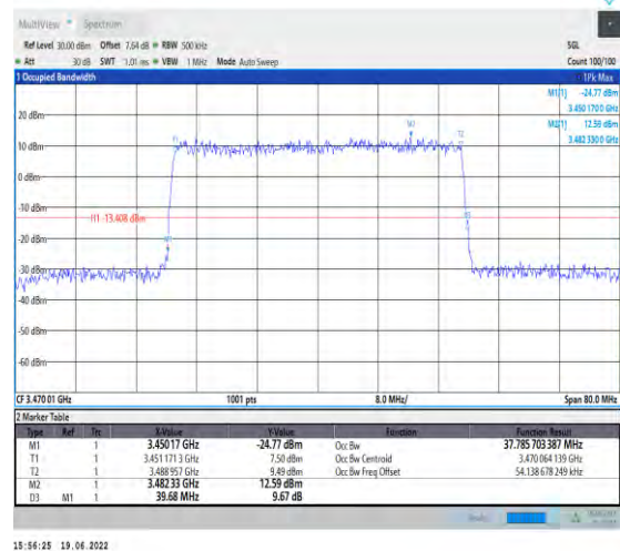
1-N78-3450-3550-PC2-30-40-L-6-CP-QPSK-Outer_Full-106@0-Ant1-37.786-39.680-≤40-PASS
