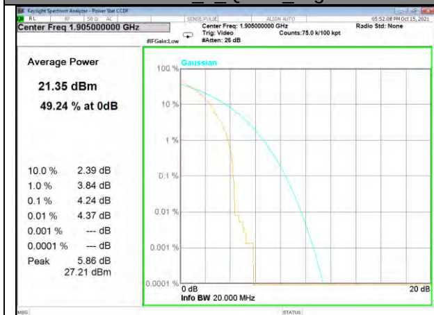
Band 25_1_Q16_High
