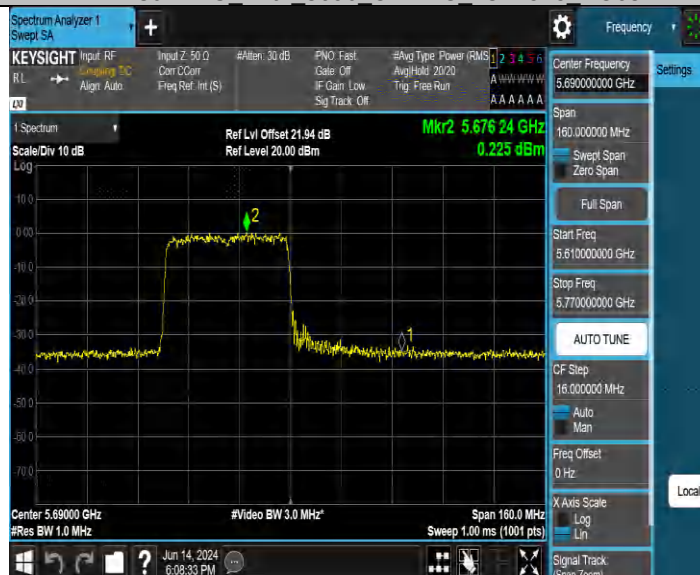
11BE80MIMO Ant1 5690 UNII-3 26Tone RU0
