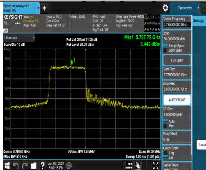
11BE40MIMO Ant4 5795 26Tone RU00
