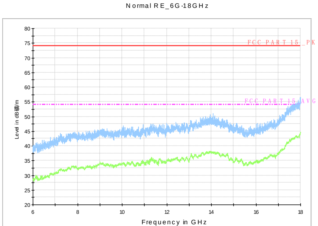
Fig. 69 Radiated Spurious Emission (802.11a, ch100, 6 GHz-18 GHz)
