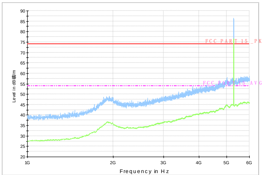
Fig. 62 Radiated Spurious Emission (802.11a, ch56, 1 GHz-6 GHz)
