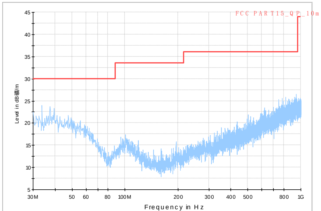
Fig. 61 Radiated Spurious Emission (802.11a, ch56, 30 MHz-1 GHz)
