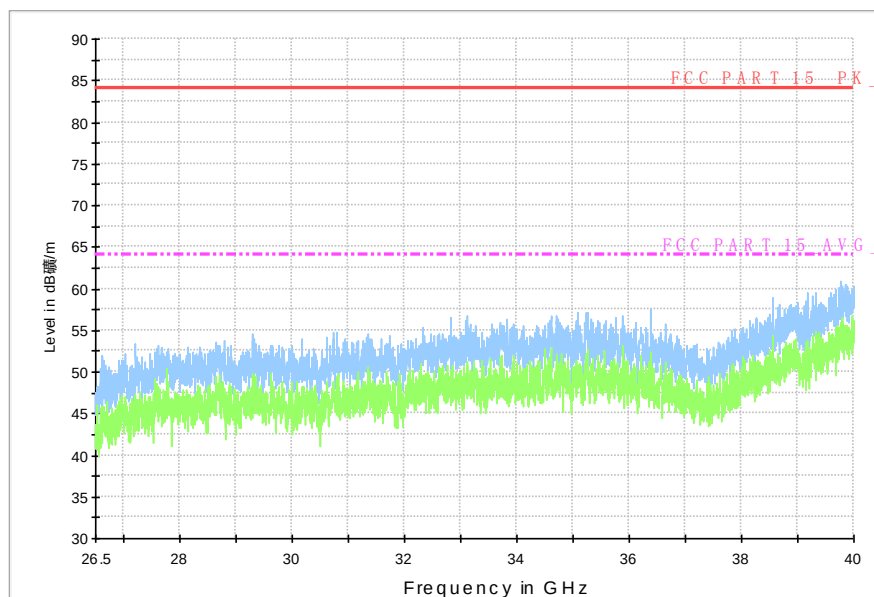
Normal RE_26.5G-40GHz
