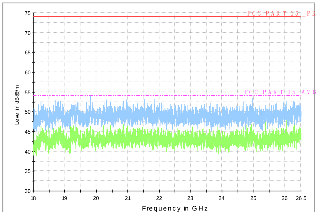
Normal RE_18G-26.5GHz
