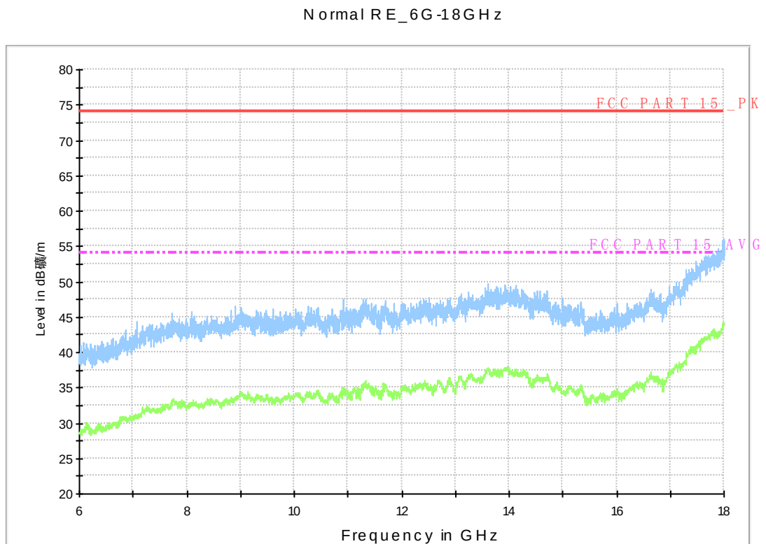
Fig. 54 Radiated Spurious Emission (802.11a, ch40, 6 GHz-18 GHz)
