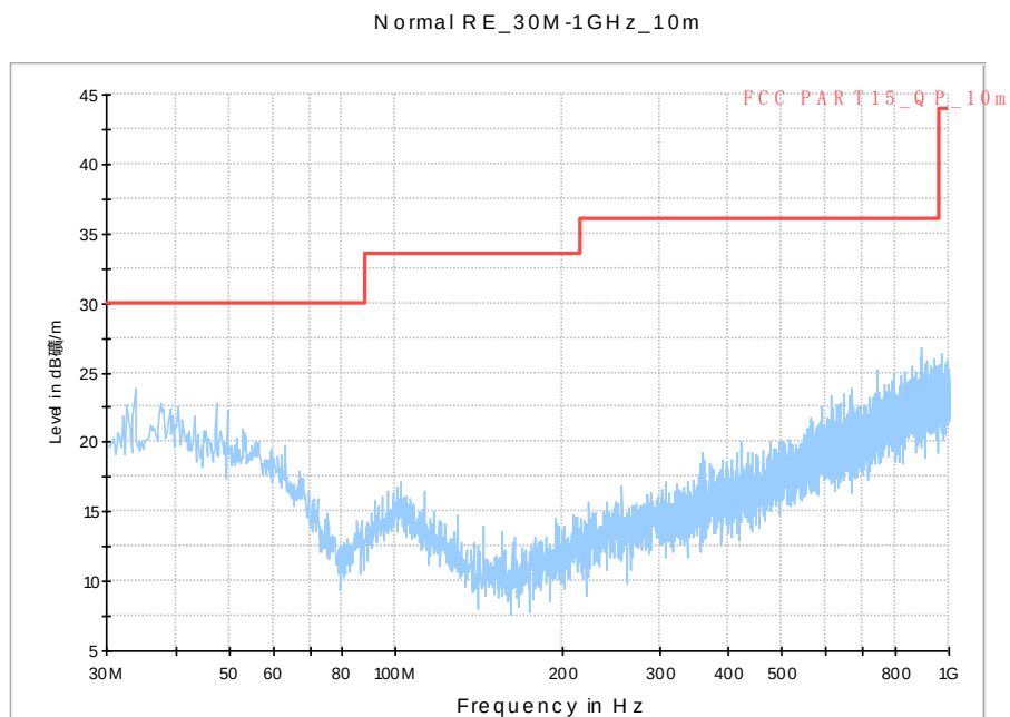
Fig. 52 Radiated Spurious Emission (802.11a, ch40, 30 MHz-1 GHz)
