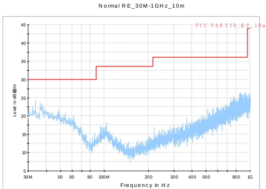
Fig. 79 Radiated Spurious Emission (802.11n-HT20, ch40, 30 MHz-1 GHz)
