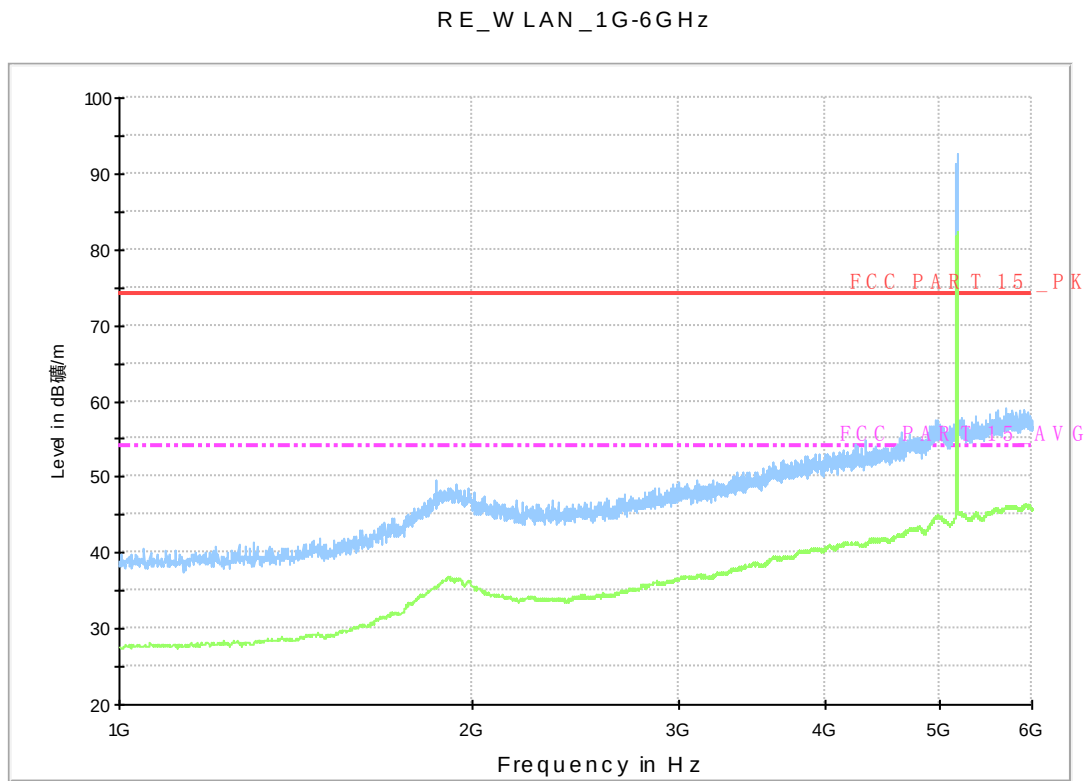
Fig. 50 Radiated Spurious Emission (802.11a, ch36, 1 GHz-6 GHz)
