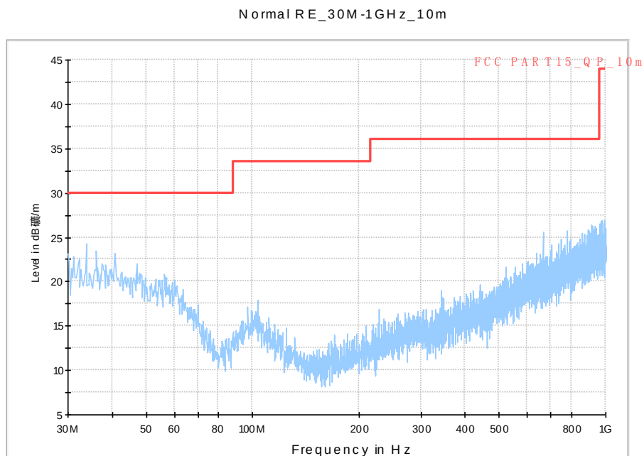
Fig. 70 Radiated Spurious Emission (802.11a, ch120, 30 MHz-1 GHz)
