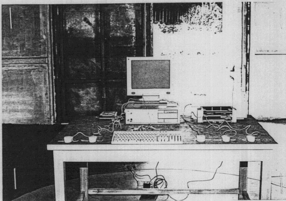
Radiated Emission, Rear View
