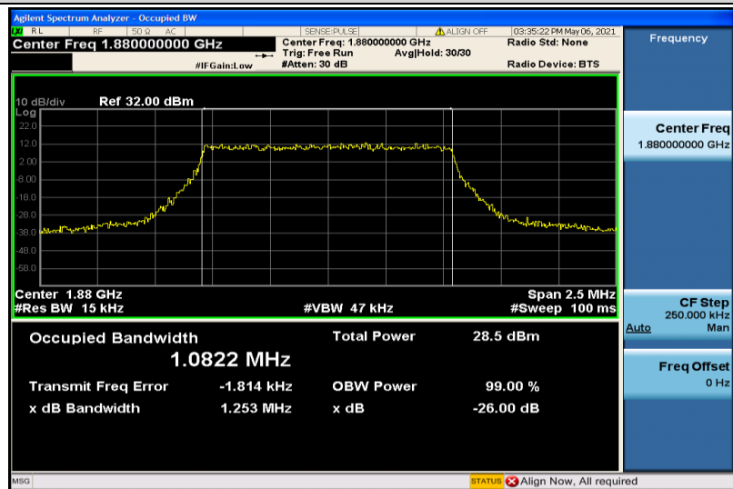
Band2-1.4MHz-16QAM-18900-6RB#0-1.0822
