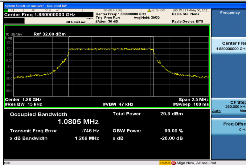
Band2-1.4MHz-QPSK-18900-6RB#0-1.0805
