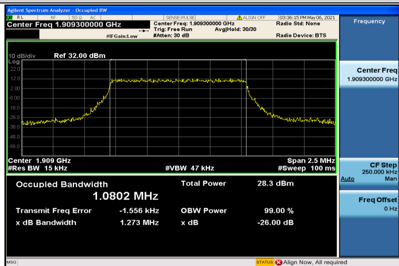
Band2-1.4MHz-16QAM-19193-6RB#0-1.0802
