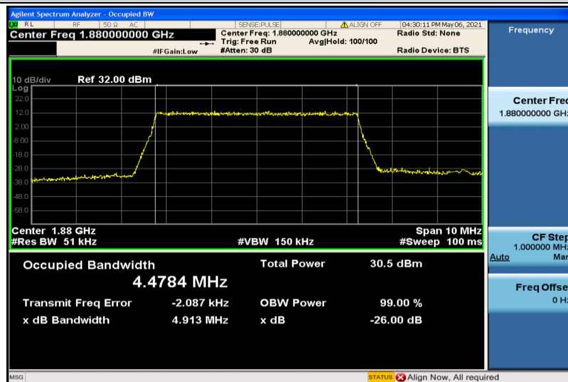
Band2-5MHz-QPSK-18900-25RB#0-4.4784
