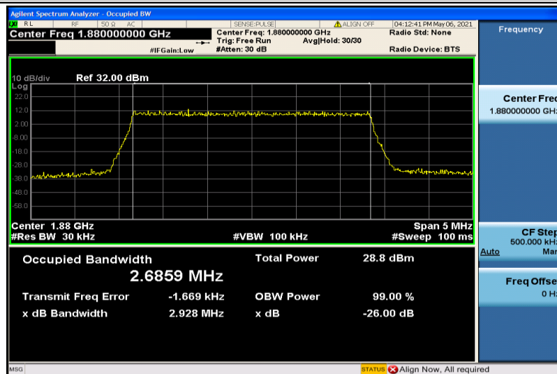
Band2-3MHz-16QAM-18900-15RB#0-2.6859
