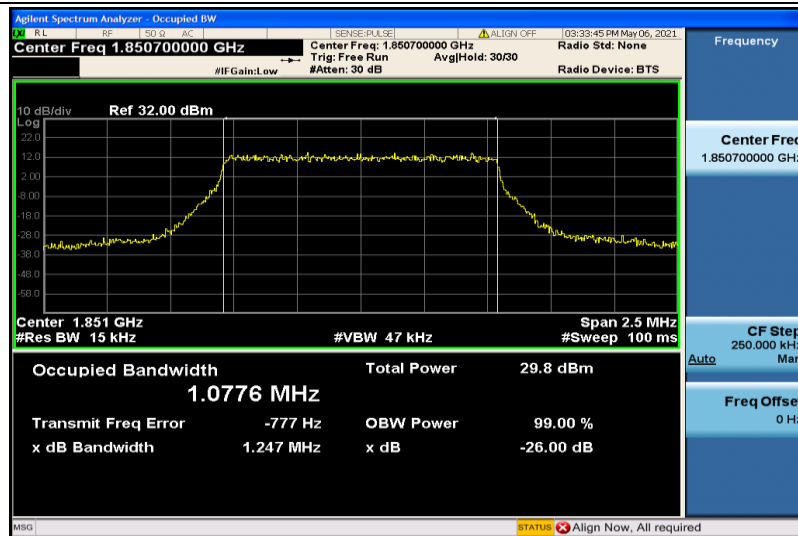
Band2-1.4MHz-QPSK-18607-6RB#0-1.0776
