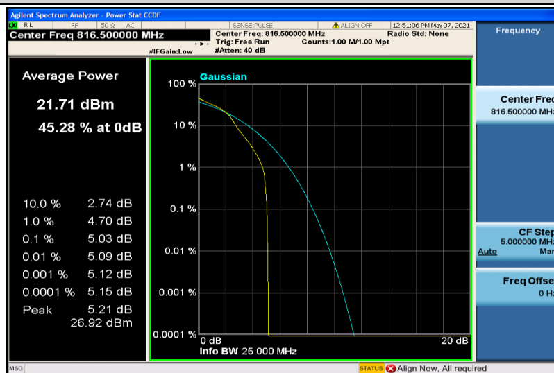
Band26-5MHz-16QAM-26715-1RB#0
