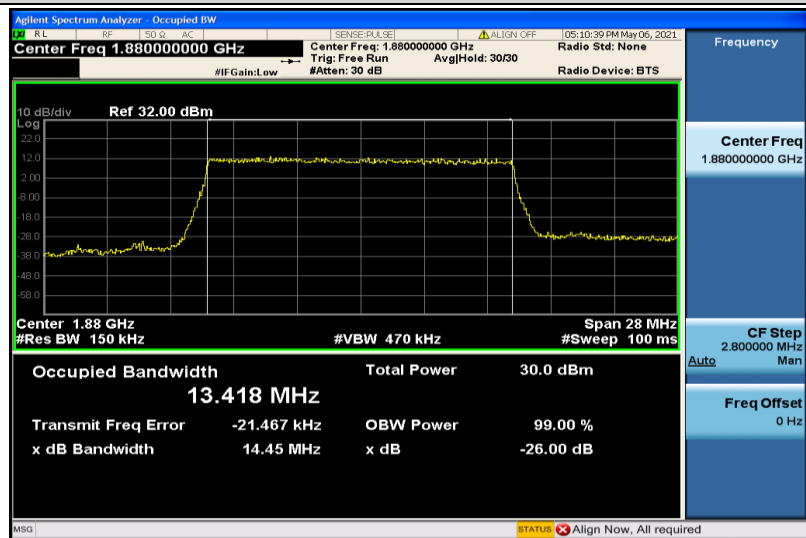
Band2-15MHz-16QAM-18900-75RB#0-13.418
