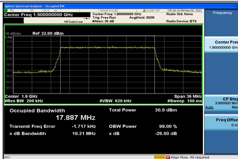
Band2-20MHz-QPSK-19100-100RB#0-17.887
