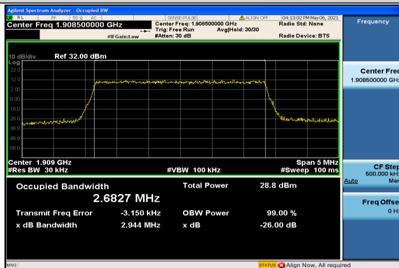
Band2-3MHz-16QAM-19185-15RB#0-2.6827
