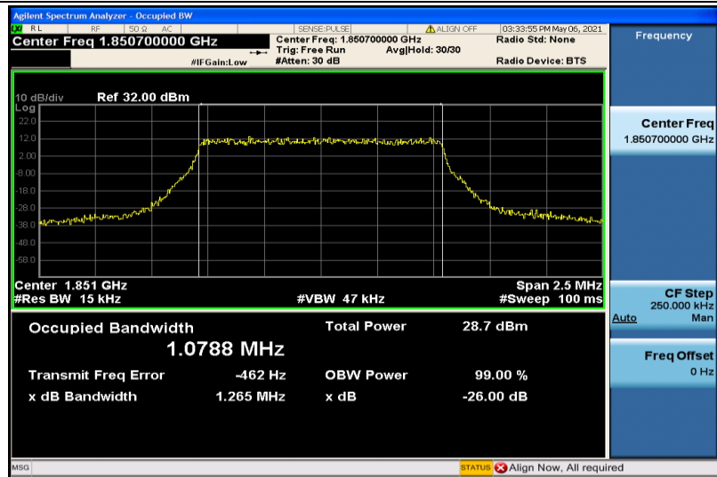
Band2-1.4MHz-16QAM-18607-6RB#0-1.0788
