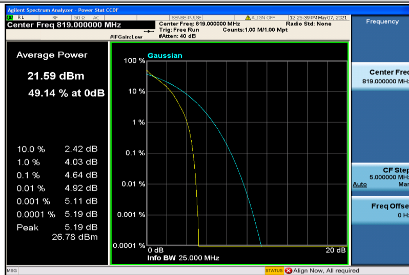
Band26-1.4MHz-QPSK-26740-6RB#0
