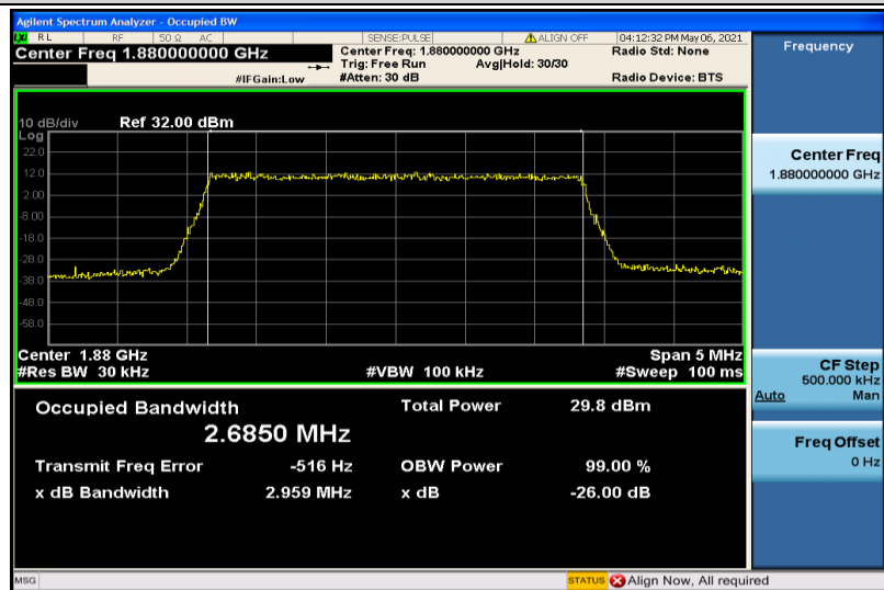
Band2-3MHz-QPSK-18900-15RB#0-2.6850
