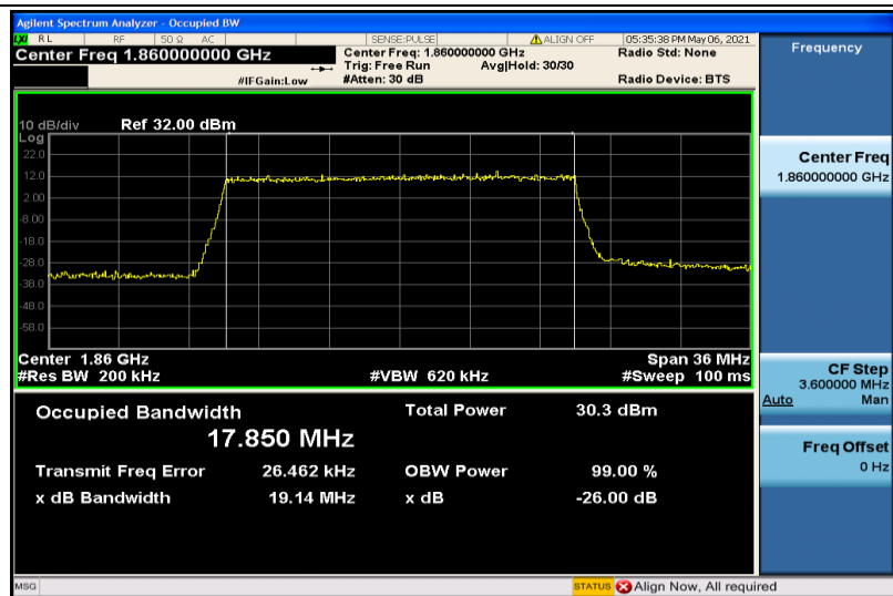
Band2-20MHz-16QAM-18700-100RB#0-17.850
