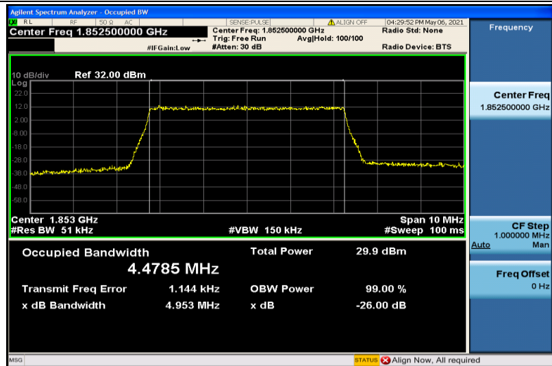
Band2-5MHz-16QAM-18625-25RB#0-4.4785
