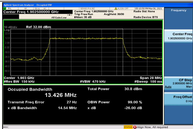
Band2-15MHz-QPSK-19125-75RB#0-13.426
