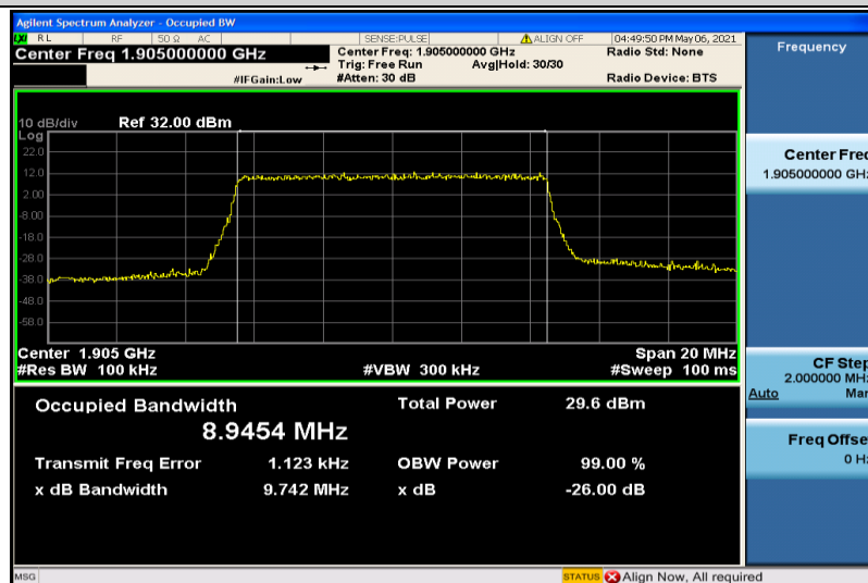
Band2-10MHz-16QAM-19150-50RB#0-8.9454
