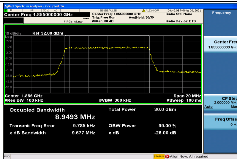
Band2-10MHz-16QAM-18650-50RB#0-8.9493
