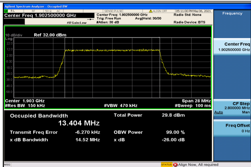
Band2-15MHz-16QAM-19125-75RB#0-13.404
