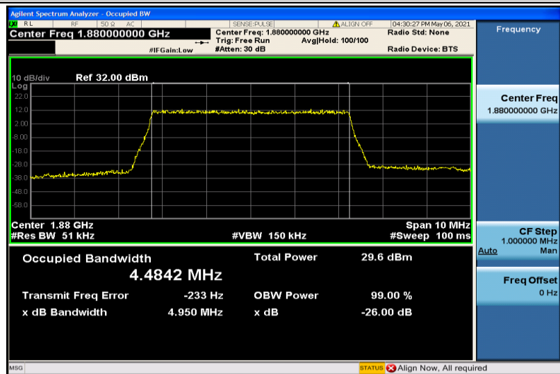
Band2-5MHz-16QAM-18900-25RB#0-4.4842
