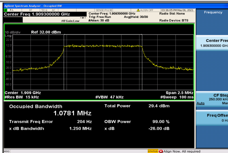
Band2-1.4MHz-QPSK-19193-6RB#0-1.0781
