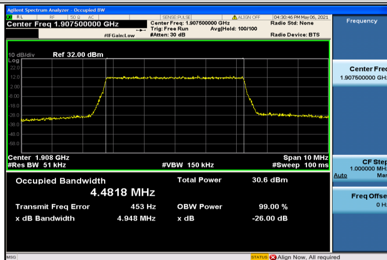
Band2-5MHz-QPSK-19175-25RB#0-4.4818
