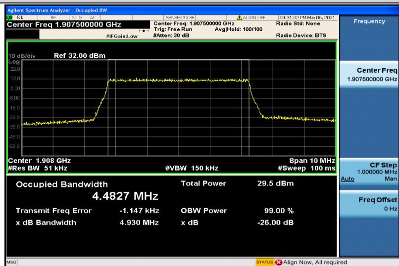
Band2-5MHz-16QAM-19175-25RB#0-4.4827
