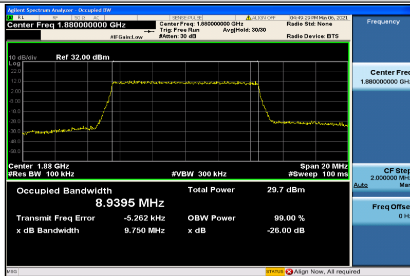
Band2-10MHz-16QAM-18900-50RB#0-8.9395
