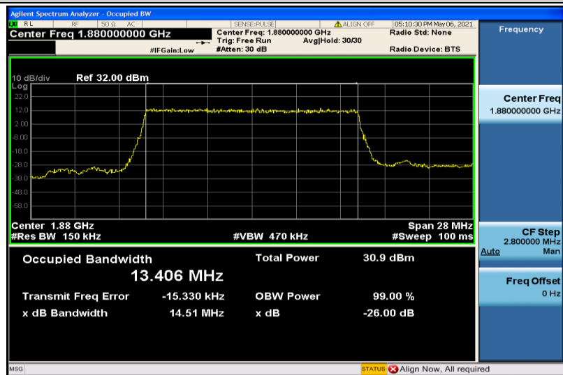
Band2-15MHz-QPSK-18900-75RB#0-13.406
