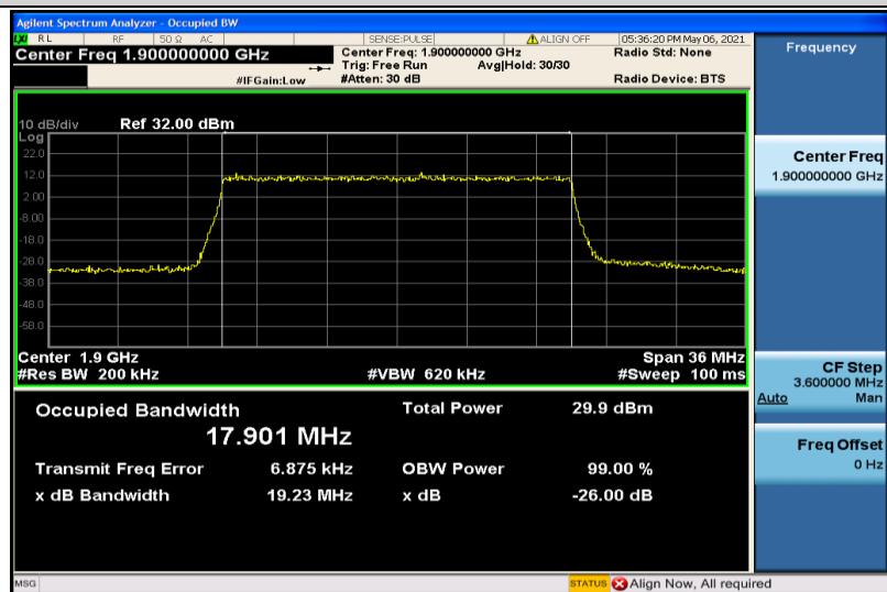
Band2-20MHz-16QAM-19100-100RB#0-17.901
