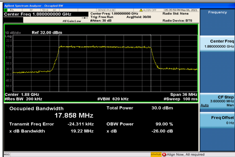
Band2-20MHz-16QAM-18900-100RB#0-17.858
