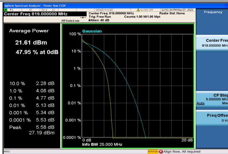
Band26-5MHz-QPSK-26740-25RB#0
