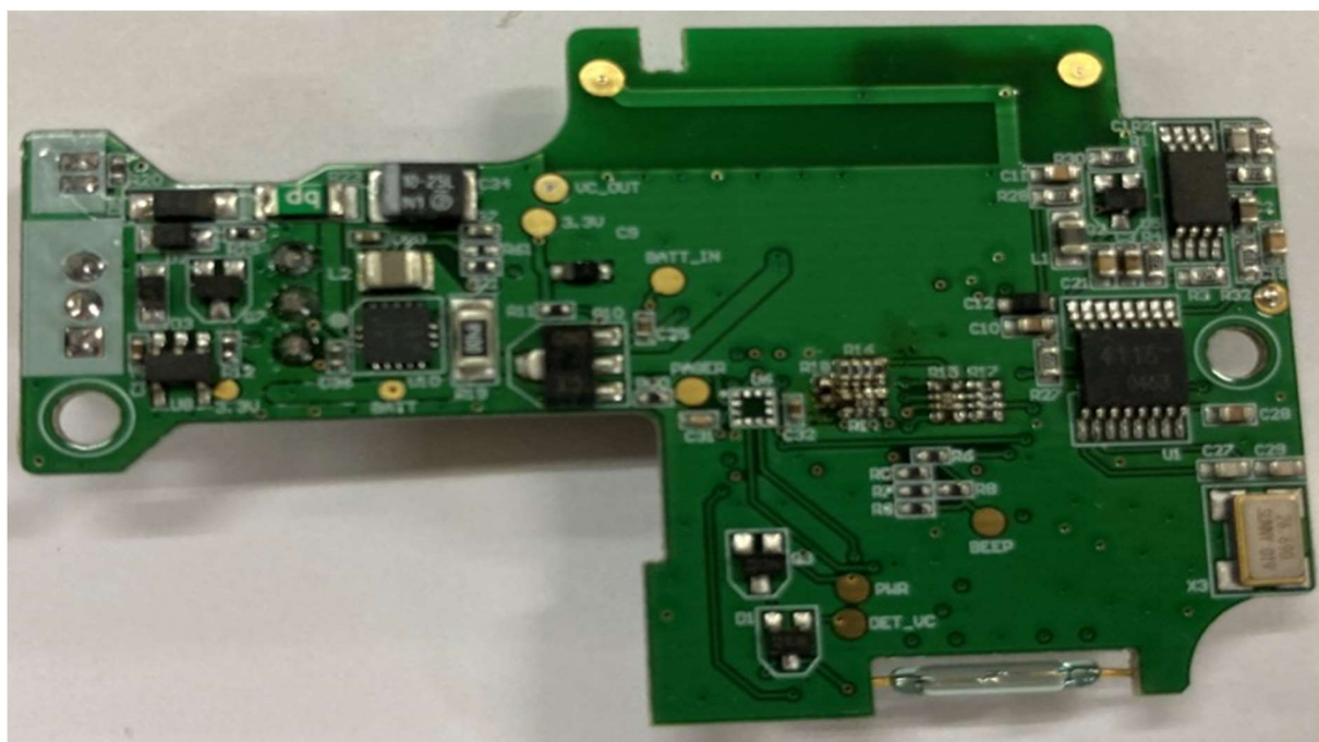
Bottom view of Main PCB
