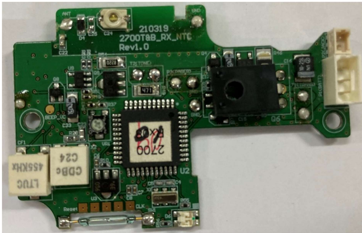
Bottom view of Main PCB
