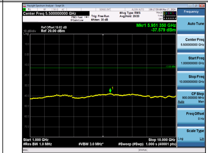
Band12_10MHz_QPSK_23095_1RB#0_1000~10000_1000~1000
