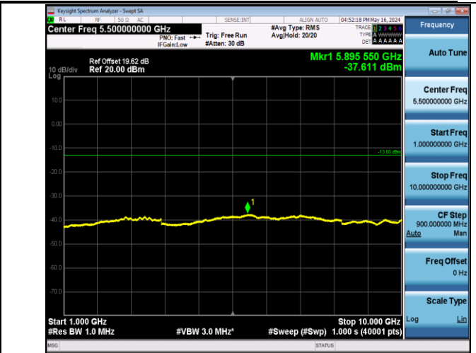
Band5_1.4MHz_QPSK_20407_1RB#0_1000~10000_1000~10000
