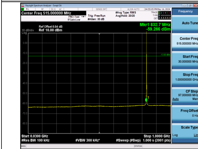
Band5_1.4MHz_16QAM_20525_1RB#0_30~1000_30~1000
