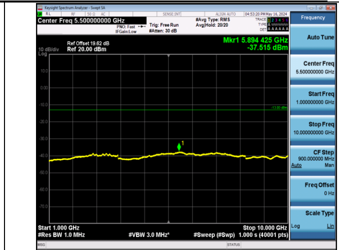
Band5_1.4MHz_16QAM_20407_1RB#0_1000~10000_1000~1000
