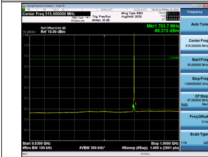
Band12_1.4MHz_QPSK_23095_1RB#0_30~1000_30~1000
