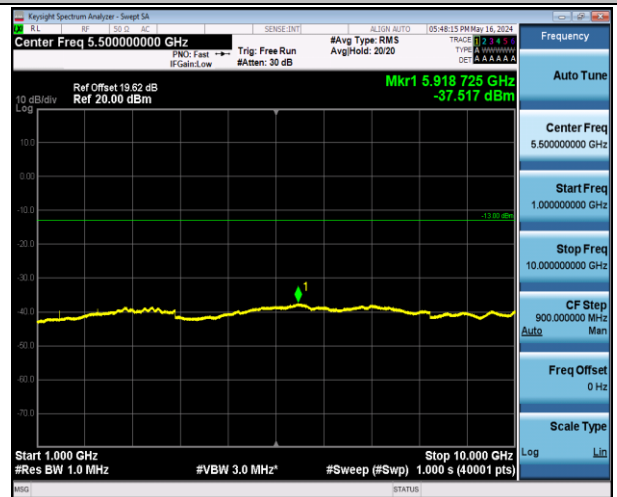
Band12_1.4MHz_16QAM_23173_1RB#0_1000~10000_1000~100 00
