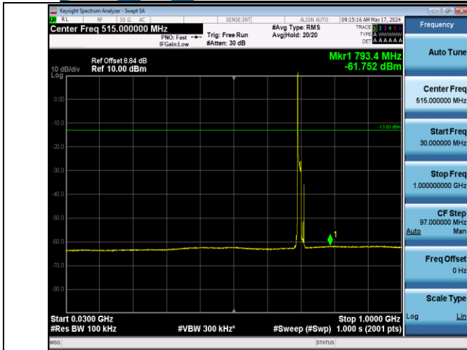
Band12_10MHz_QPSK_23060_1RB#0_30~1000_30~1000
