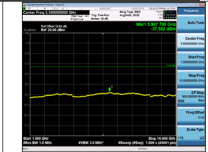
Band12_1.4MHz_QPSK_23017_1RB#0_1000~10000_1000~1000
