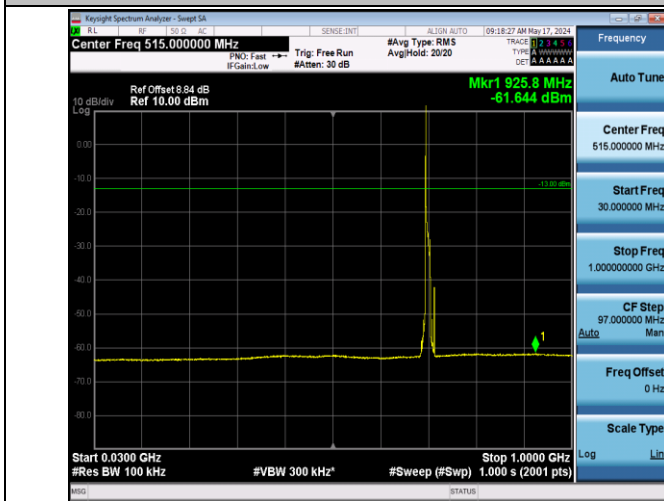
Band12_10MHz_16QAM_23095_1RB#0_30-1000_30-1000
