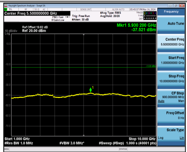
Band12_1.4MHz_16QAM_23095_1RB#0_1000~10000_1000~100 00
