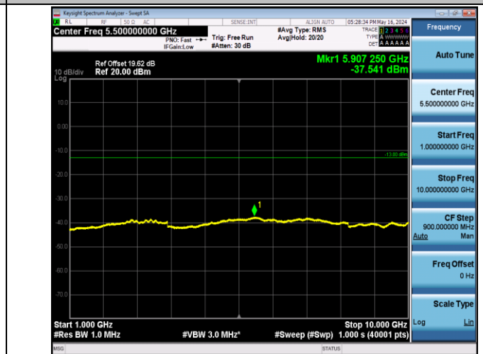
Band5_10MHz_16QAM_20600_1RB#0_1000~10000_1000~1000
