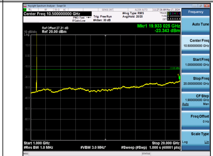
Band66_20MHz_QPSK_132572_1RB#0_1000-20000_1000-2000
