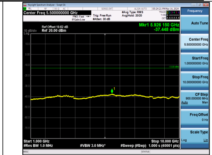
Band5_10MHz_16QAM_20450_1RB#0_1000~10000_1000~1000
