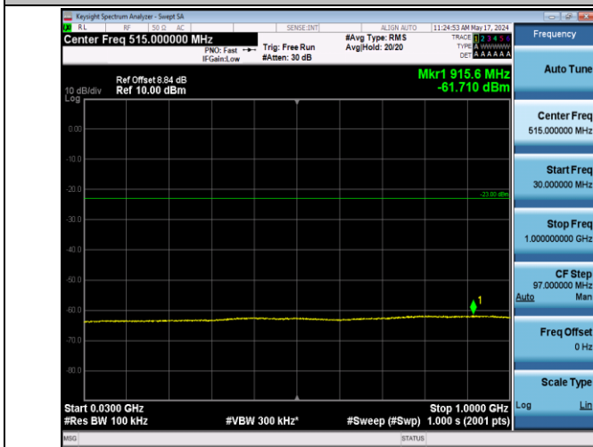
Band66_20MHz_QPSK_132322_1RB#0_30-1000_30-1000
