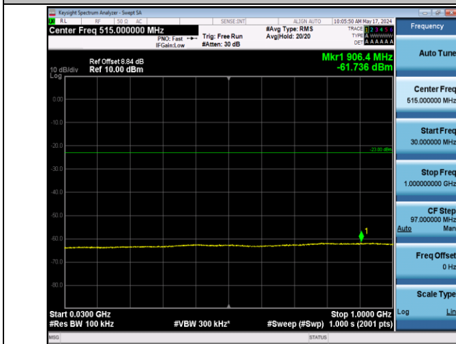
Band66_1.4MHz_QPSK_132322_1RB#0_30~1000_30~1000
