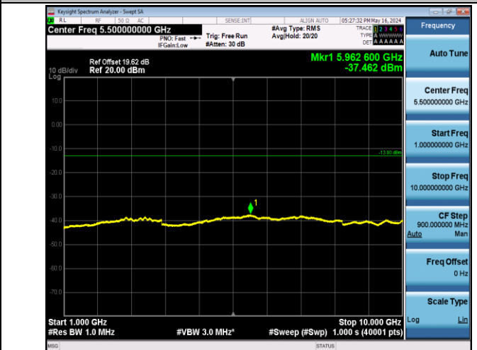
Band5_10MHz_QPSK_20600_1RB#0_1000~10000_1000~10000
