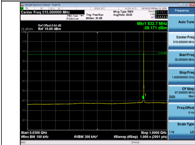
Band5_1.4MHz_QPSK_20525_1RB#0_30~1000_30~1000
