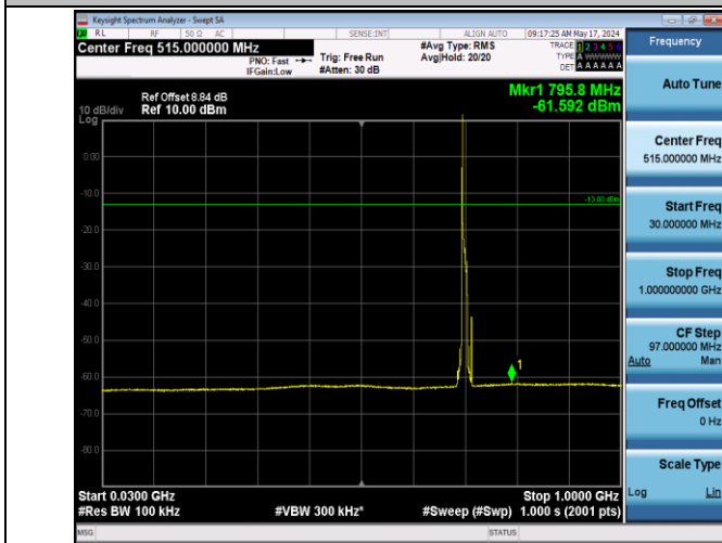
Band12_10MHz_QPSK_23095_1RB#0_30~1000_30~1000
