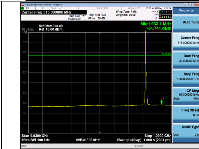
Band5_10MHz_QPSK_20450_1RB#0_30~1000_30~1000
