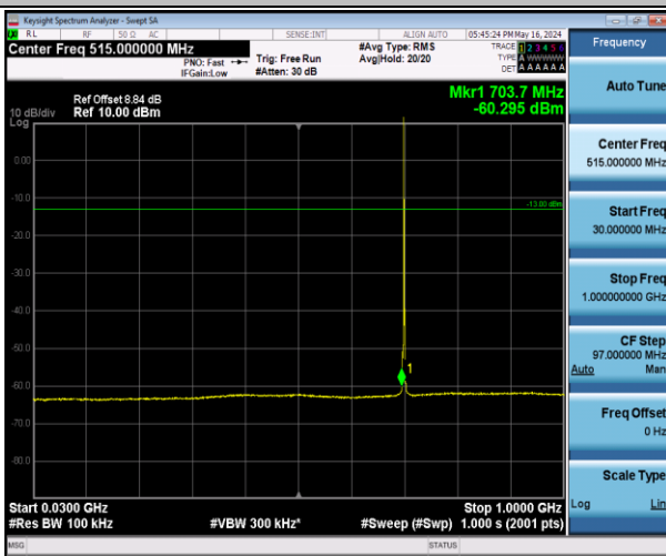
Band12_1.4MHz_16QAM_23095_1RB#0_30~1000_30~1000
