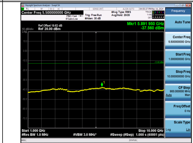
Band5_1.4MHz_16QAM_20525_1RB#0_1000~10000_1000~1000
