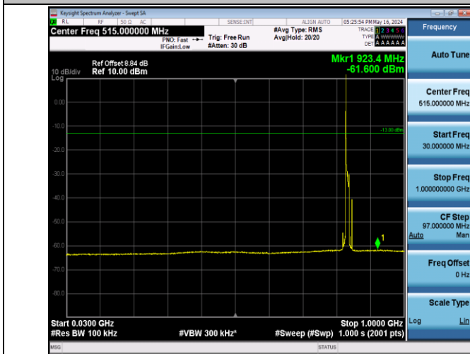
Band5_10MHz_16QAM_20525_1RB#0_30~1000_30~1000
