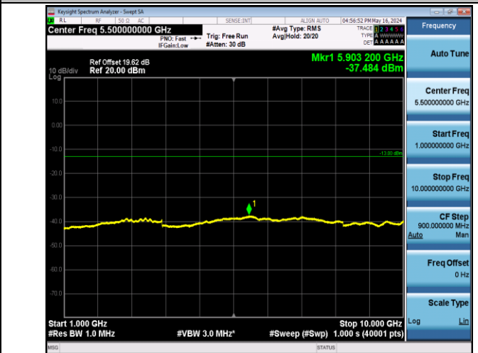
Band5_1.4MHz_QPSK_20643_1RB#0_1000~10000_1000~10000
