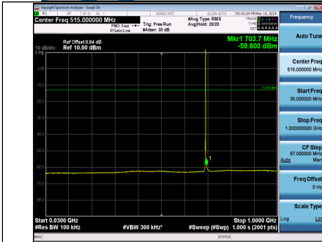
Band12_1.4MHz_QPSK_23017_1RB#0_30~1000_30~1000
