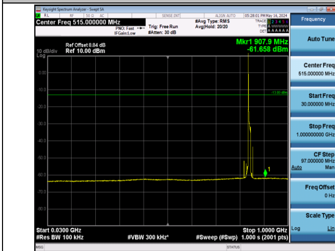
Band5_10MHz_16QAM_20600_1RB#0_30~1000_30~1000
