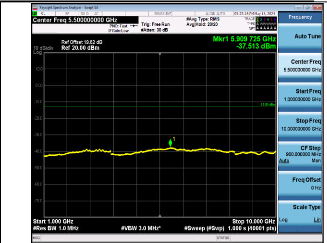
Band5_10MHz_QPSK_20450_1RB#0_1000~10000_1000~10000
