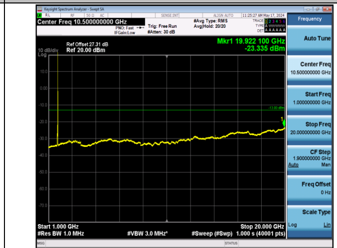
Band66_20MHz_QPSK_132322_1RB#0_1000-20000_1000-2000
