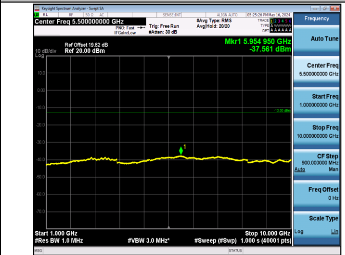
Band5_10MHz_QPSK_20525_1RB#0_1000~10000_1000~10000
