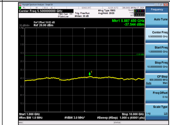
Band12_10MHz_16QAM_23095_1RB#0_1000-10000_1000-1000 00
