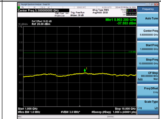
Band12_1.4MHz_QPSK_23095_1RB#0_1000~10000_1000~1000
