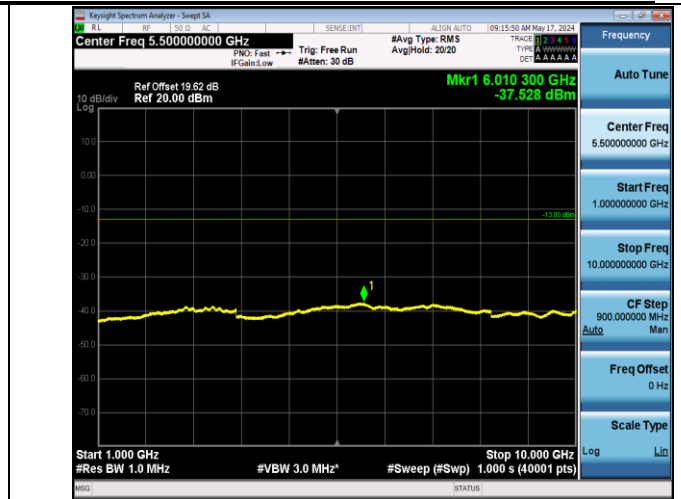
Band12_10MHz_QPSK_23060_1RB#0_1000~10000_1000~1000
