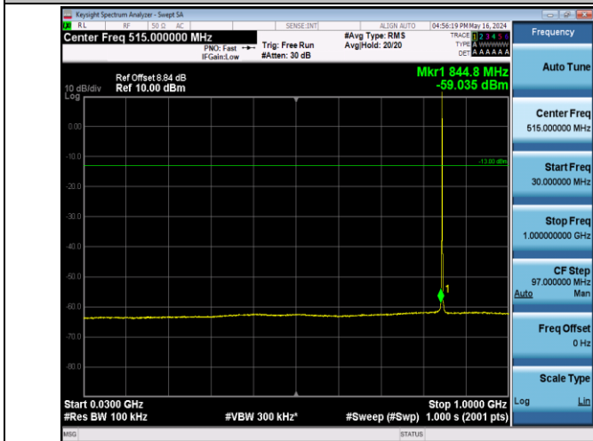
Band5_1.4MHz_QPSK_20643_1RB#0_30~1000_30~1000
