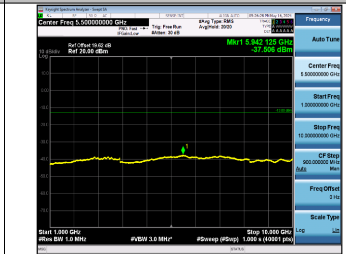
Band5_10MHz_16QAM_20525_1RB#0_1000~10000_1000~1000
