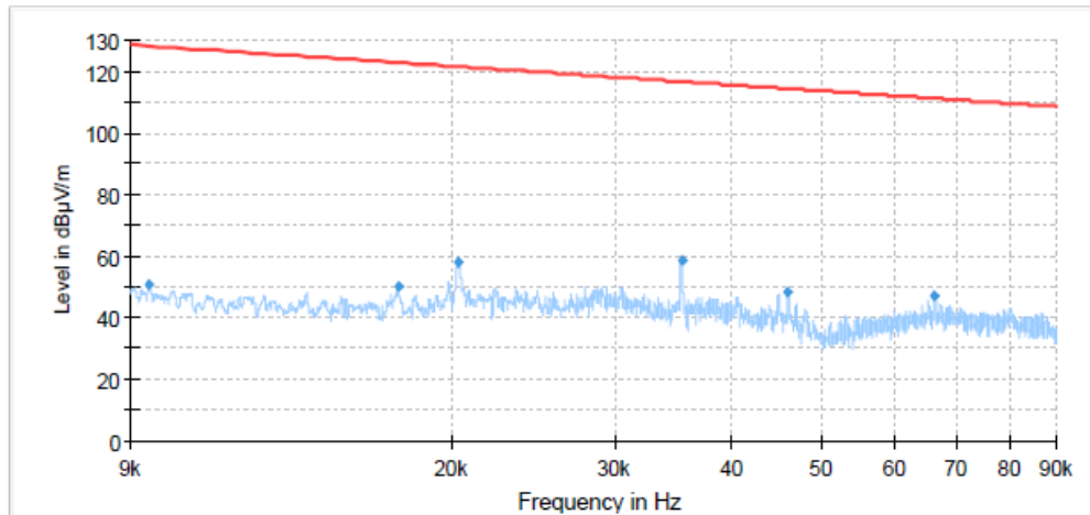
Radiates Emission from 9KHz to 90KHz
