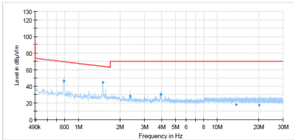
Radiates Emission from 490KHz to 30MHz
