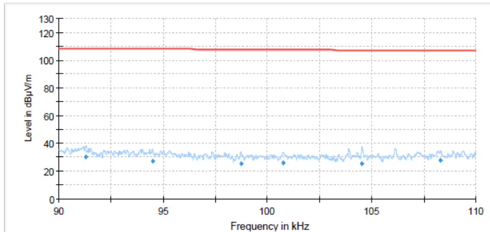
Radiates Emission from 90KHz to 110KHz
