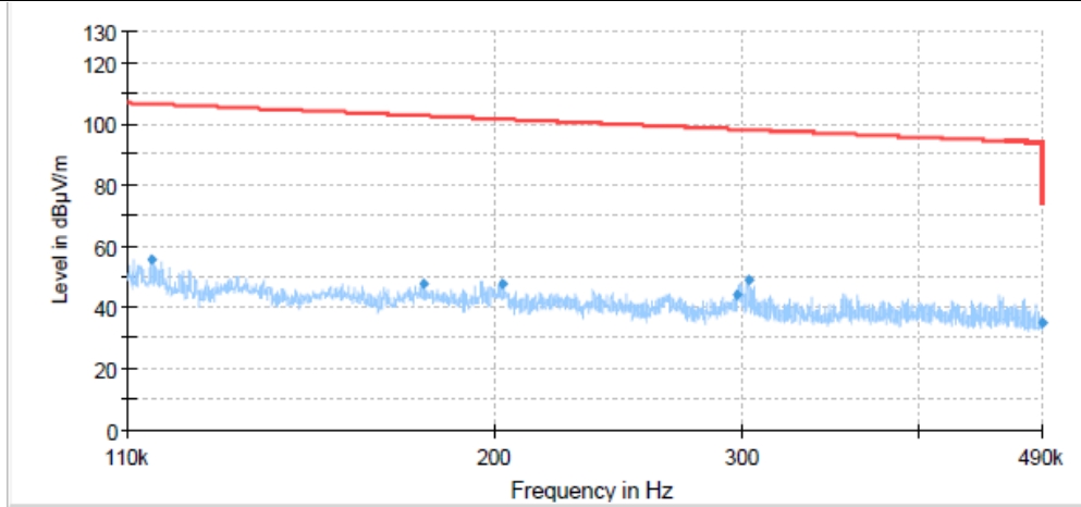
Radiates Emission from 110KHz to 490KHz
