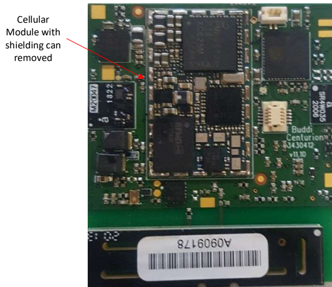
Figure 3: Smart Tag 4 v11.10 PCBA – top view with Module shielding can be removed
