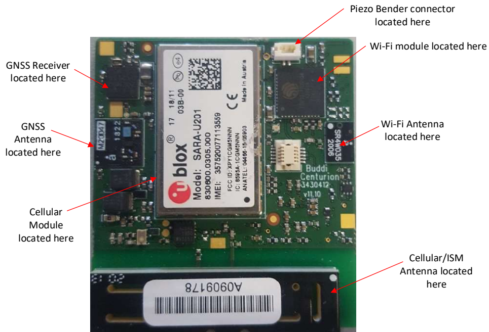
Figure 1: Smart Tag 4 v11.10 PCBA – top view
