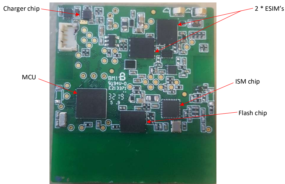
Figure 2: Smart Tag 4 v11.10 PCBA – bottom view
