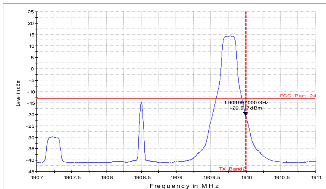
Fula2_028b_FCC_24_BE_High_Ch19185_BW_3MHz_AV
