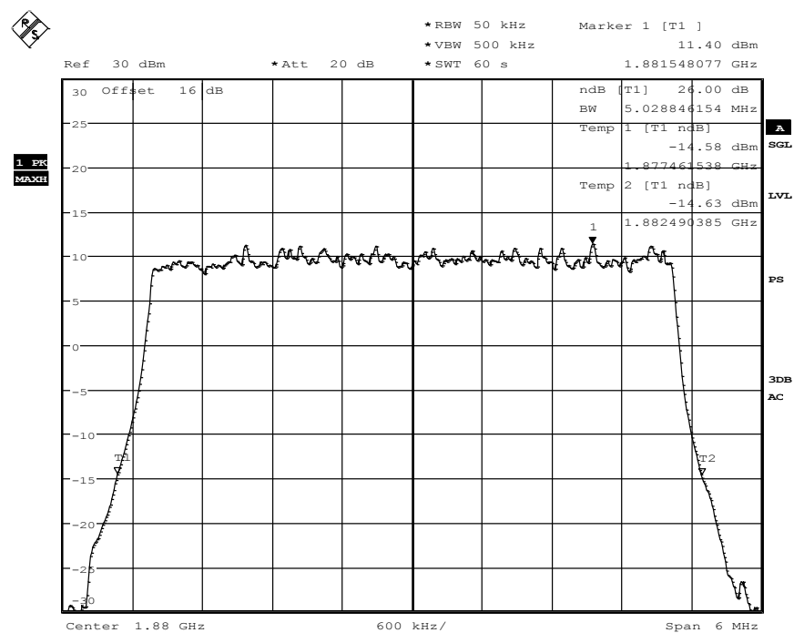
Diagram 34.207, QPSK-Modulation
