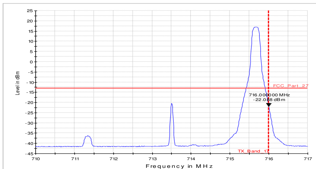
Fula2_003b_FCC_27_BE_high_Channel_23825_BW_5MHz_AV
