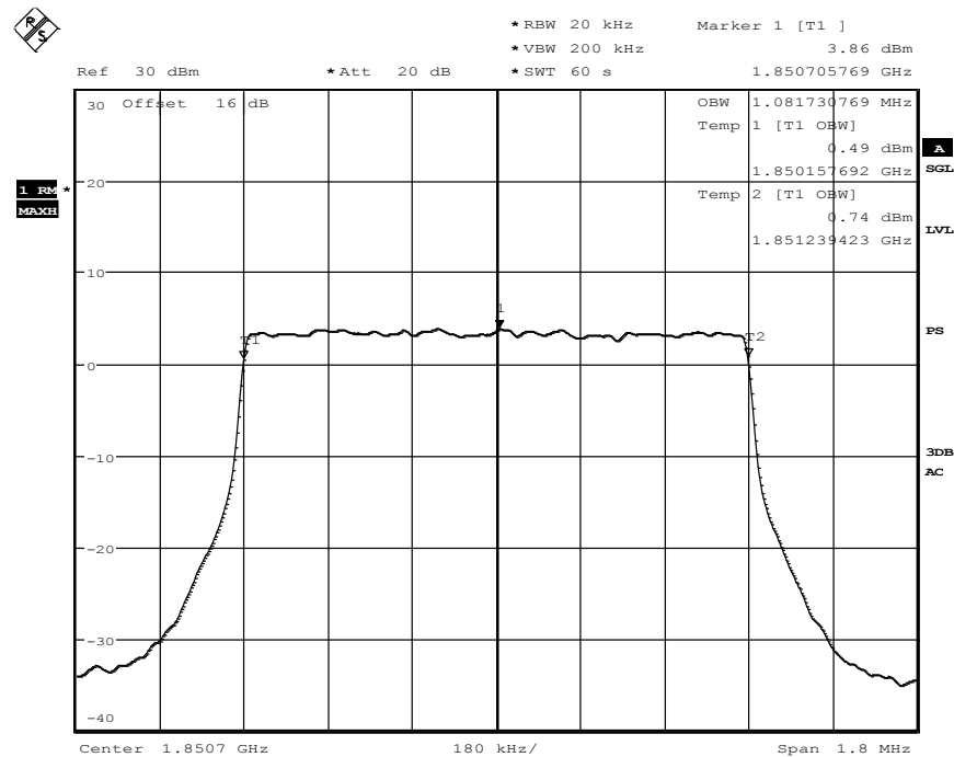
Diagram 35.200, QPSK-Modulation
