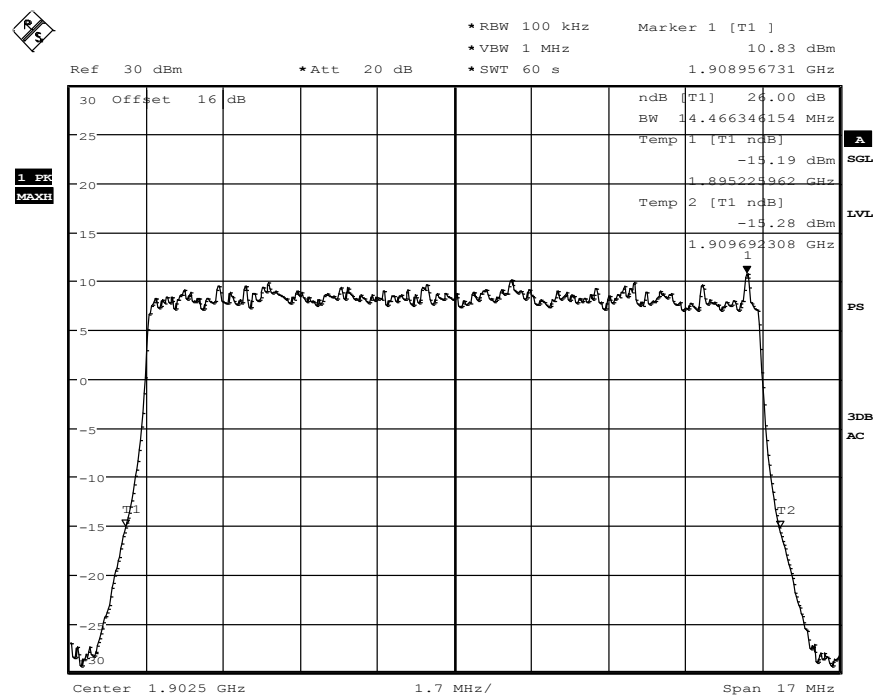
Diagram 34.212, QPSK-Modulation
