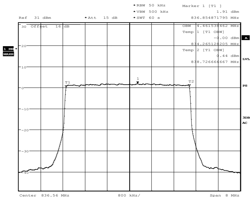
Diagram 35.509, QPSK-Modulation
