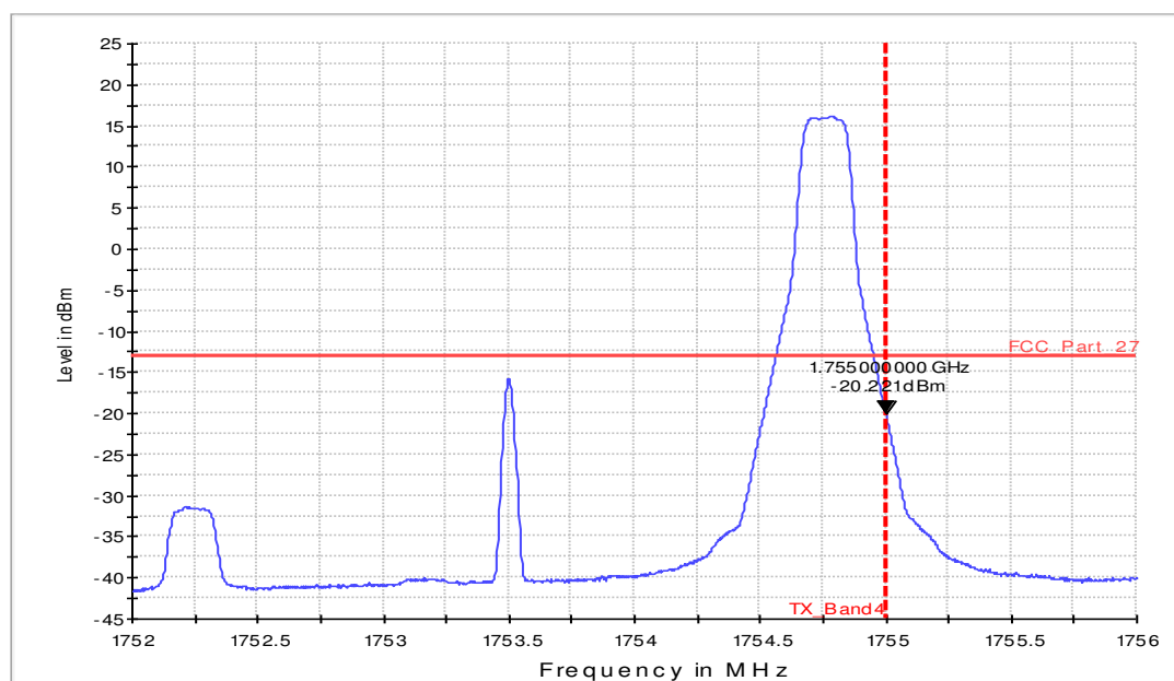
Fula2_016b_FCC_27_BE_High_Ch20385_BW_3MHz_AV
