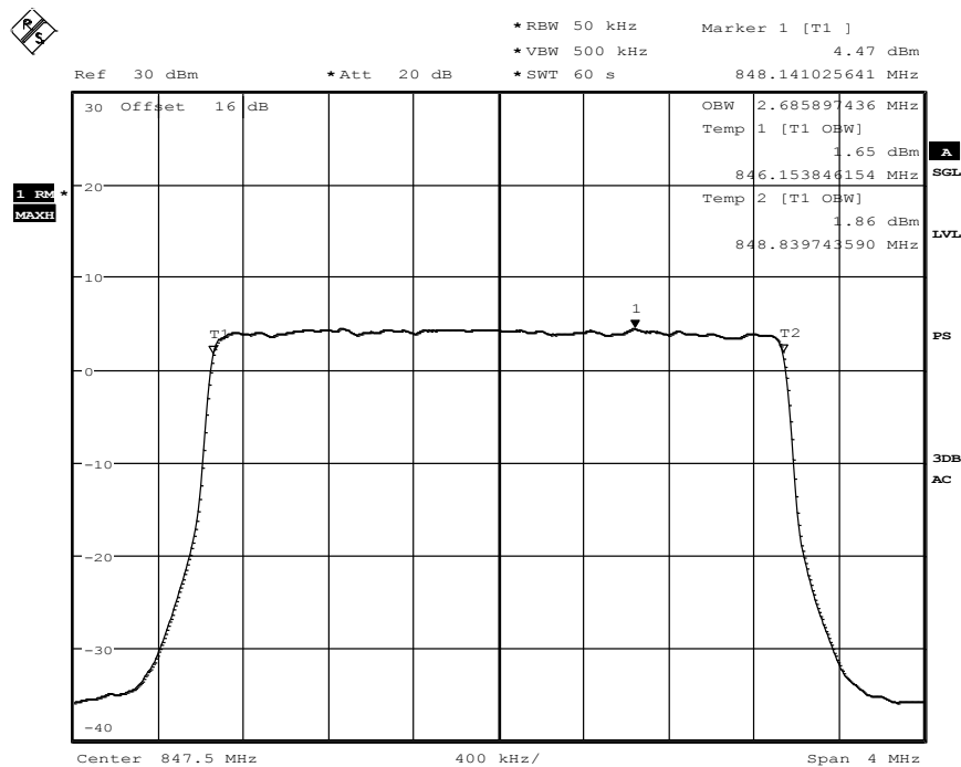
Diagram 35.504, QPSK-Modulation
