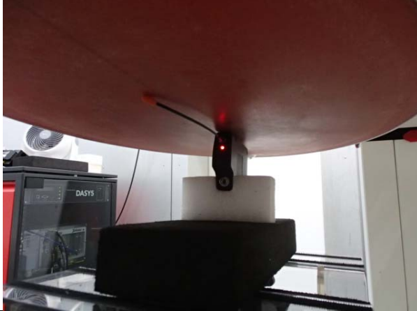
Photograph B14: Body, Right without microphone, 0 mm (Side view)
