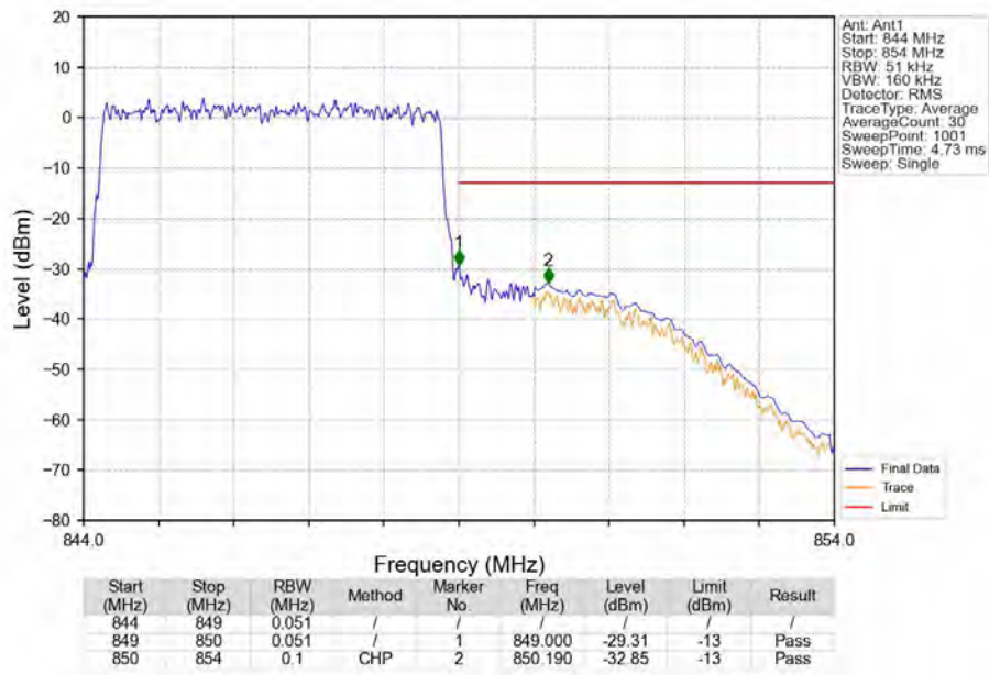
Band5_5MHz_16QAM_HCH_846.5MHz_RB_25_0_NTNV
