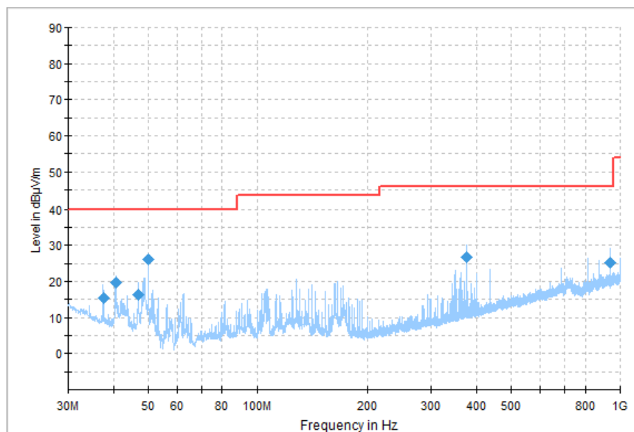
Fig.66 Radiated Spurious Emission (All Channels, 30MHz-1GHz)
