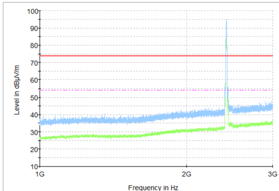
Fig.67 Radiated Spurious Emission (All Channels, 1GHz-3GHz)
