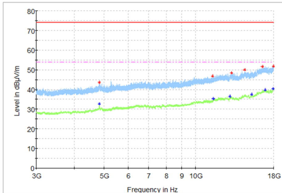
Fig.55 Radiated Spurious Emission (802.11n HT20, CH1, 3GHz-18GHz)
