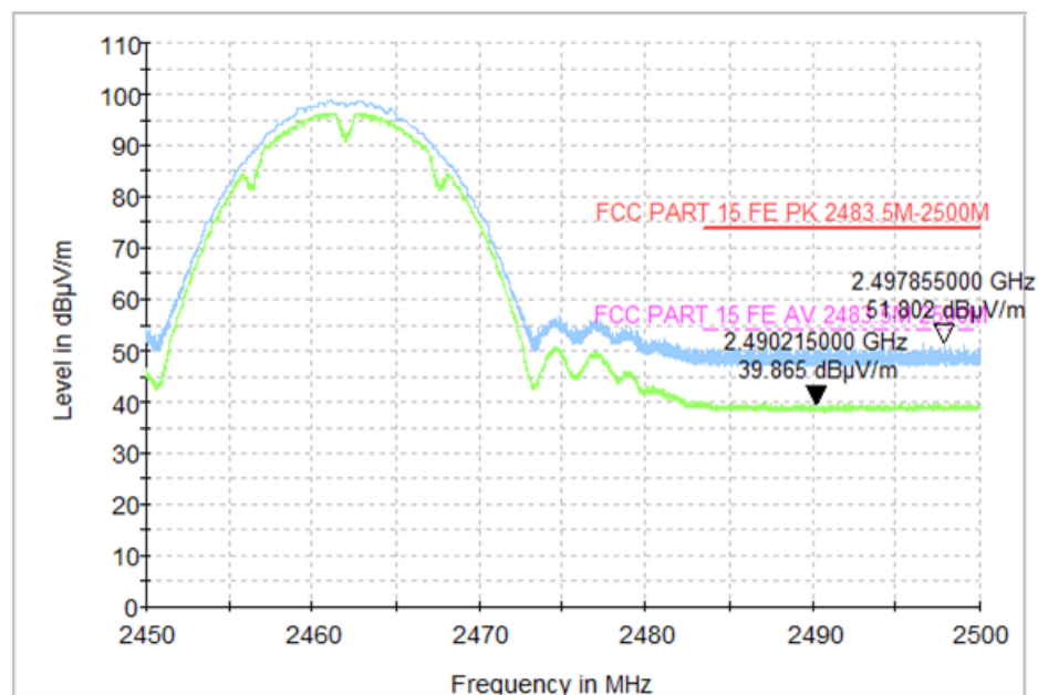
Fig.54 Radiated Restricted Band (802.11g, CH11, 2.45GHz~2.5GHz)
