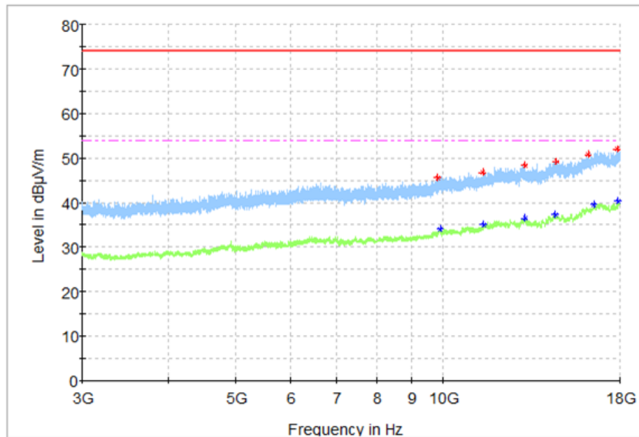
Fig.57 Radiated Spurious Emission (802.11n HT20, CH11, 3GHz-18GHz)
