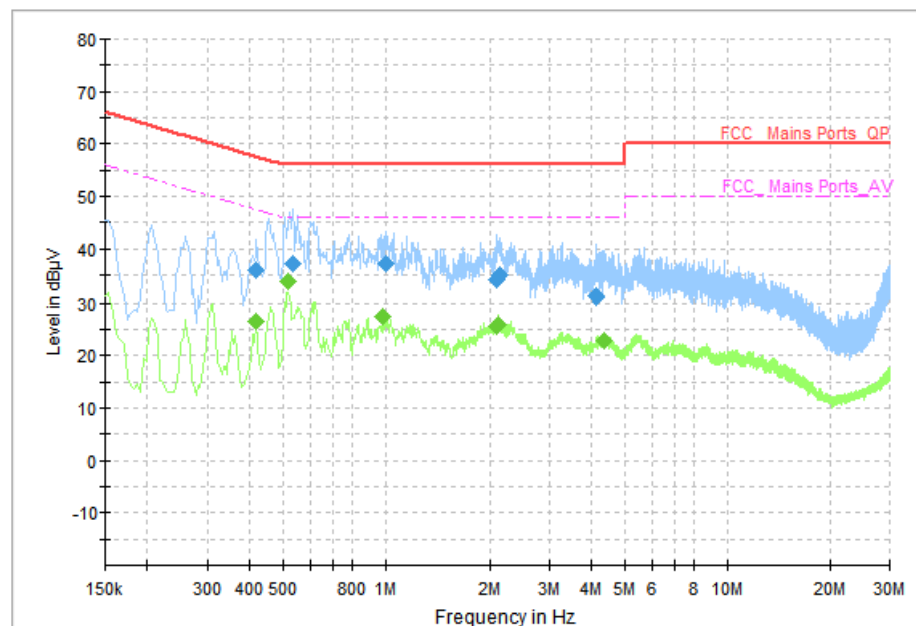
Fig.6.69 AC Power line Conducted Emission (Traffic, AE2, 120V)
