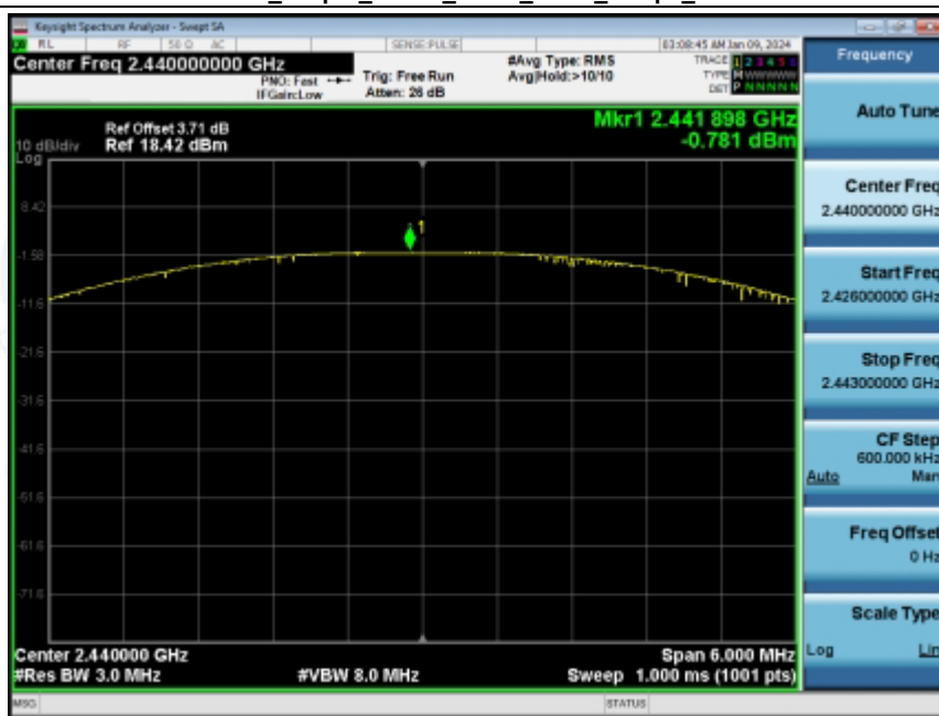
Peak_Output_Power_NVNT_ANT1_1Mbps_2440
