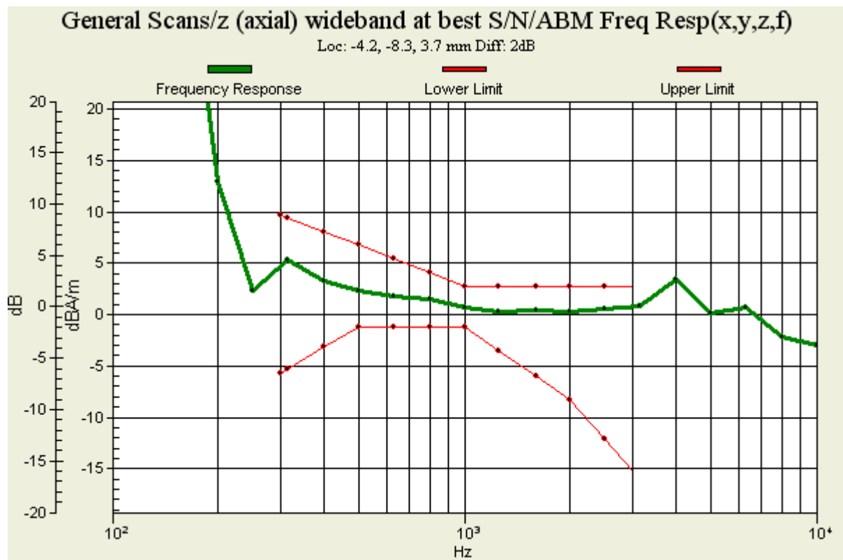
Figure 18 T-Coil WCDMA Band V Z Axial
