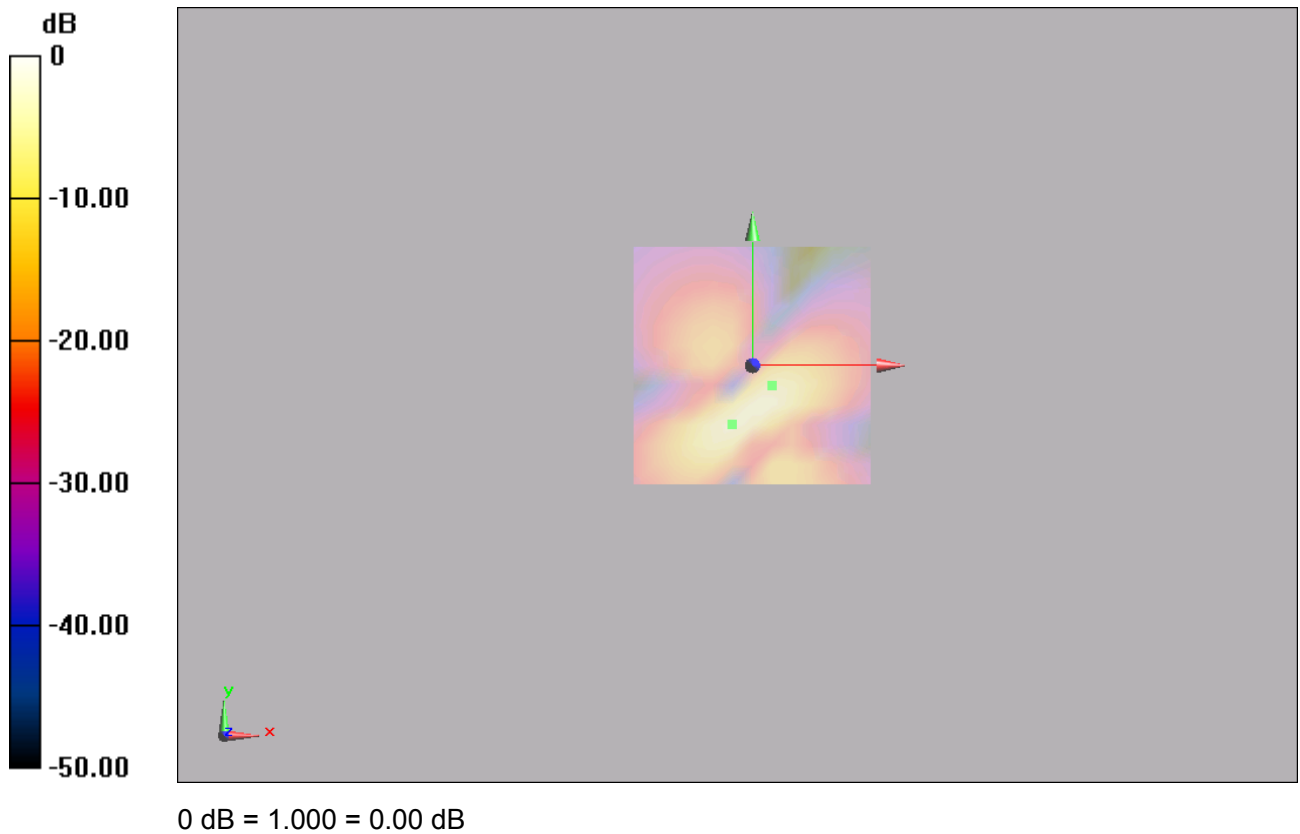
Figure 11 T-Coil GSM 850 Y transversal
