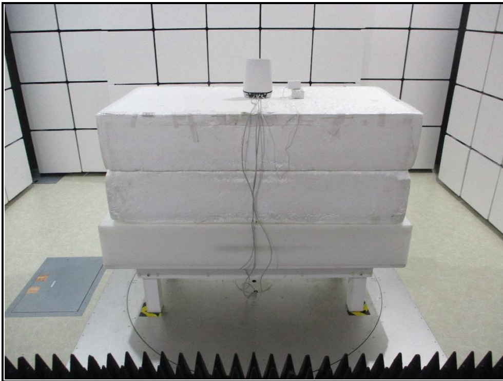
Internal Antenna
