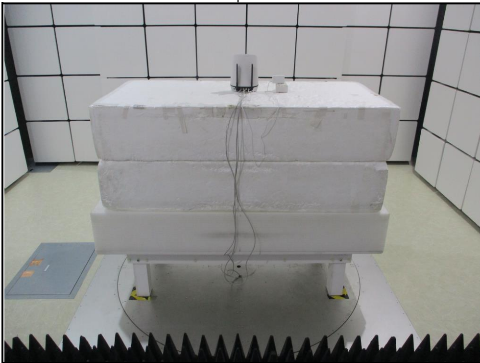
Dipole
