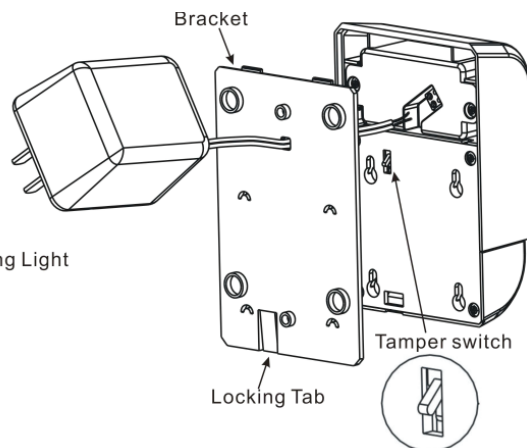
Bracket
