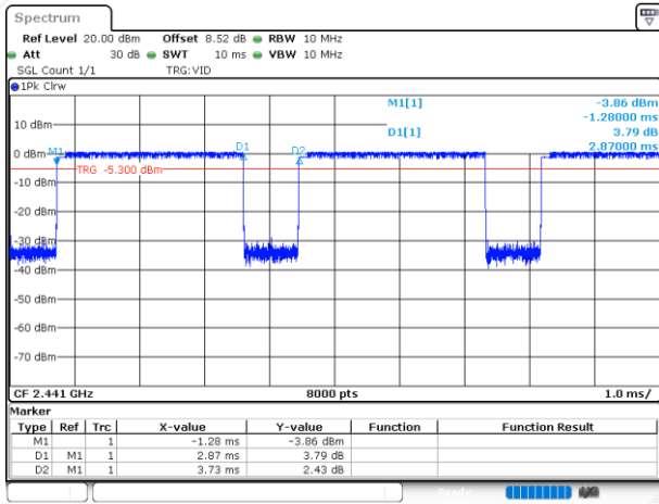
2DH5_2441MHz
