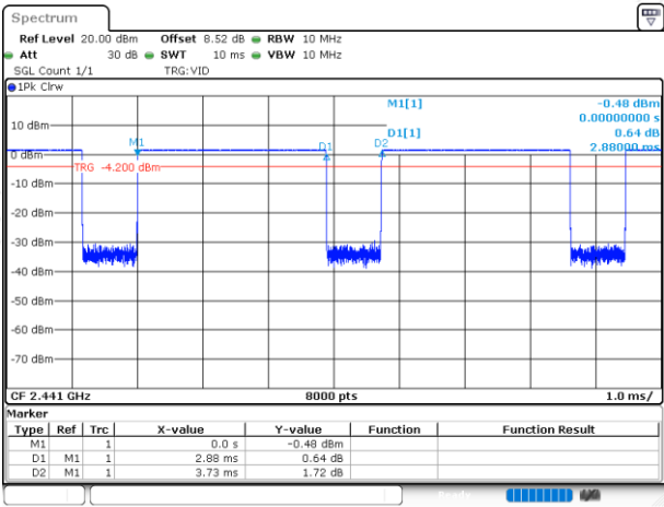
DH5_2441MHz
