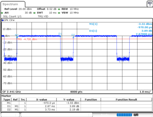
3DH5_2441MHz
