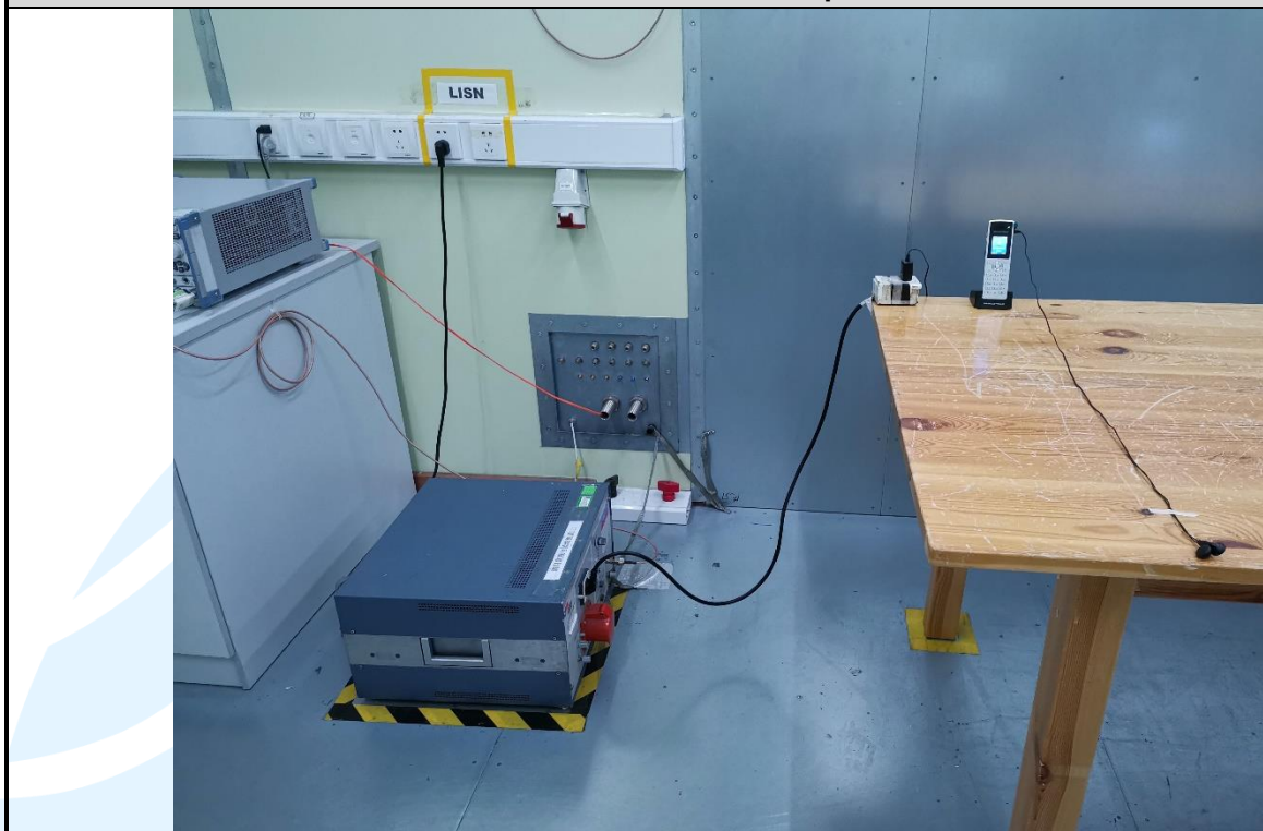
Conducted Emission Test Setup-3_Test Mode 6
