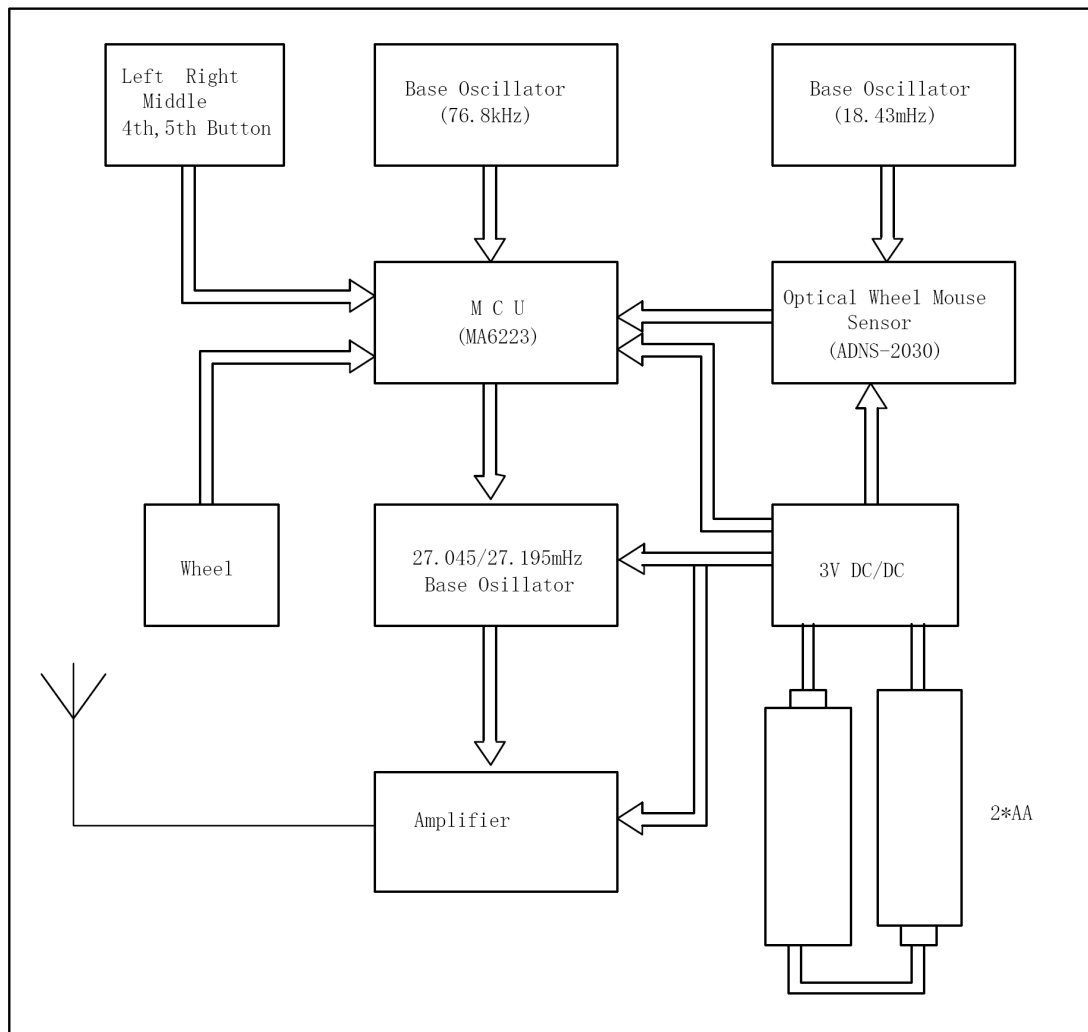
MOUSE PART
