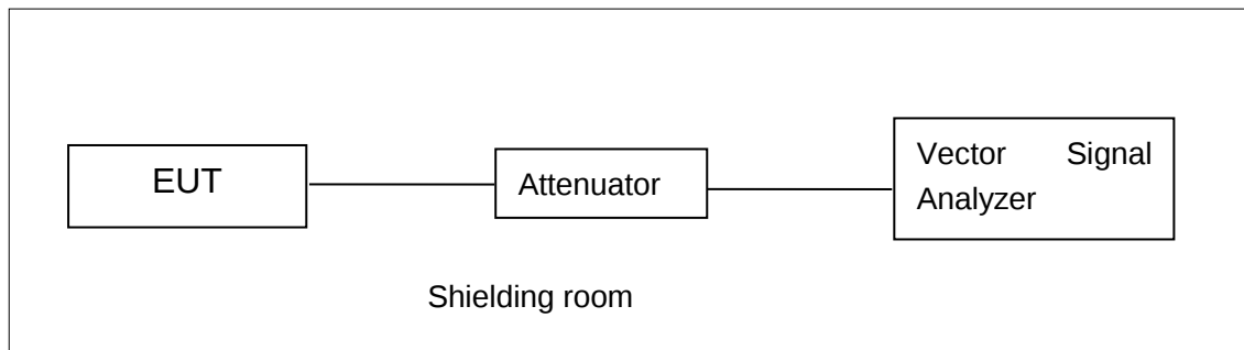
Fig.AB.1.1.1: Test Setup Diagram for Conducted Measurements
