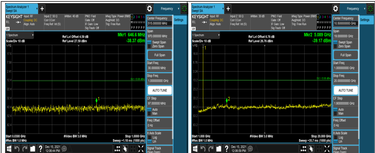
Band4-1.4MHz-QPSK-20175-1RB#0-Range1:30~1000MHz
