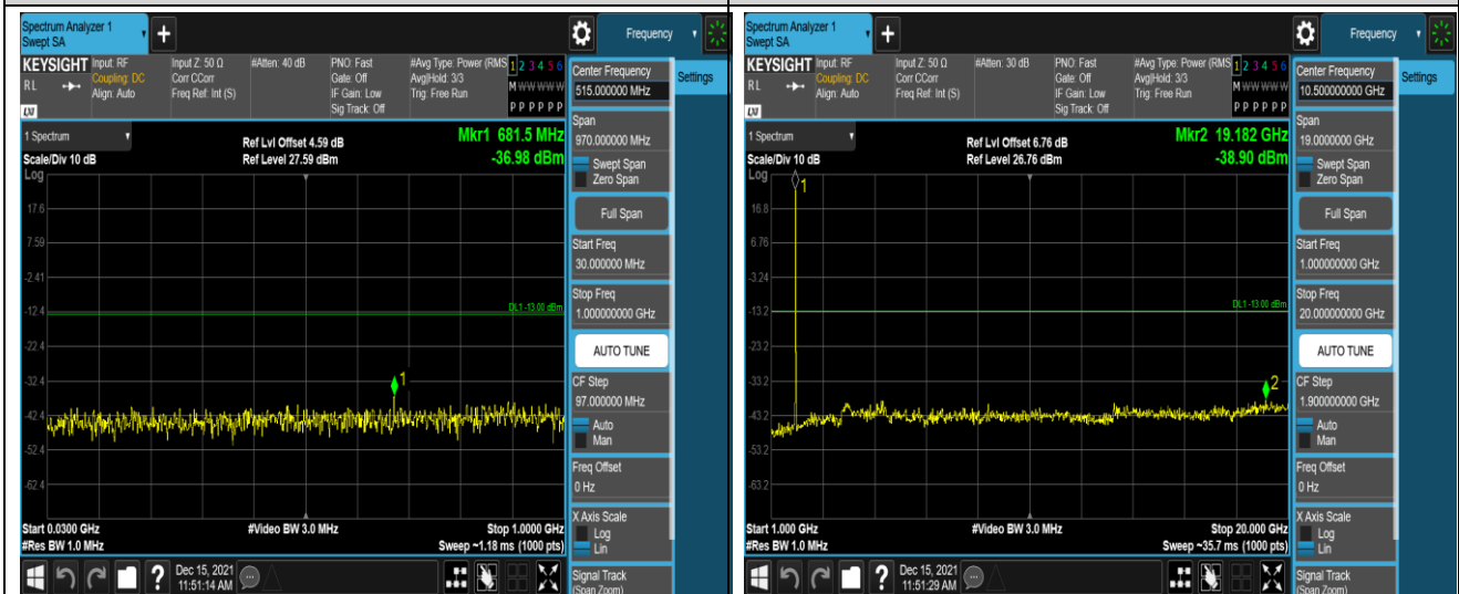
Band2-20MHz-16QAM-18700-1RB#0-Range1:30~1000MHz
