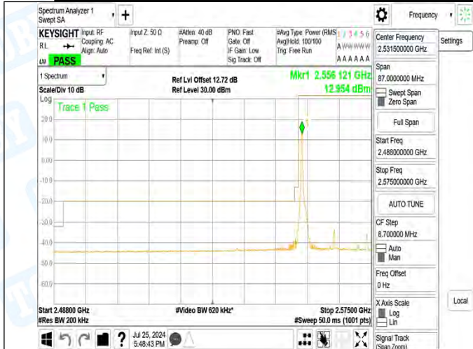
Band41_20MHz_16QAM_40340_100RB#0
