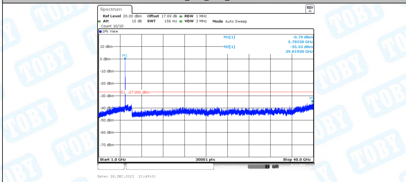
11AC40SISO_Ant1_5795_1000~40000
