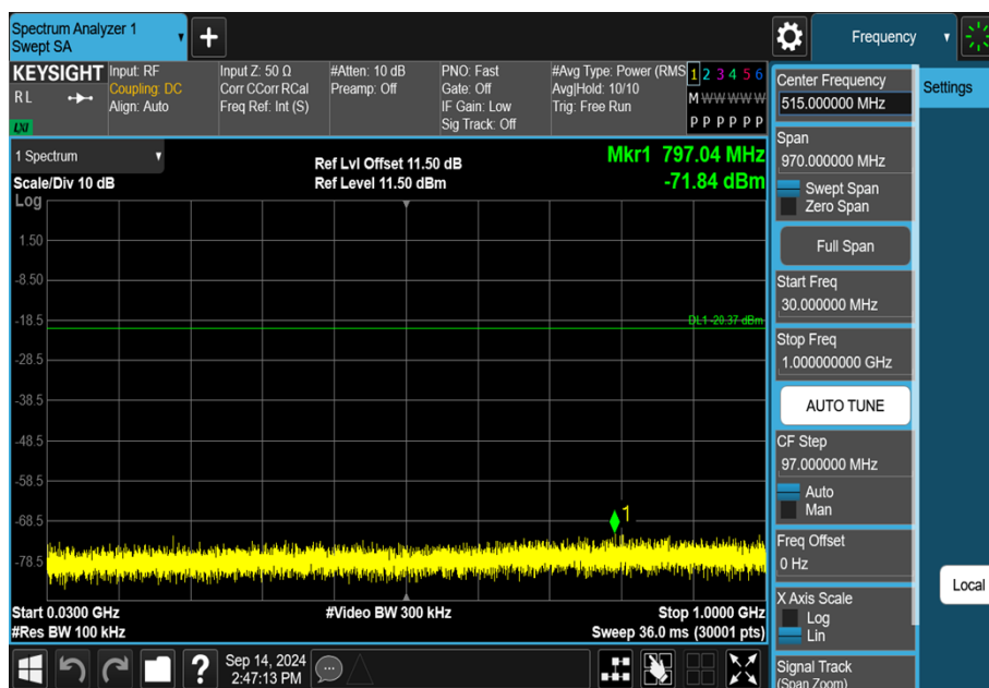
11N20SISO-Ant1-2412-30~1000-PASS
