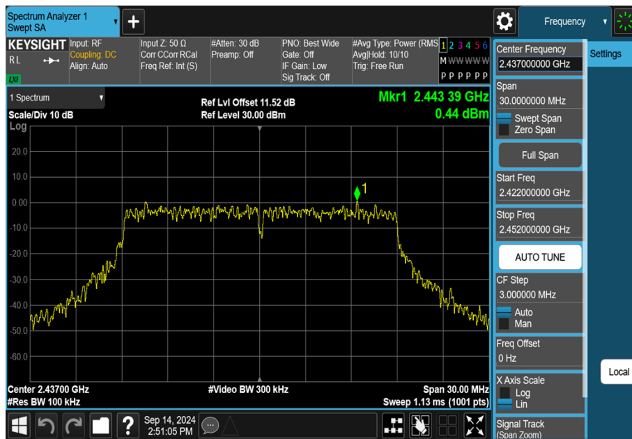
11N20SISO-Ant1-2437-0~Reference-PASS
