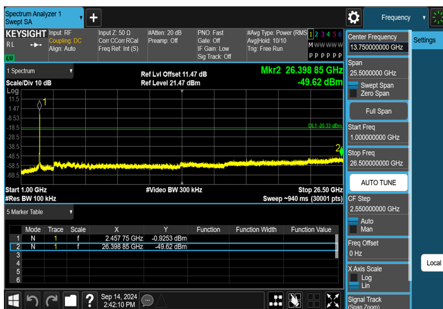
11G-Ant1-2462-1000~26500-PASS
