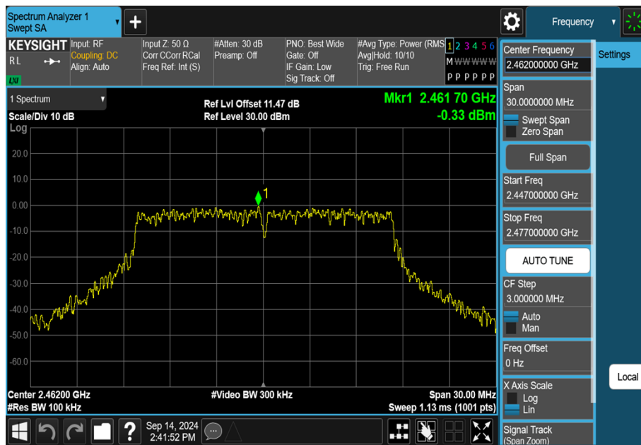
11G-Ant1-2462-0~Reference-PASS
