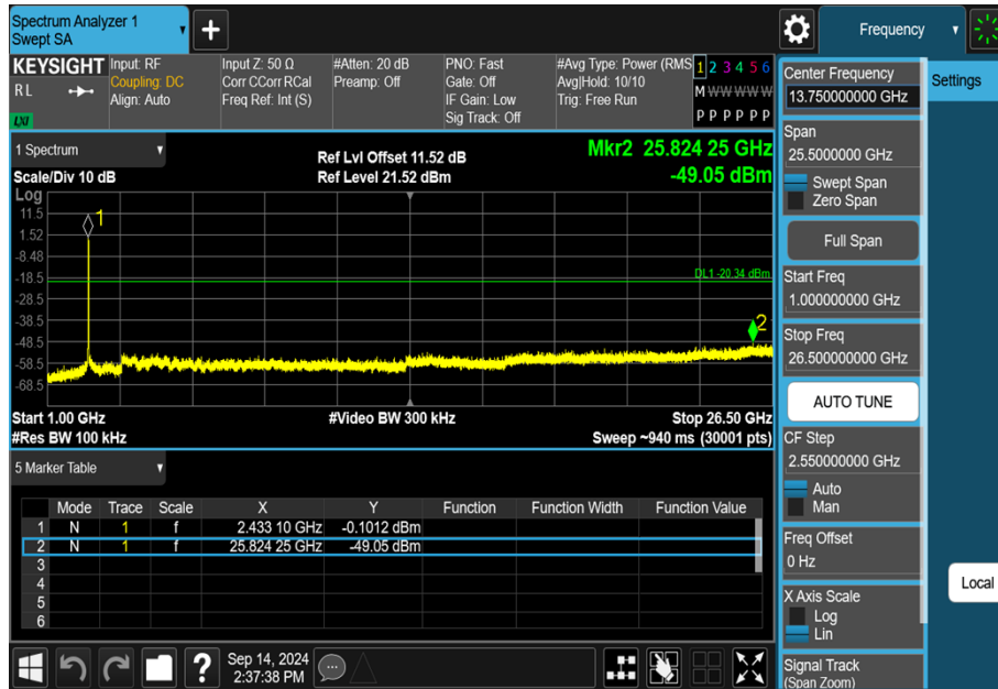
11G-Ant1-2437-1000~26500-PASS
