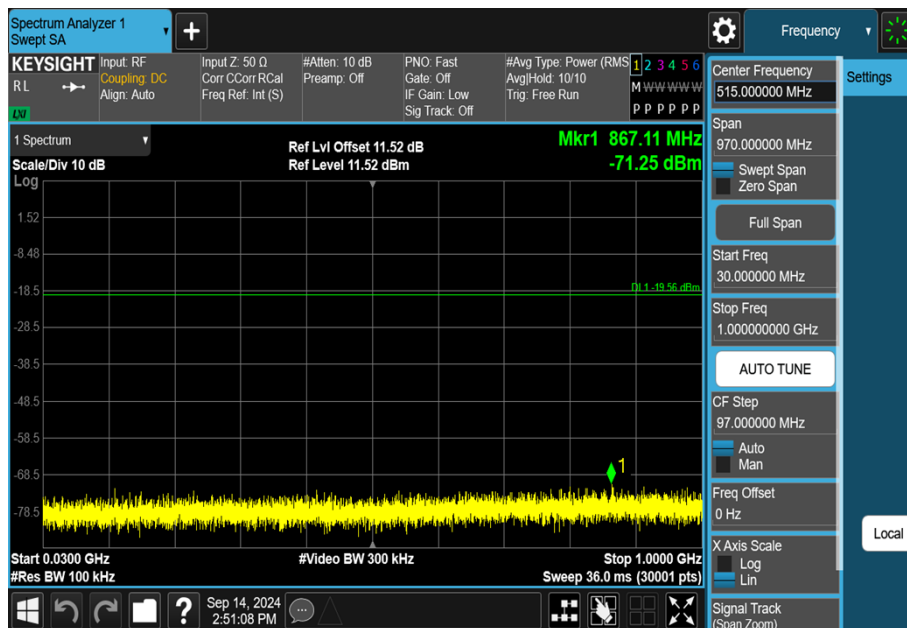
11N20SISO-Ant1-2437-30~1000-PASS
