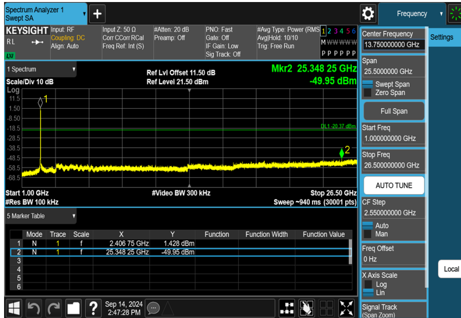
11N20SISO-Ant1-2412-1000~26500-PASS
