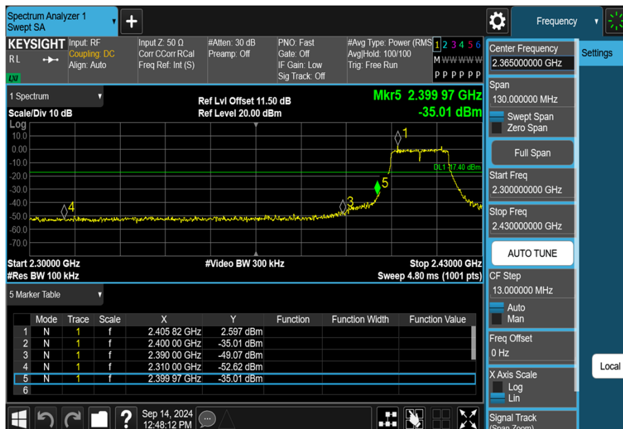
11G-Ant1-2412-PASS
