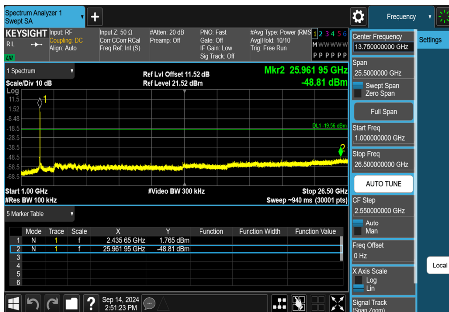
11N20SISO-Ant1-2437-1000~26500-PASS
