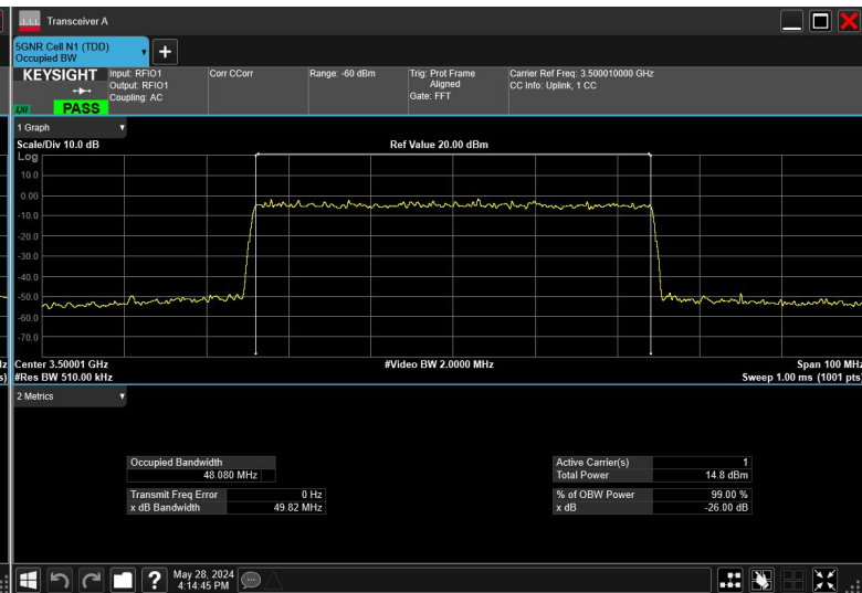
50MHz_15kHz_3500MHz_CP-OFDM256QAM_RB270@0
