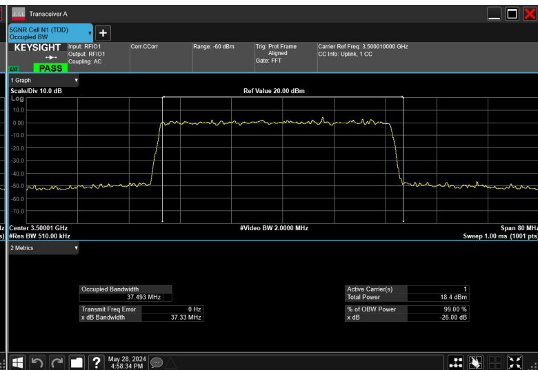
40MHz_30kHz_3500MHz_DFT-s-OFDM64QAM_RB100@0
