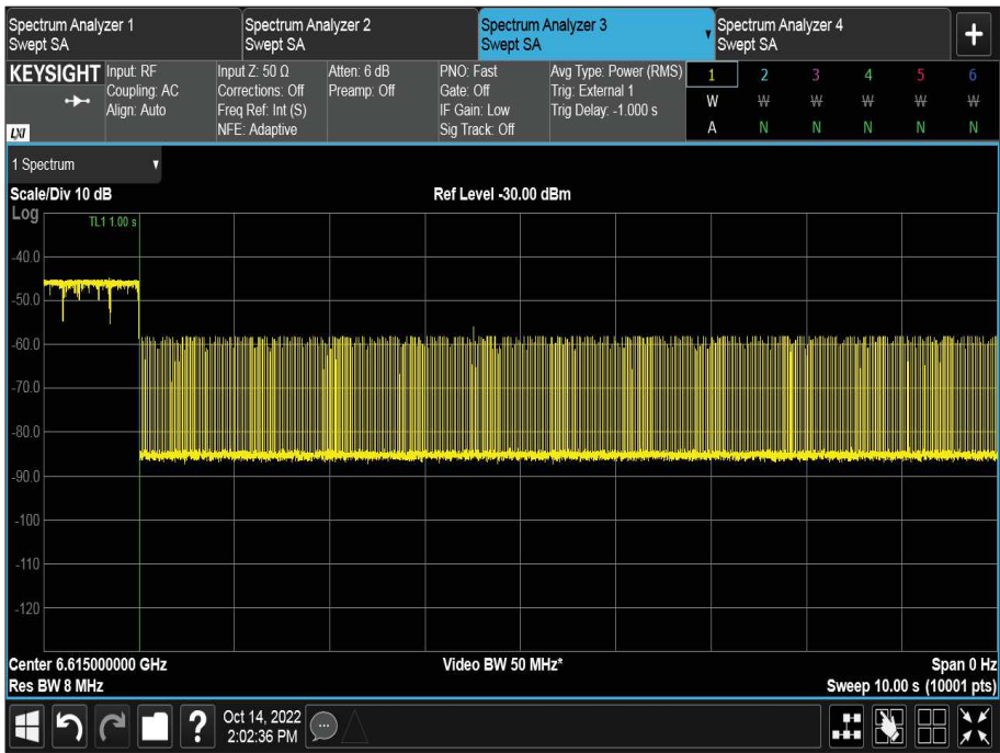
Figure 145 - - U-NII-7, Minimum Bandwidth (AWGN Low)
