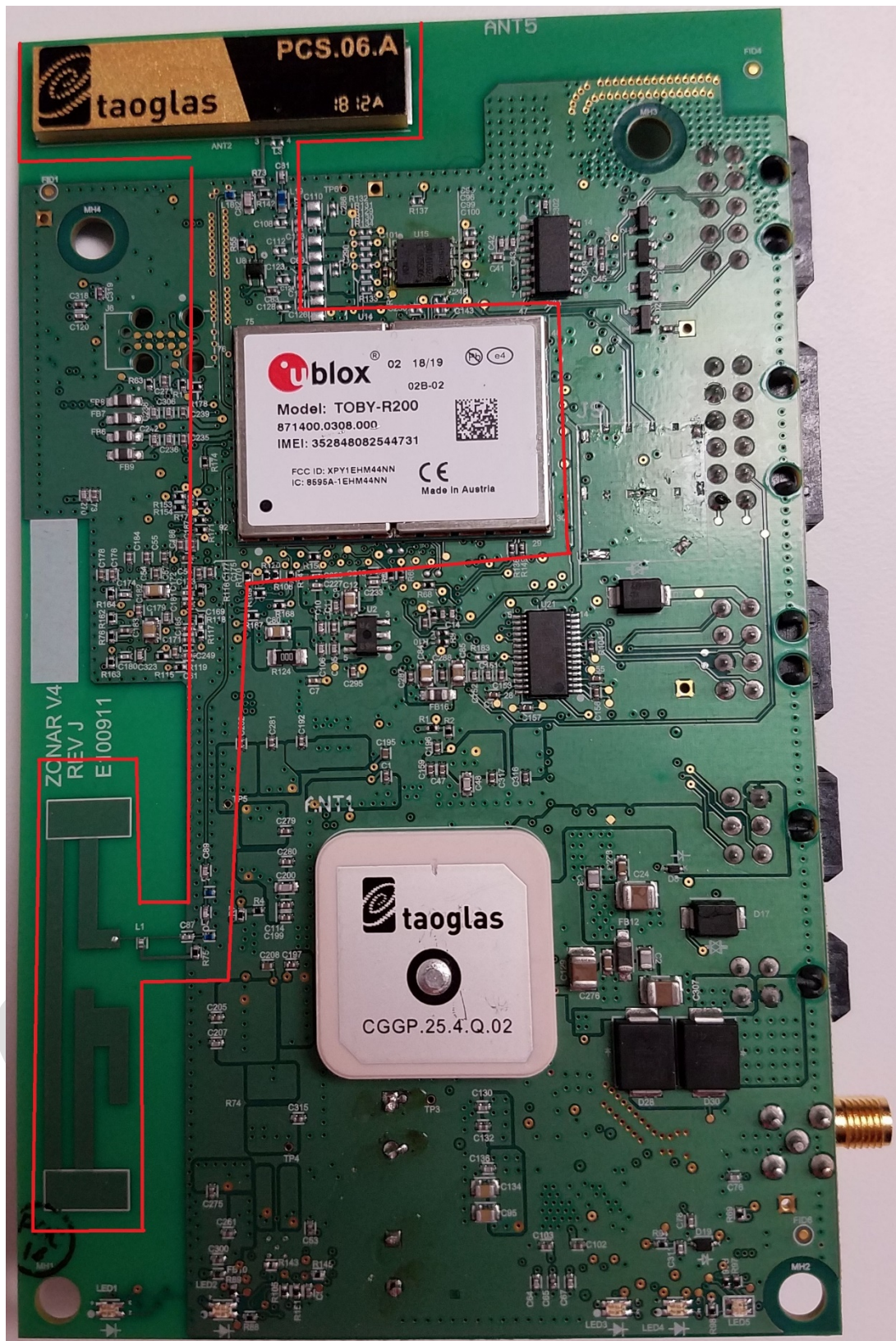
Figure 3 Cellular Radio Sub-Circuit
