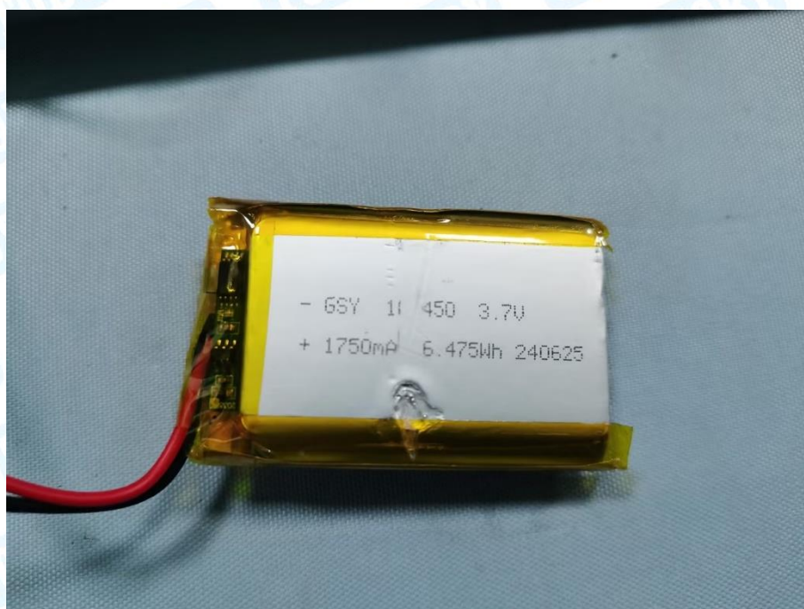
Photo 8 Battery Appearance
