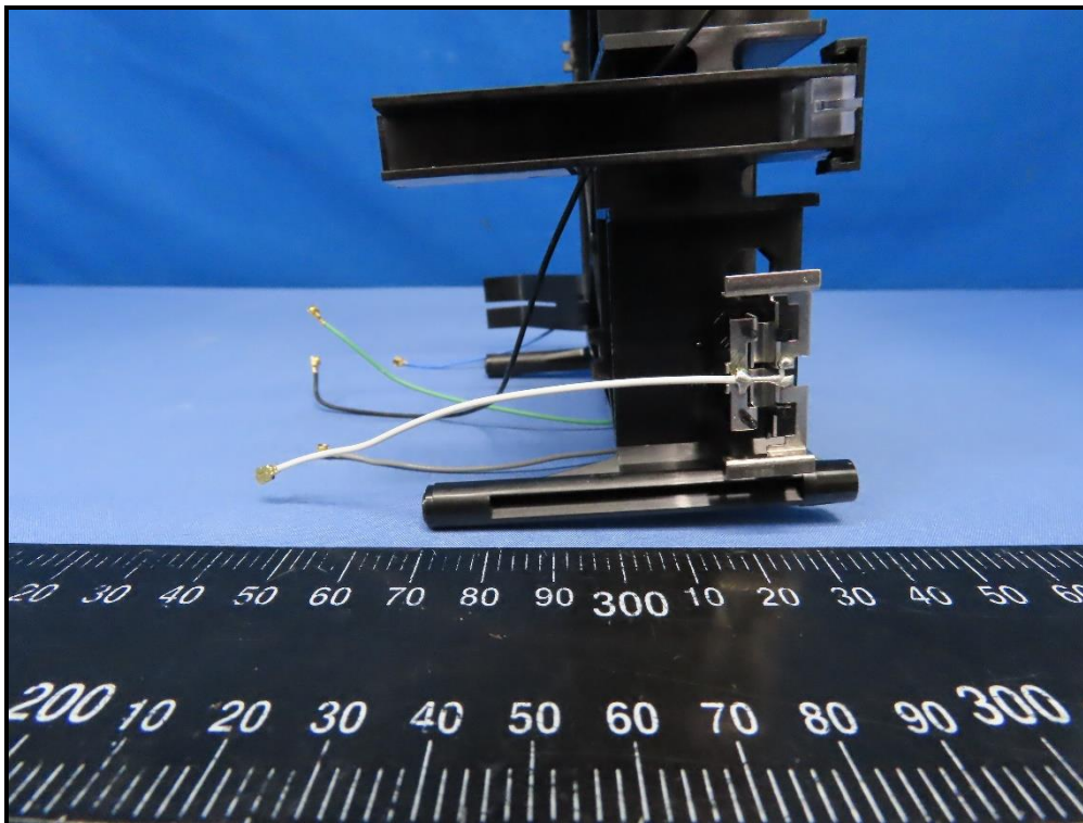
Antenna NO.: DB1
