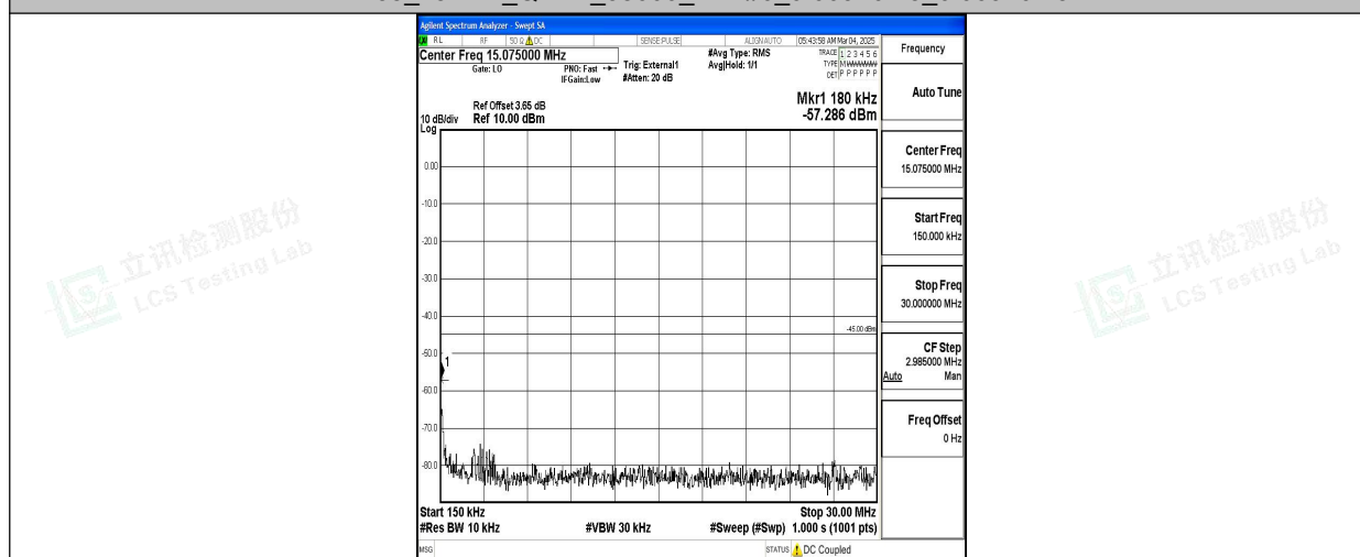
Band38_15MHz_QPSK_38000_1RB#0_0.15~30_0.15~30
