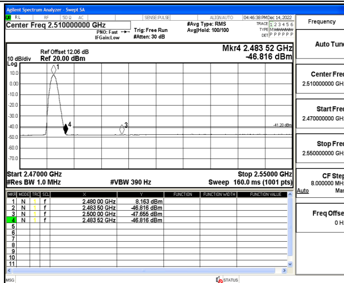
DH5_Ant3_High_2480_Peak
