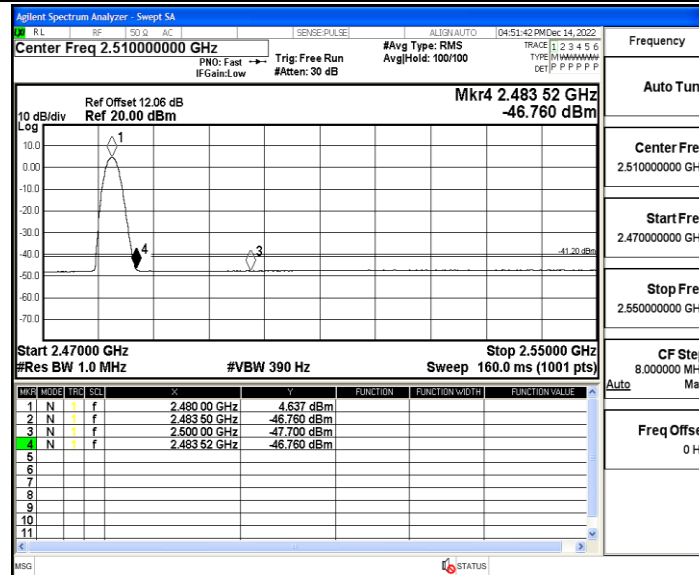
2DH5_Ant3_High_2480_Peak
