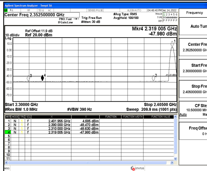
2DH5_Ant3_Low_2402_Peak
