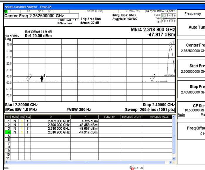
3DH5_Ant3_Low_2402_Peak
