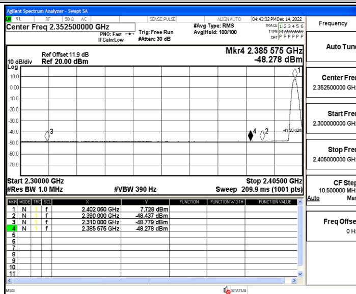
DH5_Ant3_Low_2402_Peak
