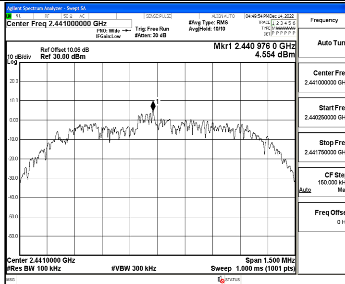
2DH5_Ant3_2441_30~1000
