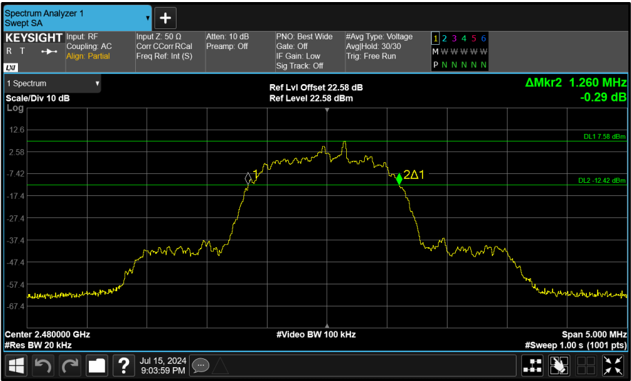
Figure 96 - Core 0 (A) 2480 MHz (CH78) 20 dB Bandwidth
