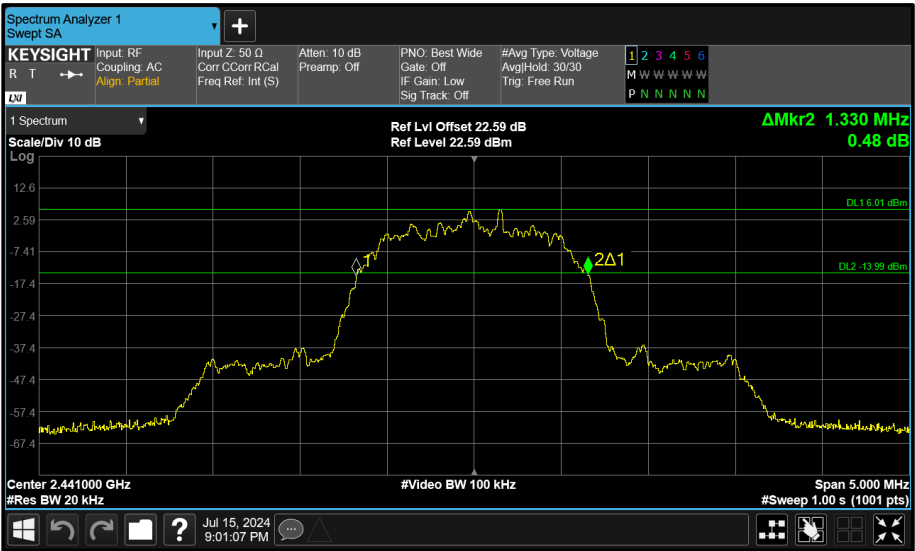
Figure 89 - Core 0 (A) 2441 MHz (CH39) 20 dB Bandwidth
