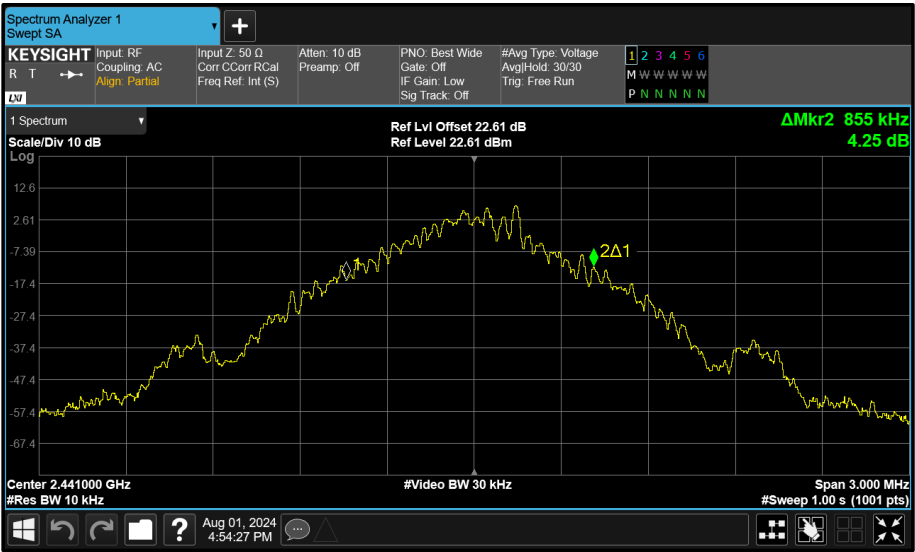
Figure 86 - Core 2 (C) 2441 MHz (CH39) 99% Bandwidth
