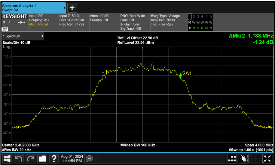
Figure 91 - Core 0 (A) 2402 MHz (CH0) 99% Bandwidth
