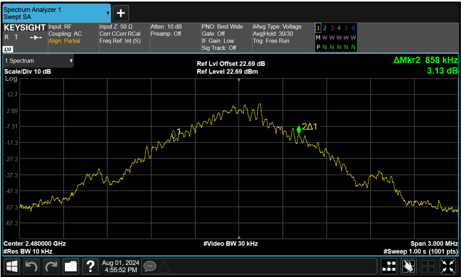
Figure 87 - Core 2 (C) 2480 MHz (CH78) 99% Bandwidth
