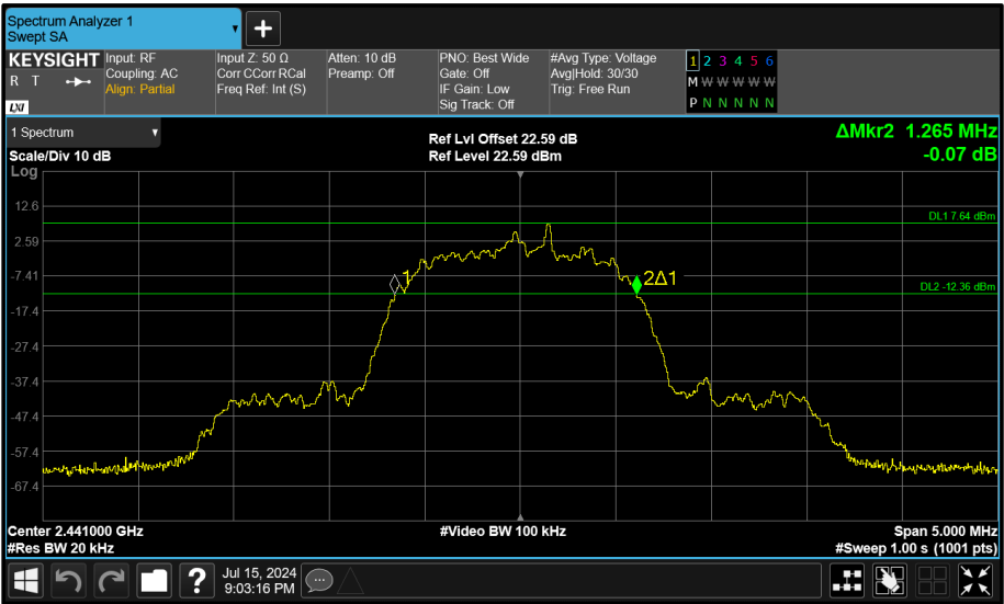
Figure 95 - Core 0 (A) 2441 MHz (CH39) 20 dB Bandwidth
