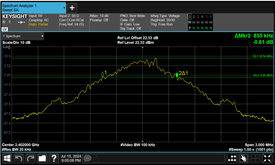
Figure 82 - Core 2 (C) 2402 MHz (CH0) 20 dB Bandwidth
