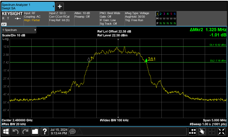
Figure 114 - Core 0 (A) 2480 MHz (CH78) 20 dB Bandwidth
