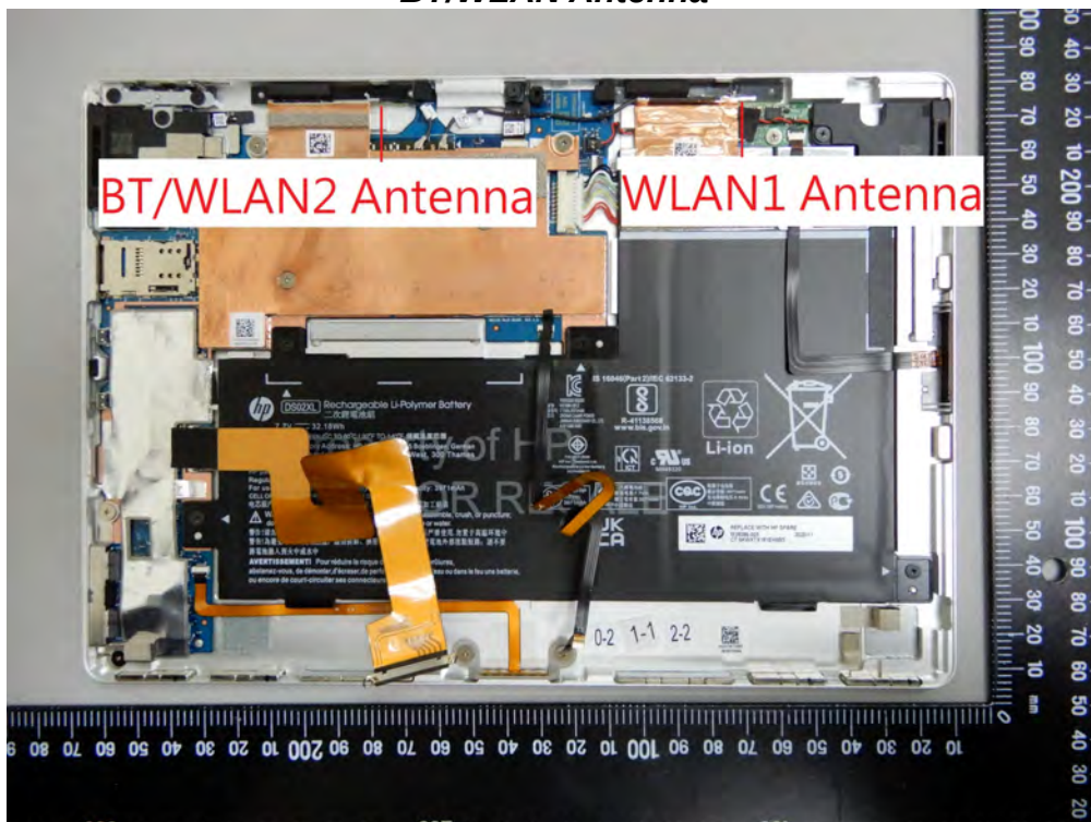
BT/WLAN Antenna
