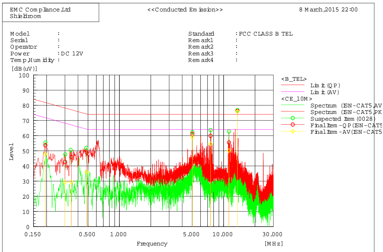
Figure4. plot of Conducted Emission
