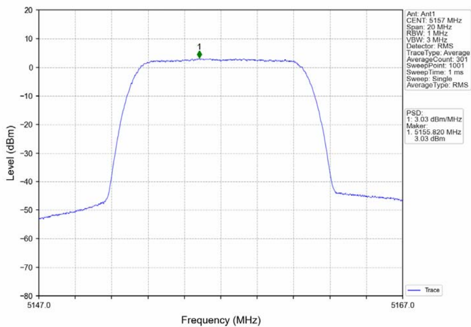
16QAM 10MHz_LCH_5157MHz_Ant1_NTNV
