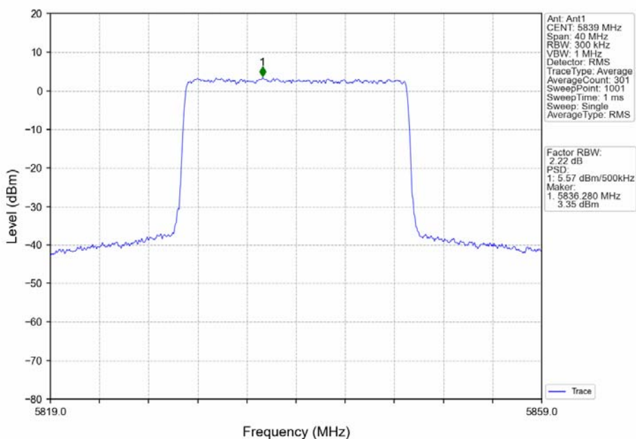
16QAM 20MHz_HCH_5839MHz_Ant1_NTNV
